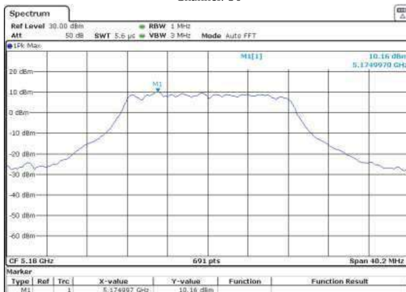
802.11a Channel: 36
