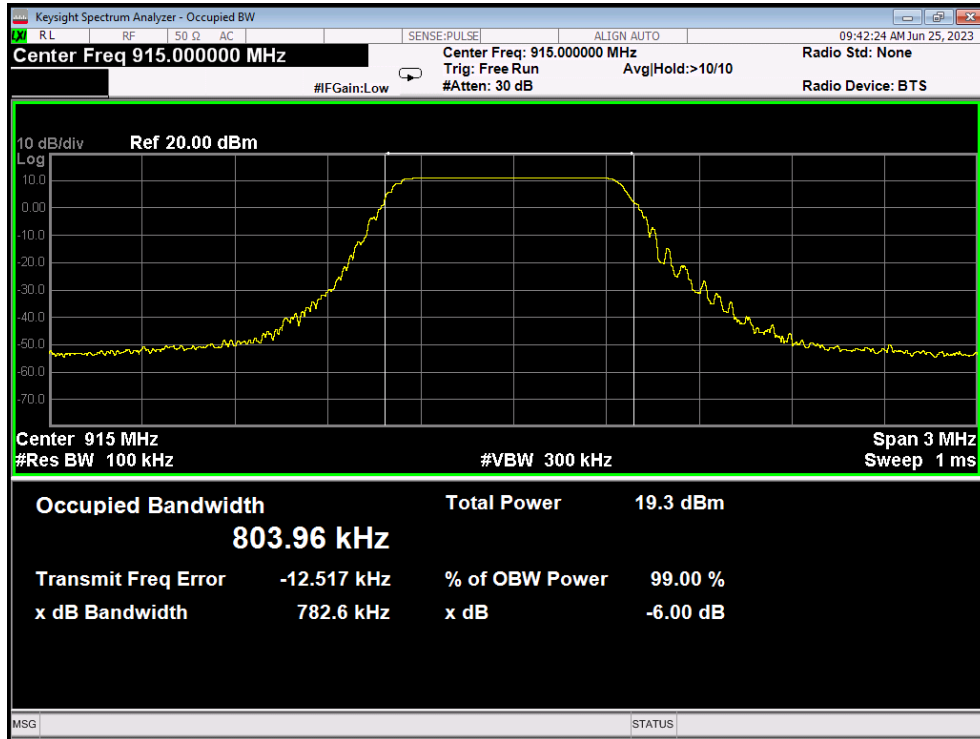
6dB Bandwidth plot on channel 0
