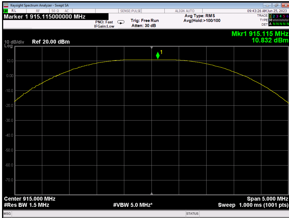
Peak output Power plot on channel 0
