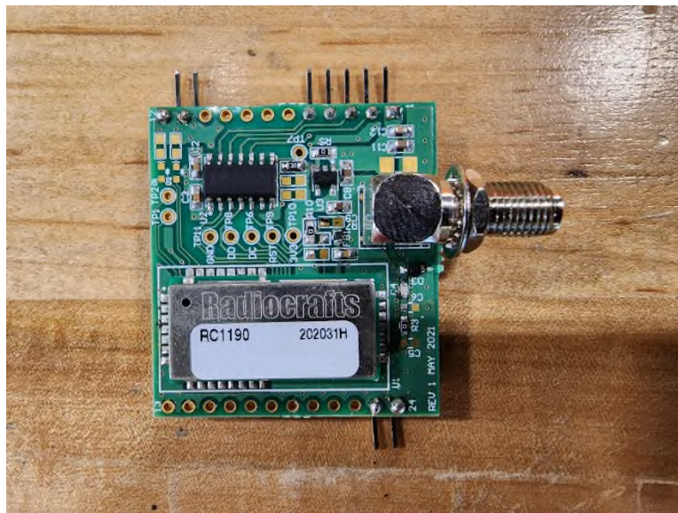
Figure 1 – Front without Antenna
