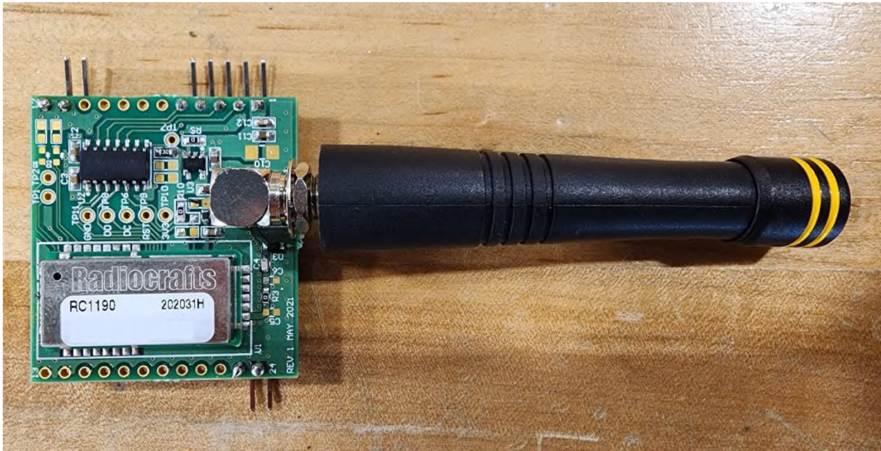
Figure 3 – Front with Antenna
