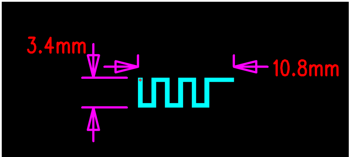
Picture of antenna
