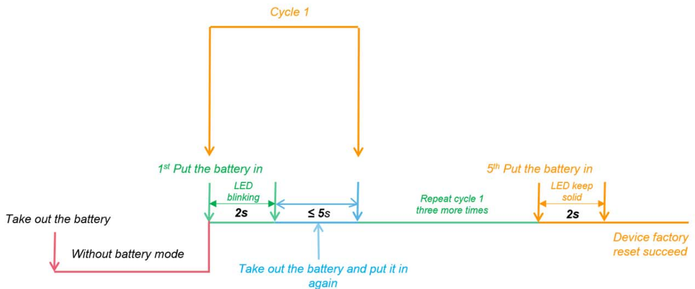
Figure 3: Hardware reset flowchart of M4 Pro Asset Tag
