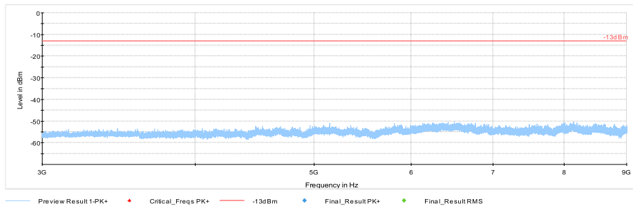
Plot #30 Radiated Emissions: 3-9 GHz
