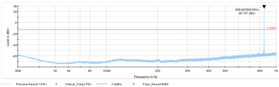
Plot #8 Radiated Emissions: 30 MHz – 1GHz
