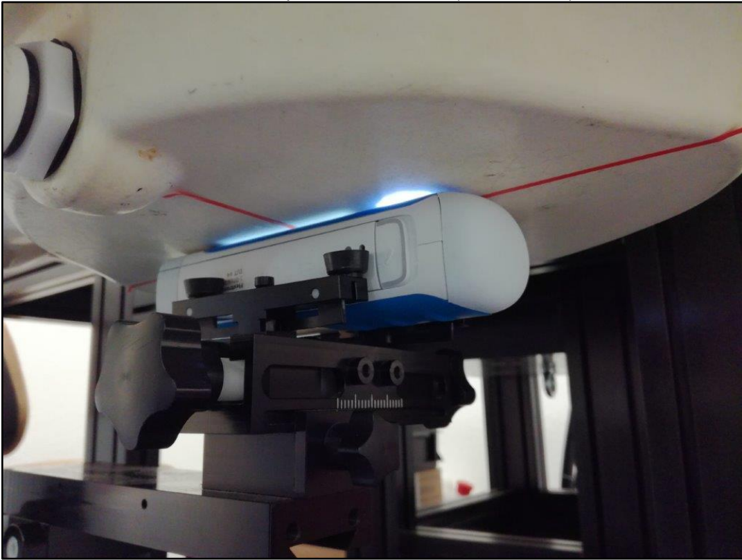
Photo 8: Test position - Rear side (0cm distance)
