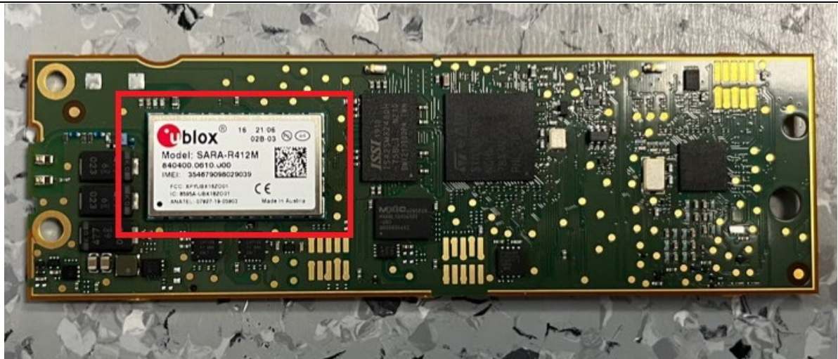
Internal pictures – Main PCBA with RF module
