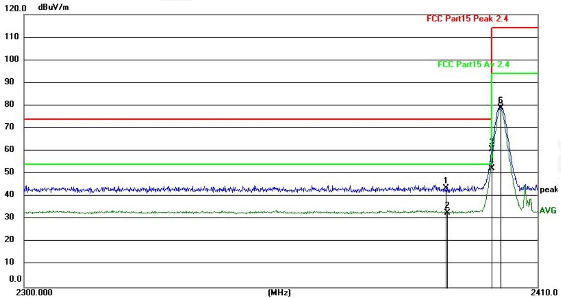
2402MHz Horizontal
