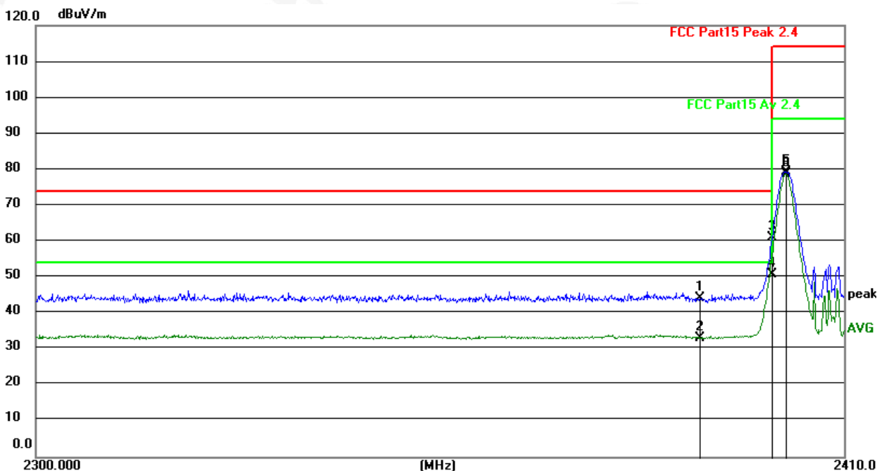
2402MHz Horizontal
