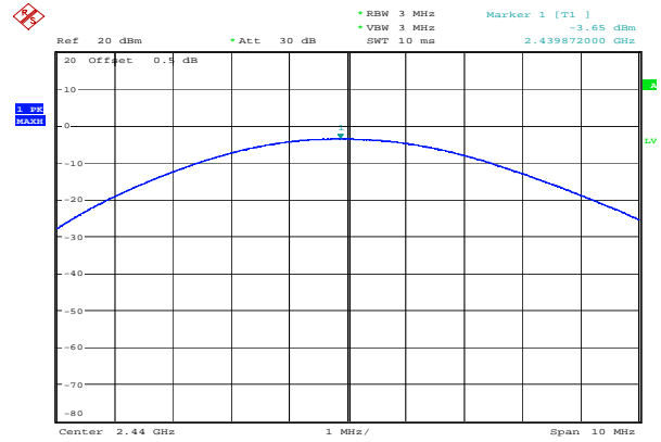
Middle -3.65 dBm
