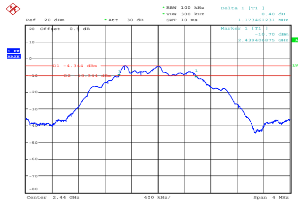
Middle 1.173 MHz
