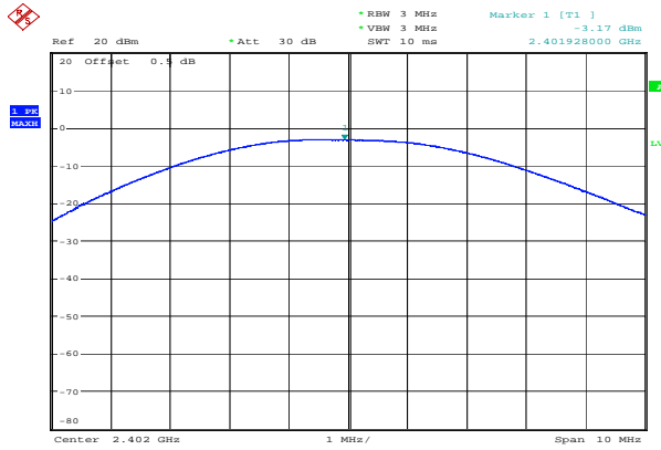
Low -3.17 dBm
