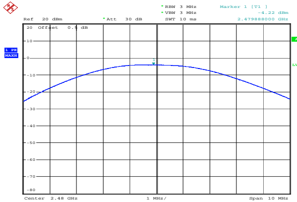
High -4.22 dBm
