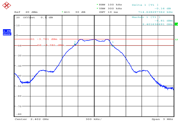
Low 0.715 MHz
