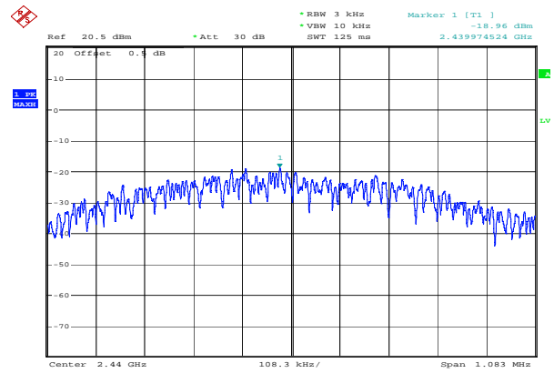
Middle -18.96 dBm/3kHz
