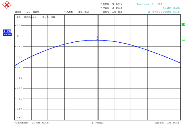
High -4.29 dBm
