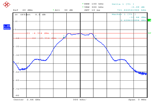
Middle 0.722 MHz
