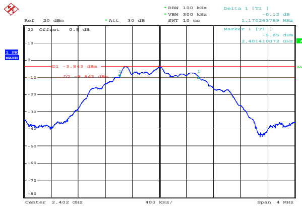
Low 1.170 MHz
