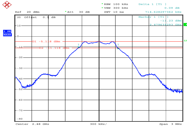
High 0.715 MHz
