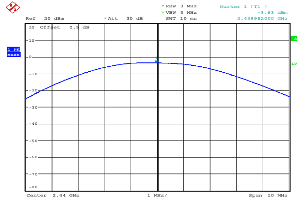
Middle -3.63 dBm
