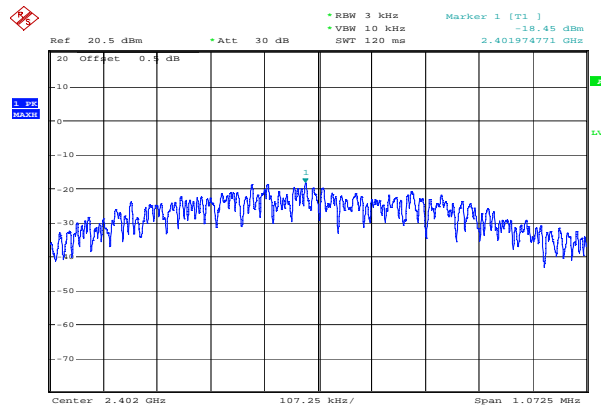
Low -18.45 dBm/3kHz
