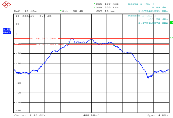
High 1.173 MHz
