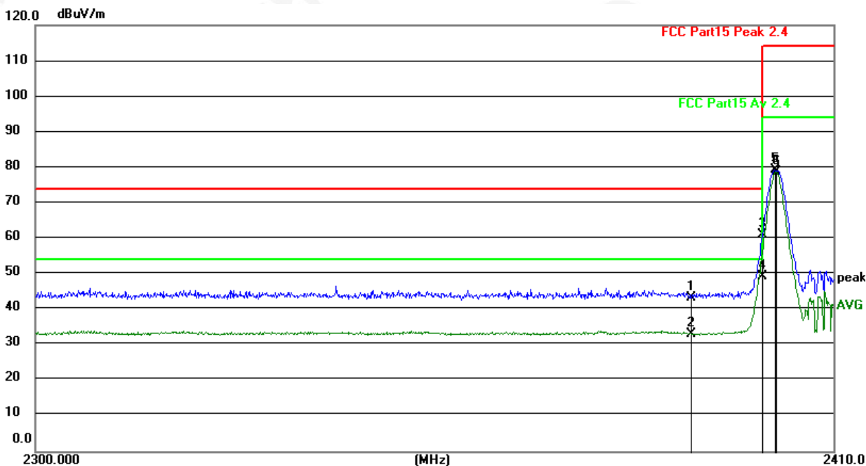
2402MHz Horizontal
