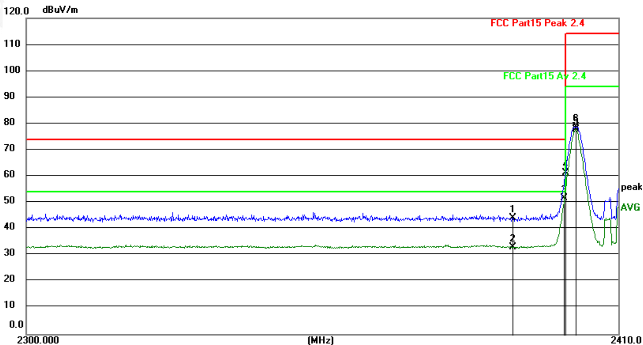
2402MHz Horizontal
