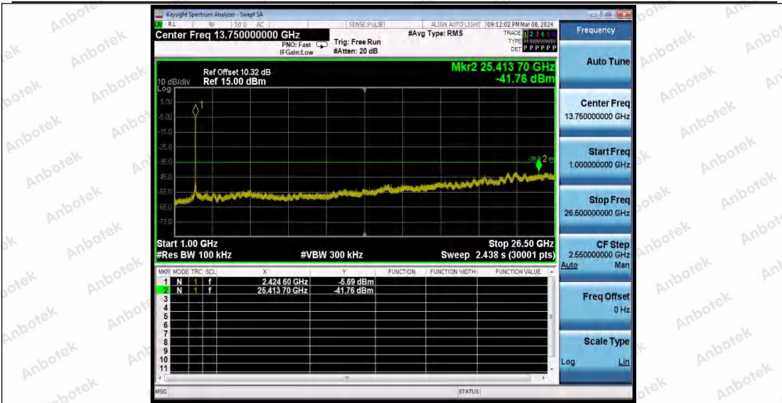
802.11n(HT40) SISO_Ant1_2437_0~Reference
