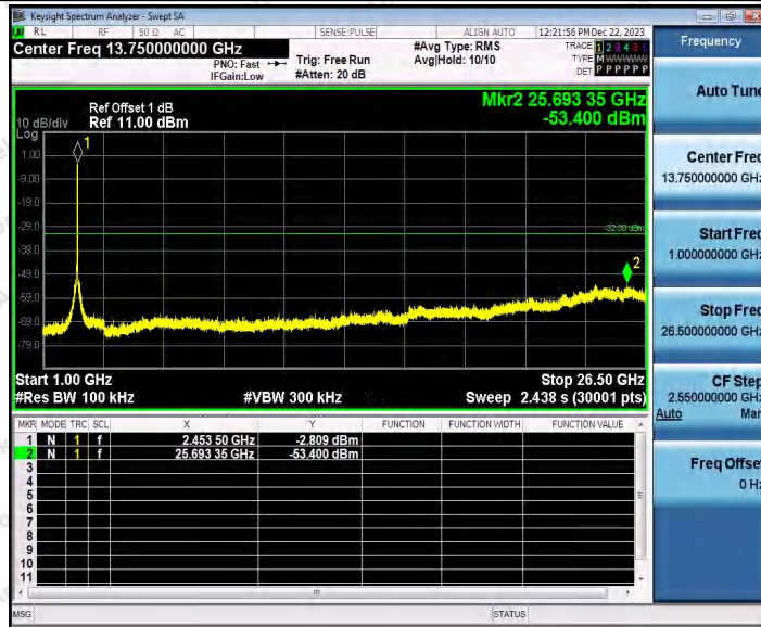
802.11n(HT40)SISO_Ant2_2452_0~Reference
