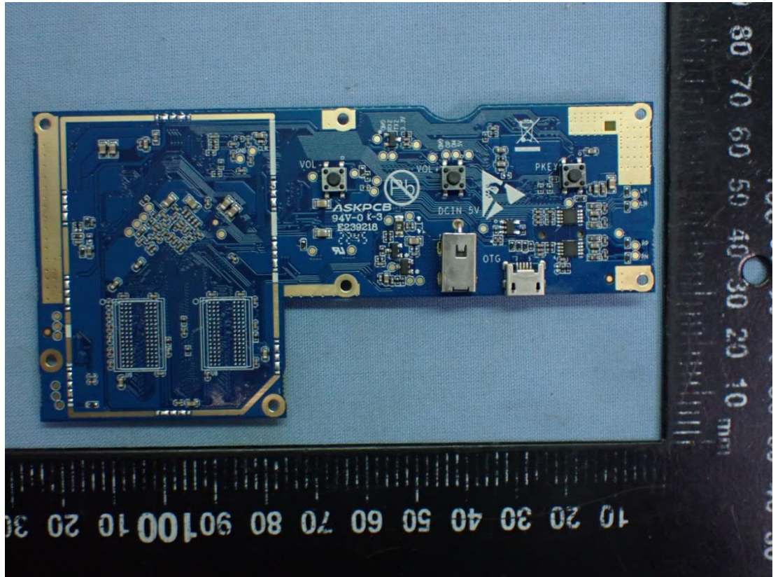
Figure 36 Internal View (Main Board, Back View)
