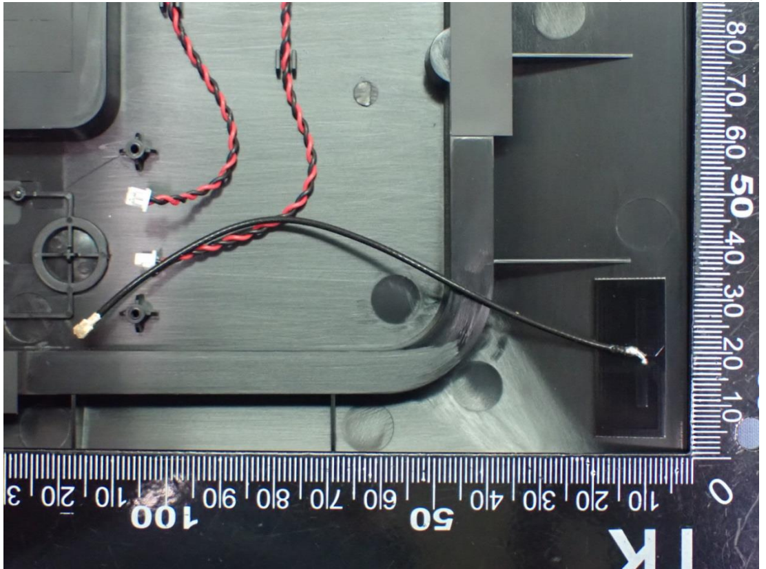
Figure 40 Internal View (RF Antenna)
