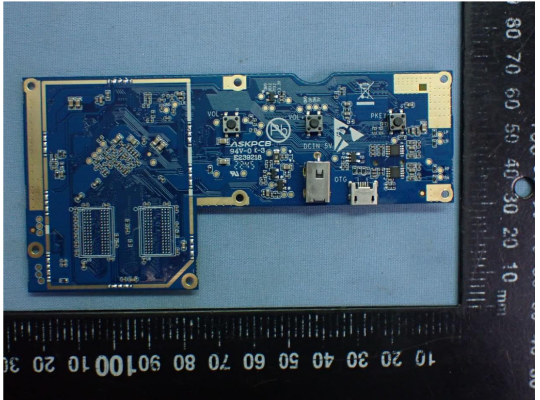
Figure 22 Internal View (Main Board, Back View)
