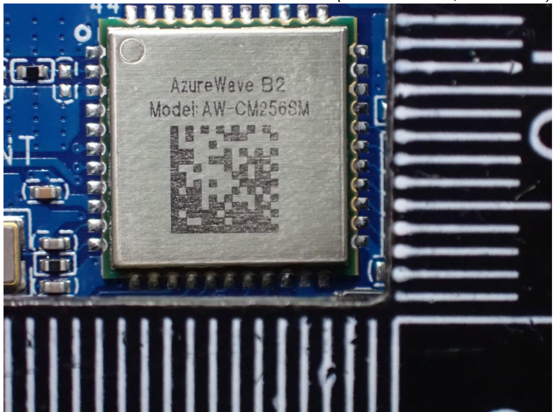
Figure 37 Internal View (WLAN Module, Front View)
