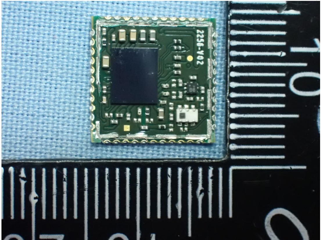
Figure 24 Internal View (WLAN Module, Front View/Removed Shielded Cover)
