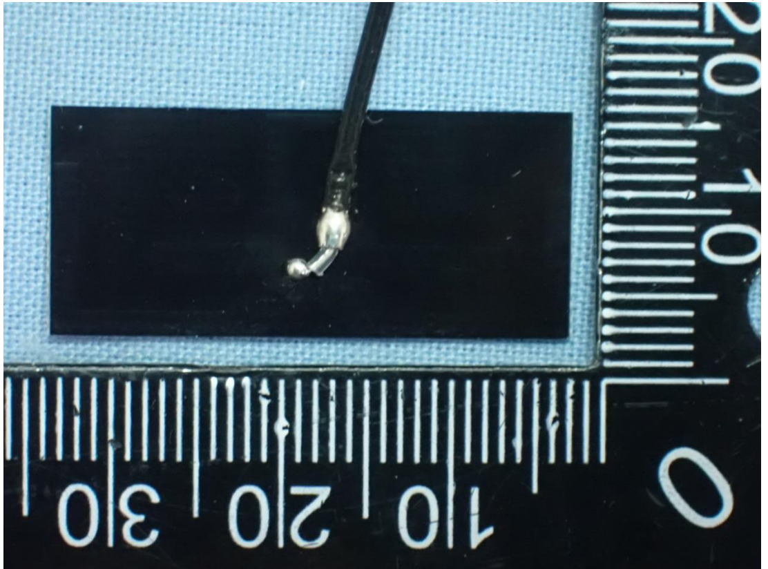
Figure 42 Internal View (RF Antenna, Back View)
