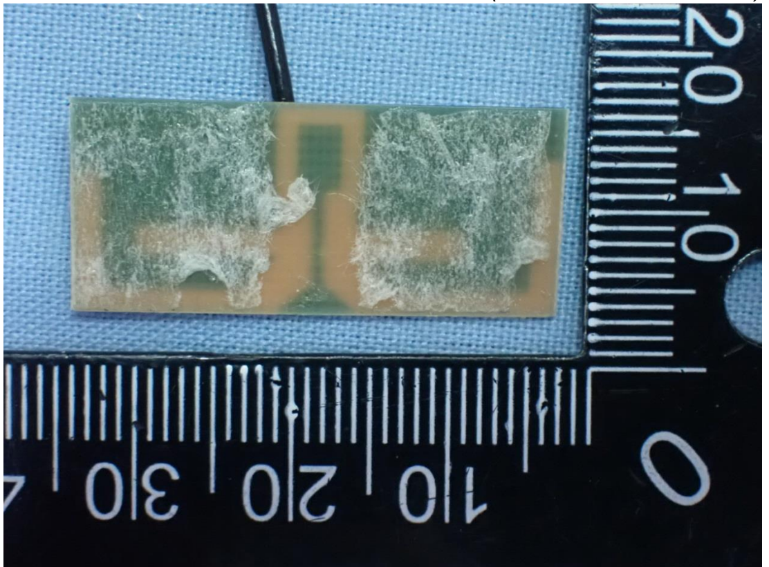
Figure 27 Internal View (RF Antenna, Front View)
