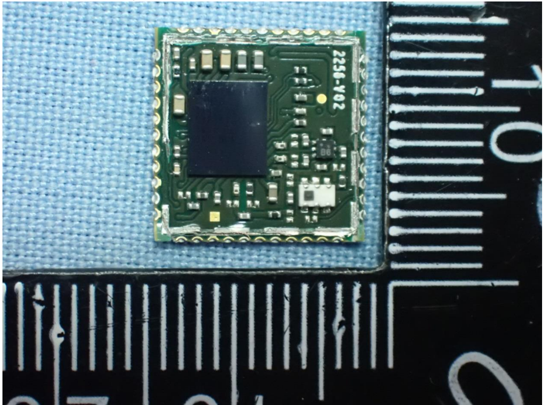
Figure 38 Internal View (WLAN Module, Front View/Removed Shielded Cover)
