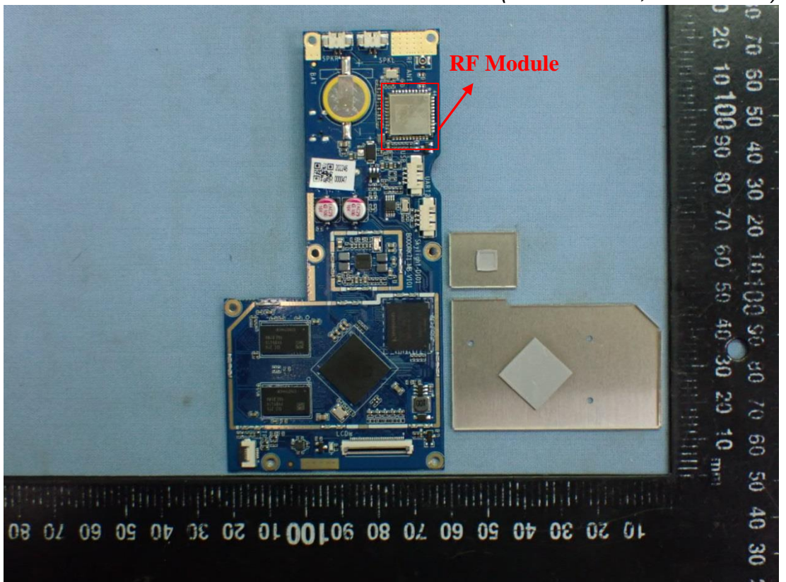
Figure 21 Internal View (Main Board, Front View)
