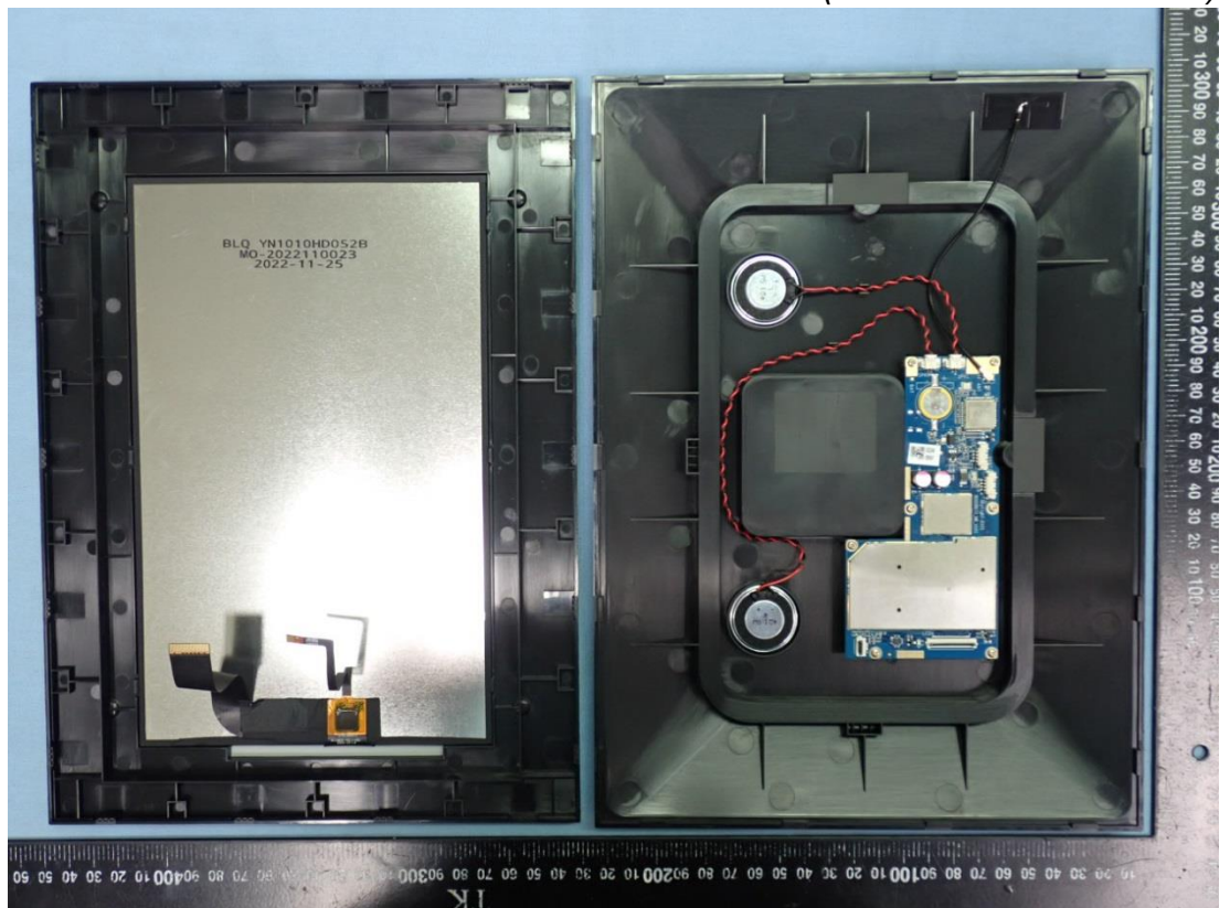
Figure 29 Internal View (Removed Back Cover)
