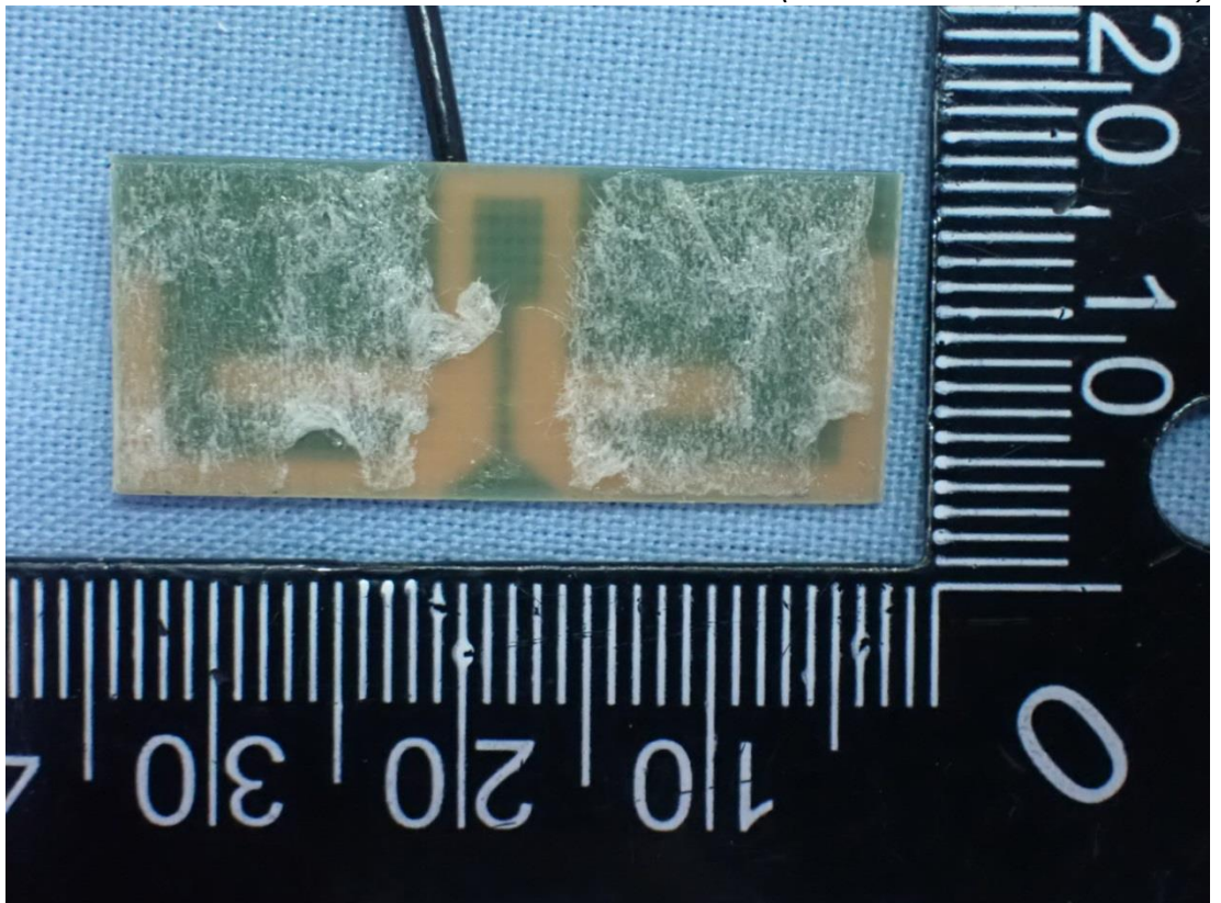
Figure 41 Internal View (RF Antenna, Front View)
