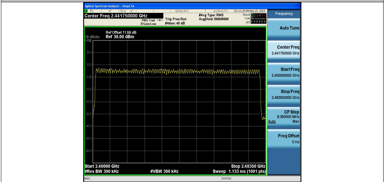
3DH5-Ant1-Hop-PASS
