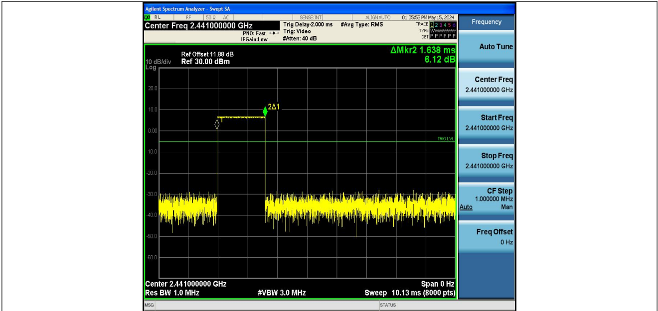
DH3-Ant1-Hop-PASS
