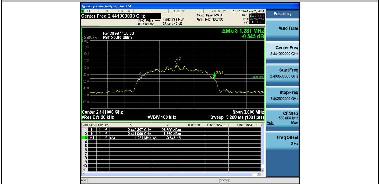
2DH5-Ant1-2441
