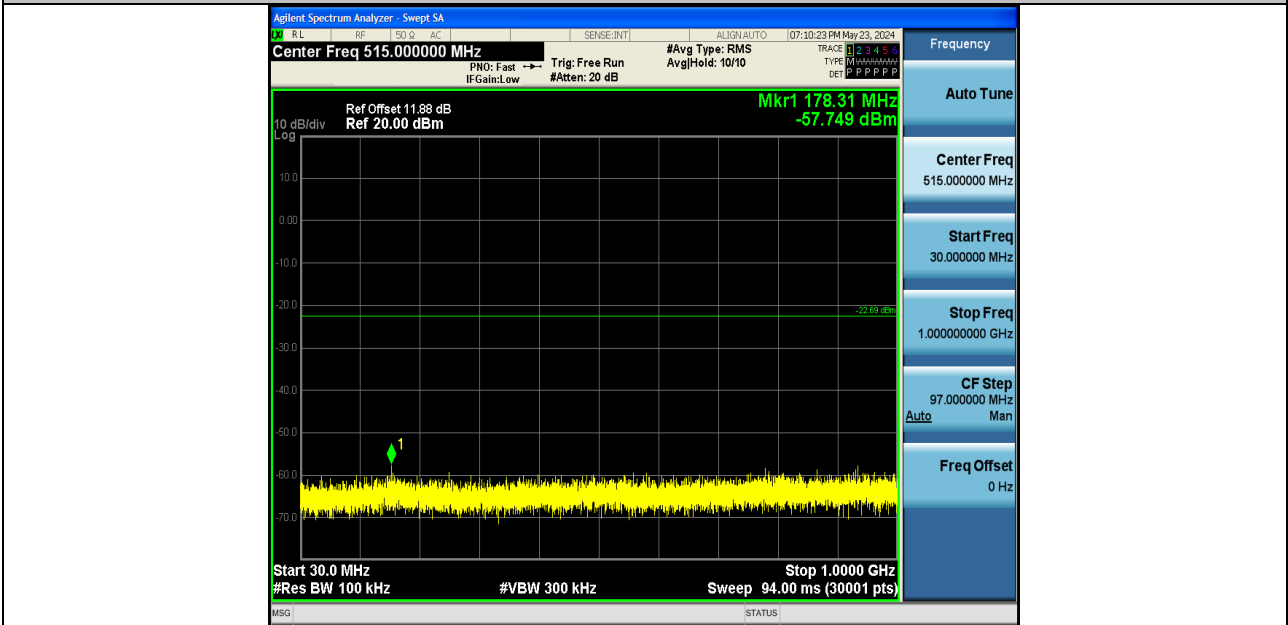
3DH5-Ant1-2441-30~1000-PASS
