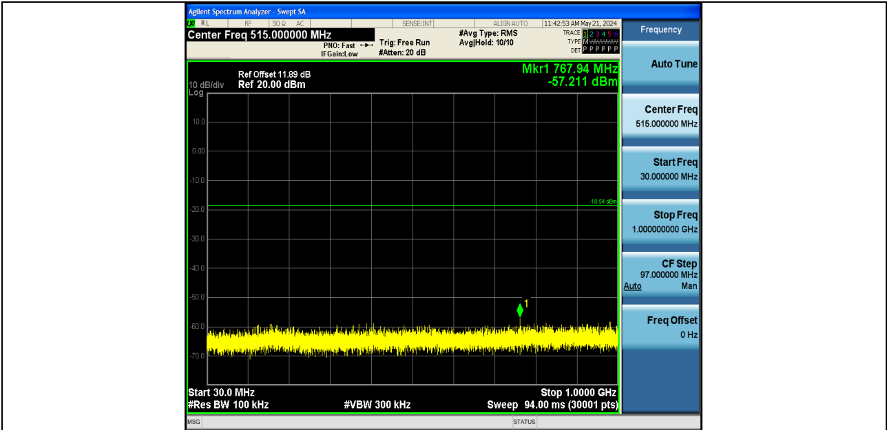
3DH5-Ant1-2402-30~1000-PASS
