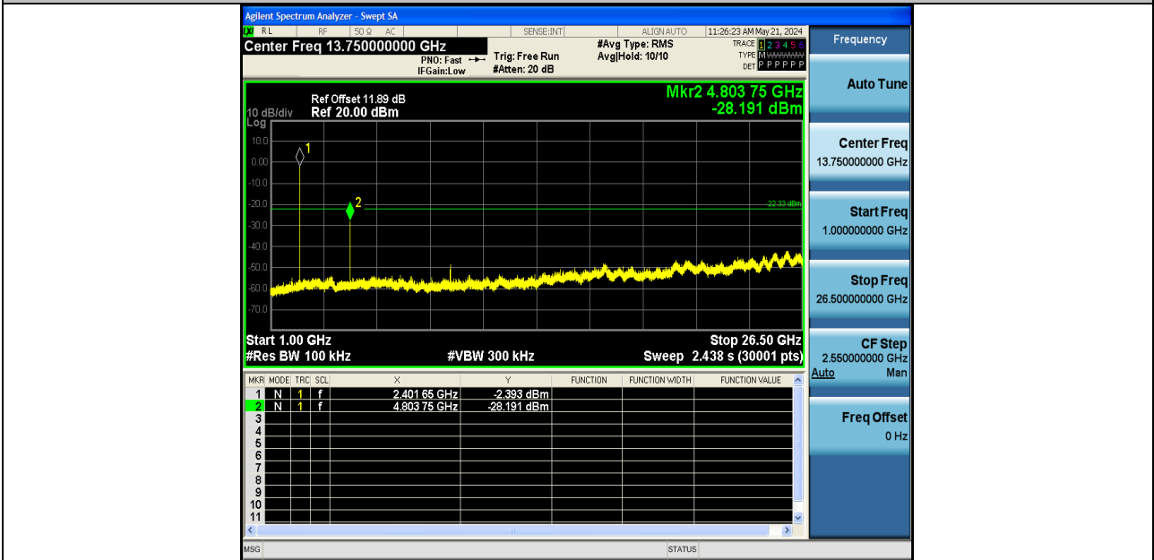
2DH5-Ant1-2402-1000~26500-PASS
