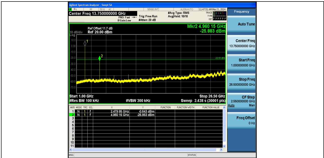
3DH5-Ant1-2480-1000~26500-PASS
