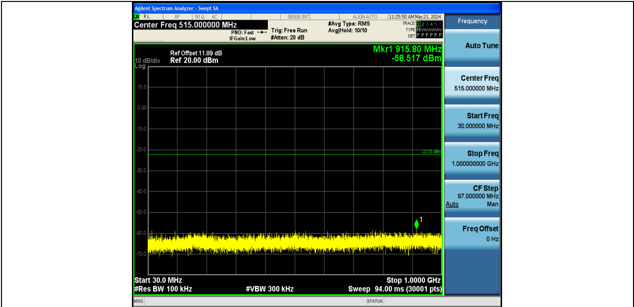
2DH5-Ant1-2402-30~1000-PASS
