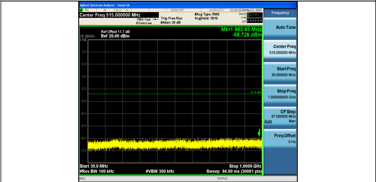
2DH5-Ant1-2480-30~1000-PASS
