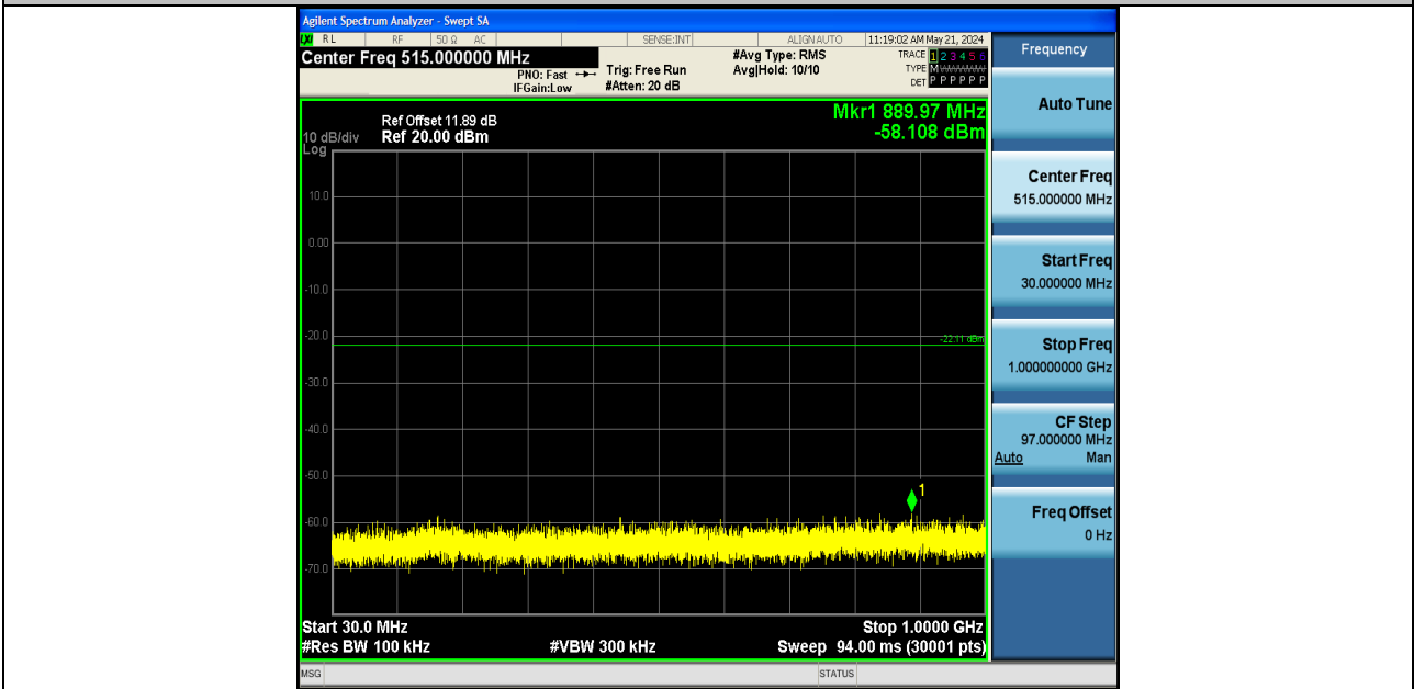
DH5-Ant1-2402-30~1000-PASS
