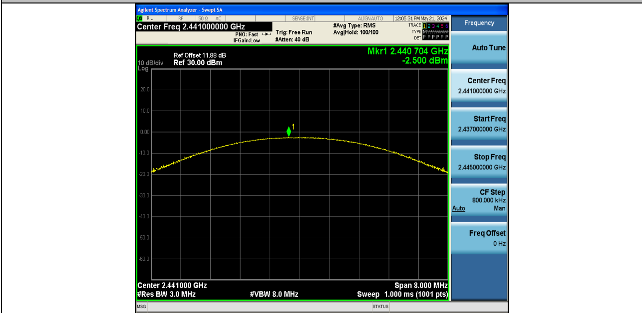
DH5-Ant1-2441-PASS
