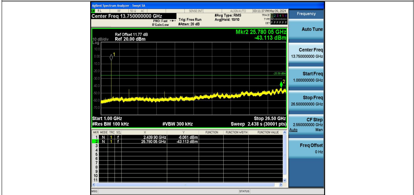
BLE_1M-Ant1-2440-1000~26500-PASS
