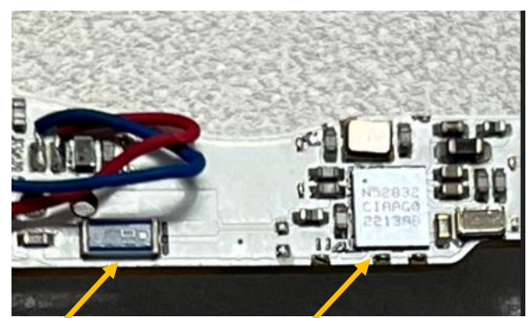
Chip Antenna
