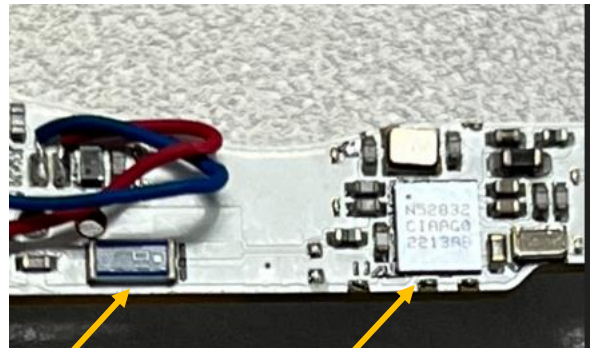
Chip Antenna
