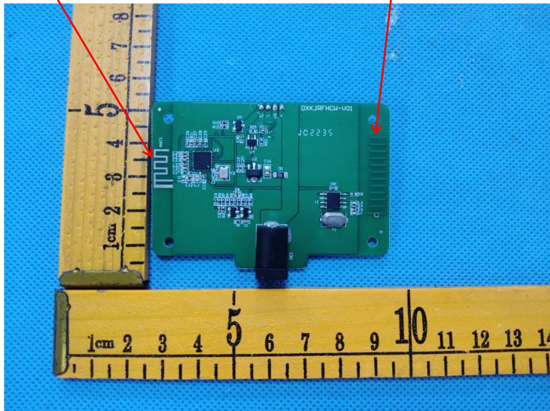
433MHz Antenna(Receiving)
