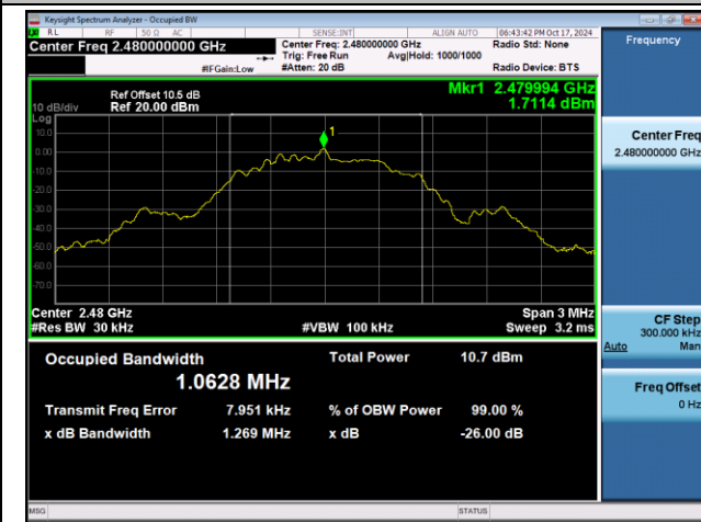
BLE_1M-Ant1-2480
