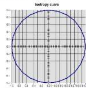
Isotropy +/-5.15% (+/-0.01dB)
