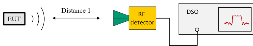
Fig. 1: Test setup 1. EIRP_{EUT} - FSL_1 + AG_{meas} = P_{detector}
