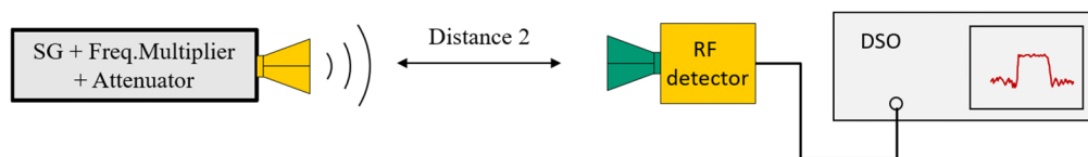
Fig. 2: Test setup 2. P_{SG} + AG_{TX} - FSL_2 + AG_{meas} = P_{detector}
