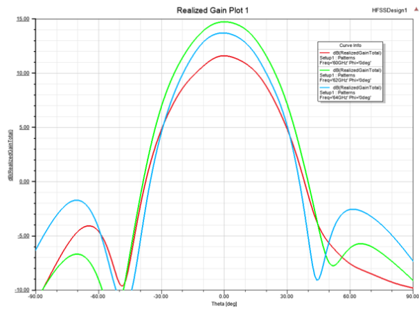
Azimuth/Horizontal
