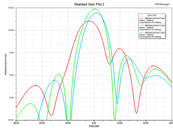
Elevation/Vertical
