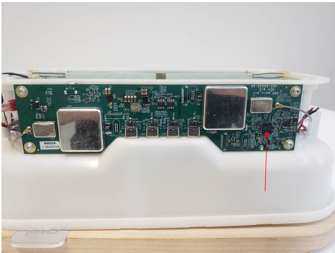
Figure 1. Main PCB Board Installed
