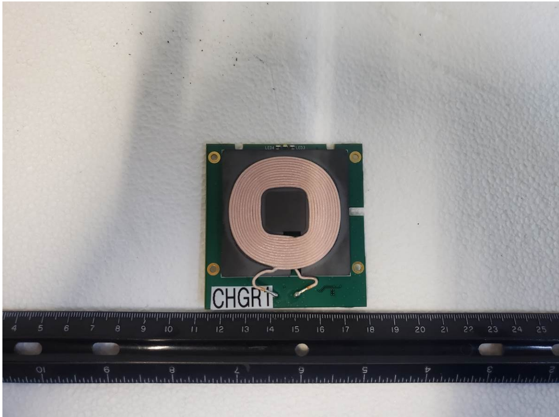
Figure 8. Front of Wireless Charging coil
