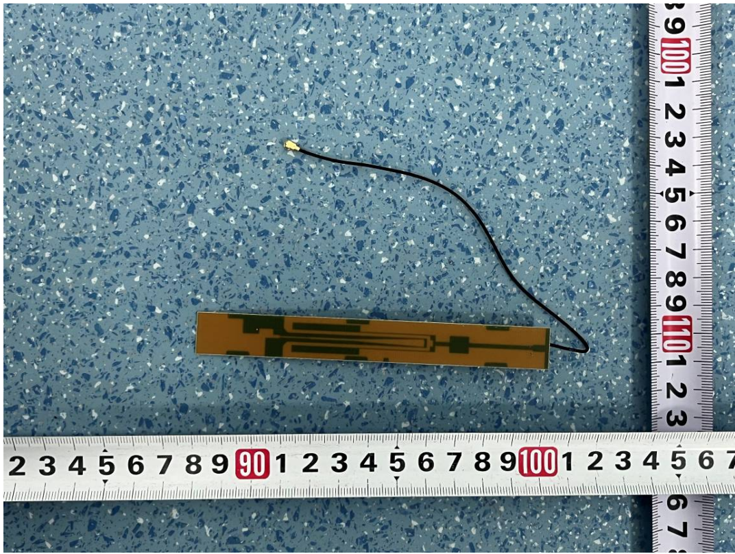
UHF RX Antenna 1
