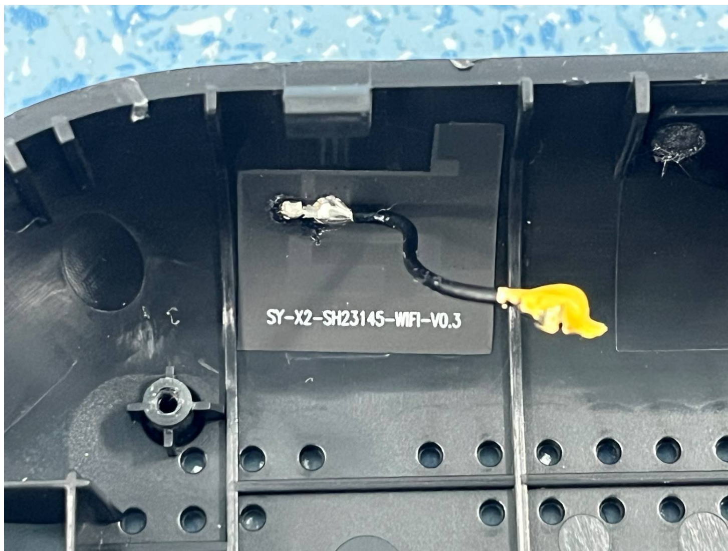
WIFI ANT
