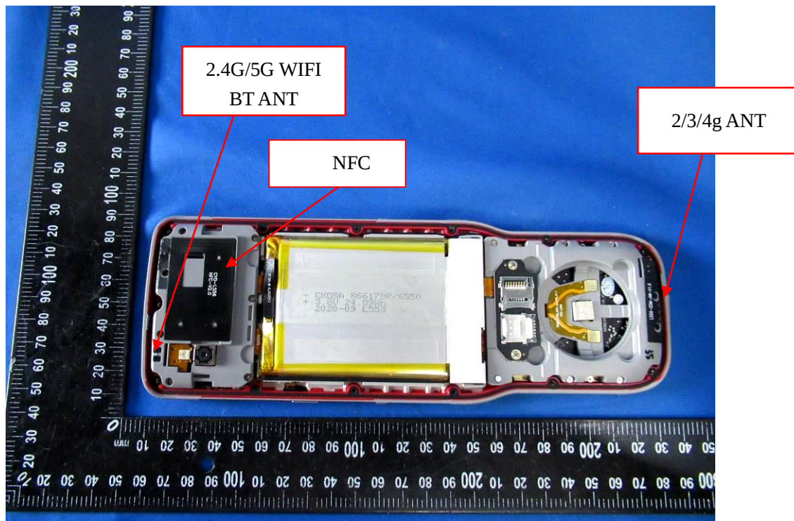
2/3/4g ANT
