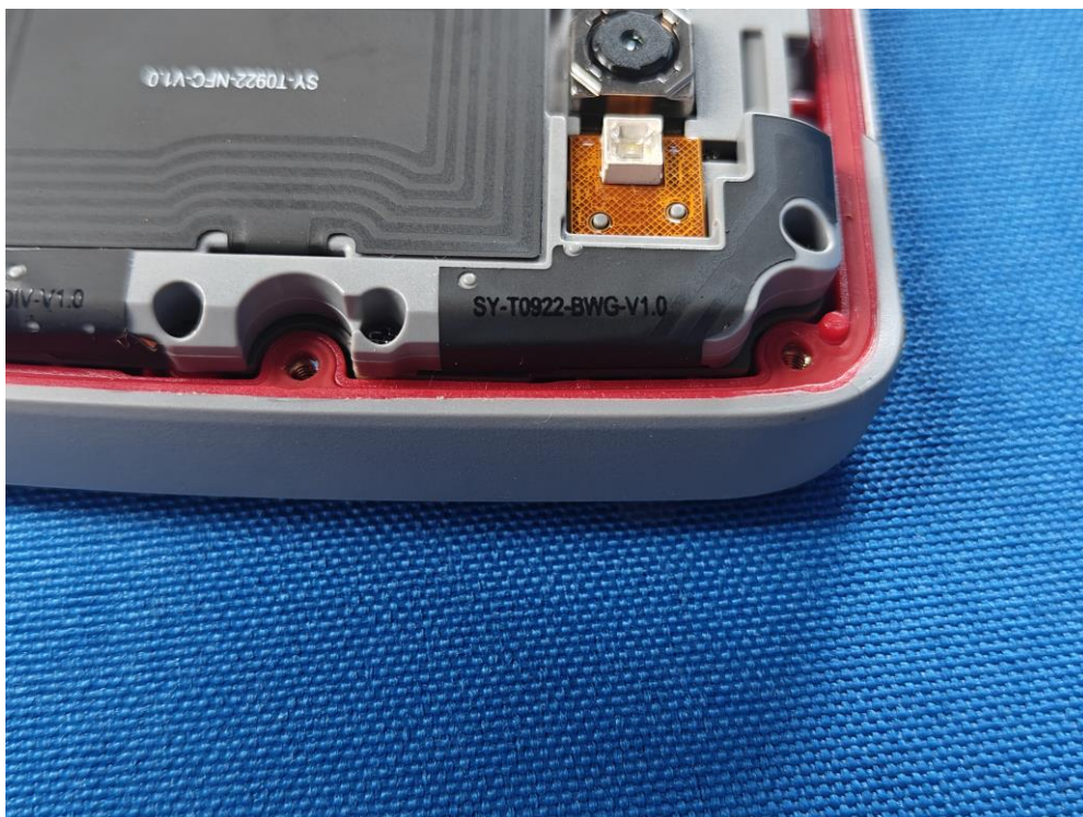
2.4G/5G WIFI BT ANT
