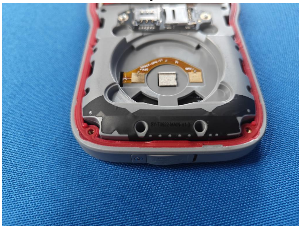
2/3/4g ANT
