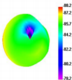
Bluetooth 0 TIS
