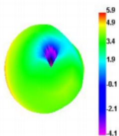
Bluetooth 0 TRP
