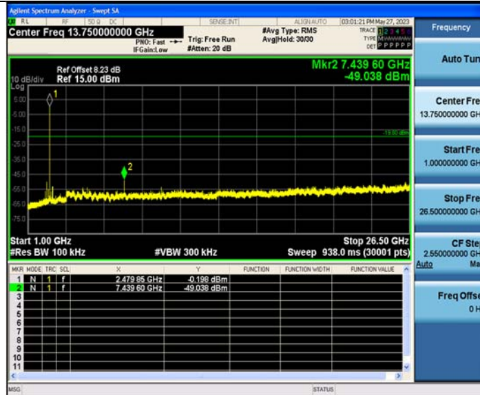
2DH5_Ant2_2480_0~Reference
