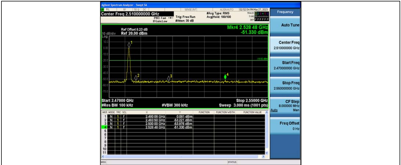
DH5_Ant2_High_2480
