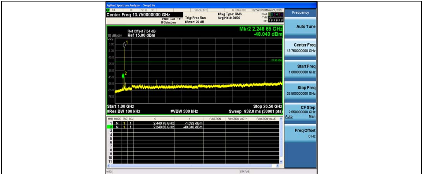
2DH5_Ant2_2441_0~Reference
