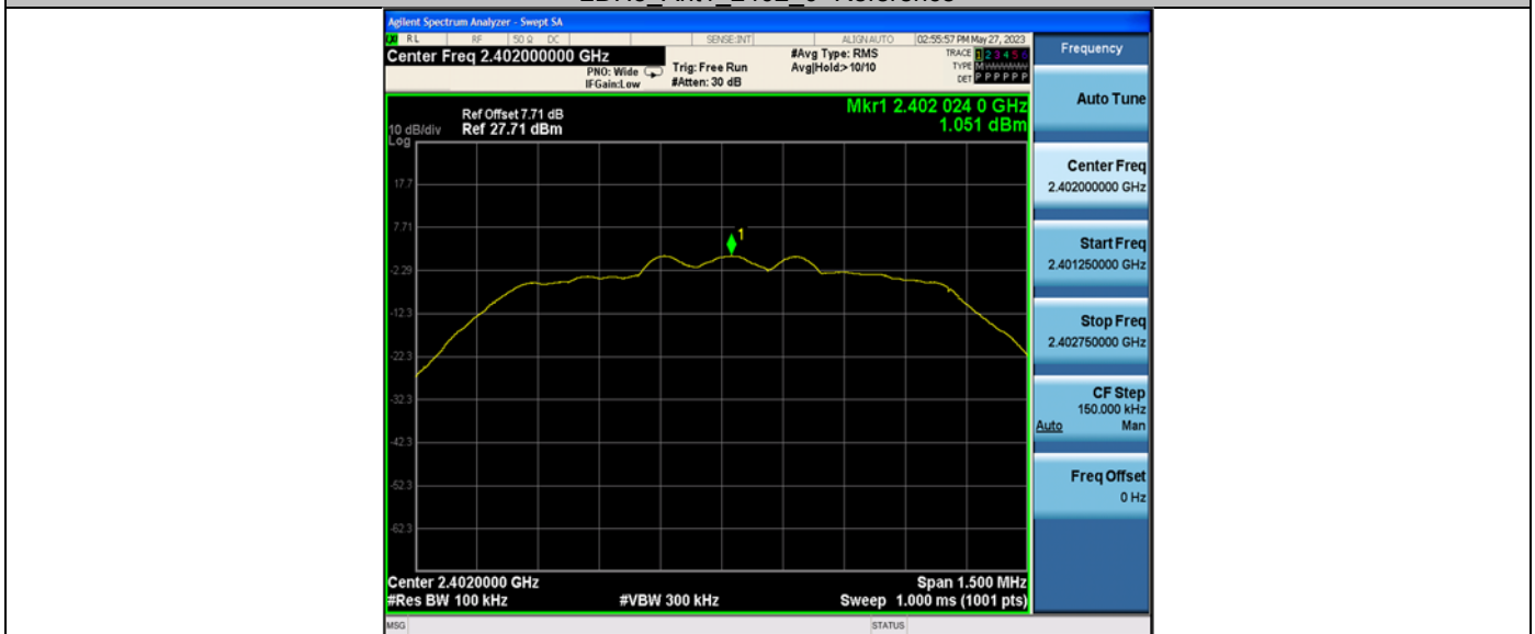
2DH5_Ant1_2402_30~100
