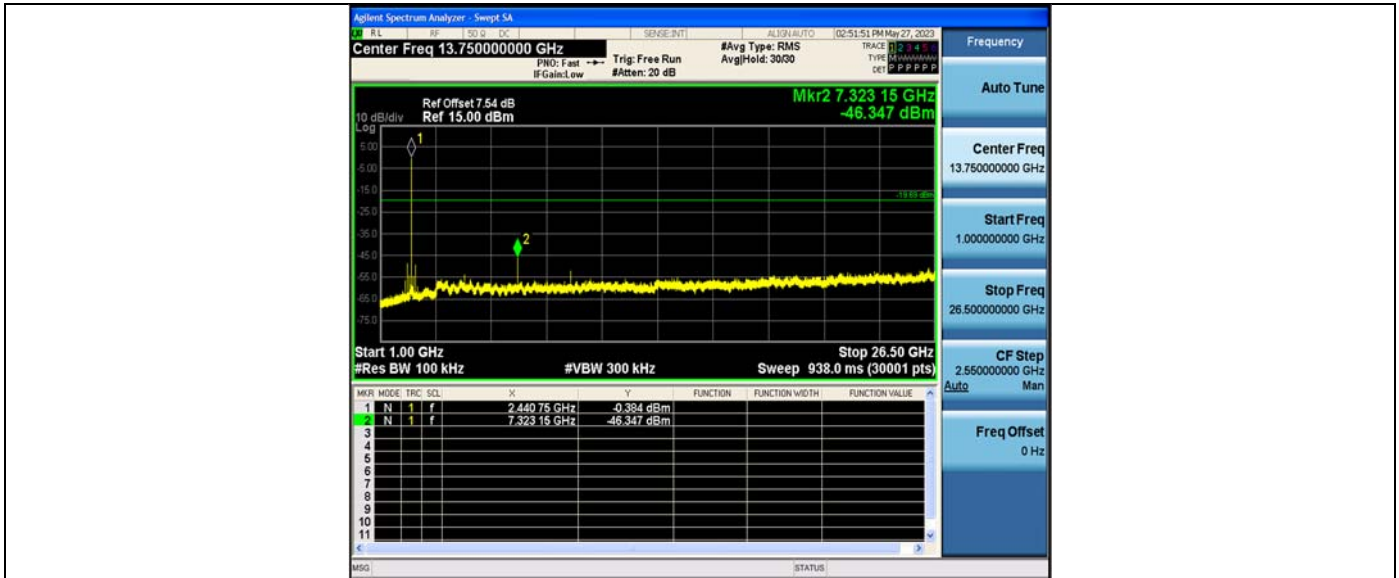
DH5_Ant2_2441_0~Reference
