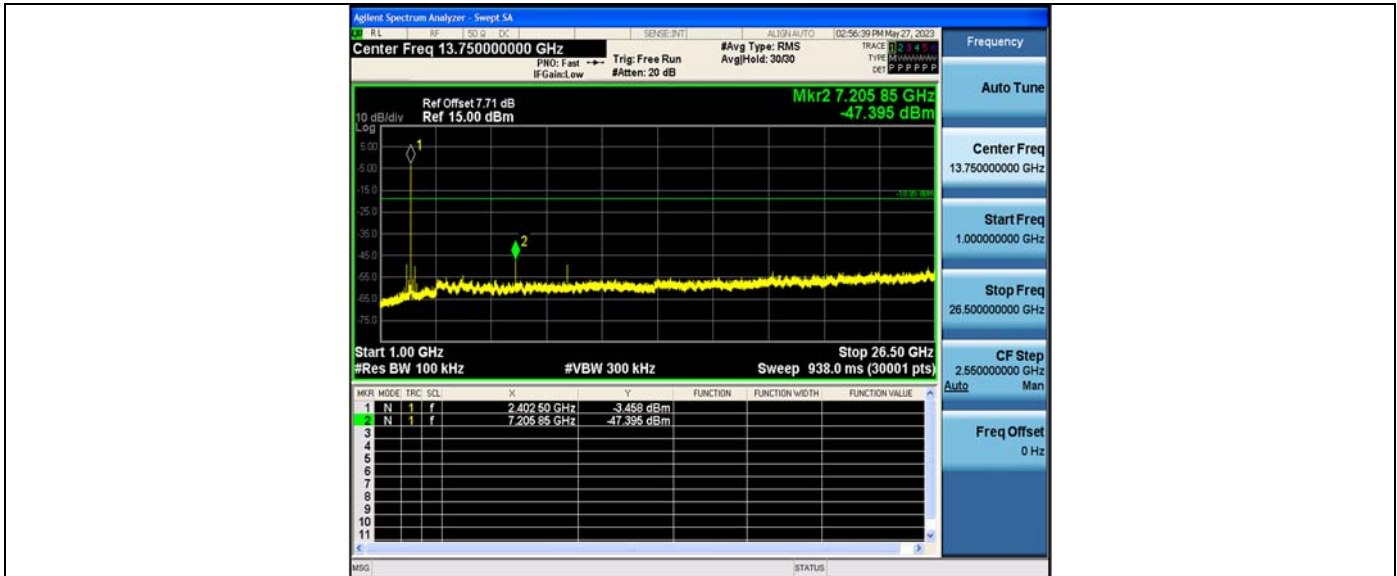
2DH5_Ant2_2402_0~Reference
