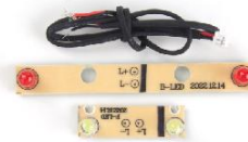
Front and rear light assembly
