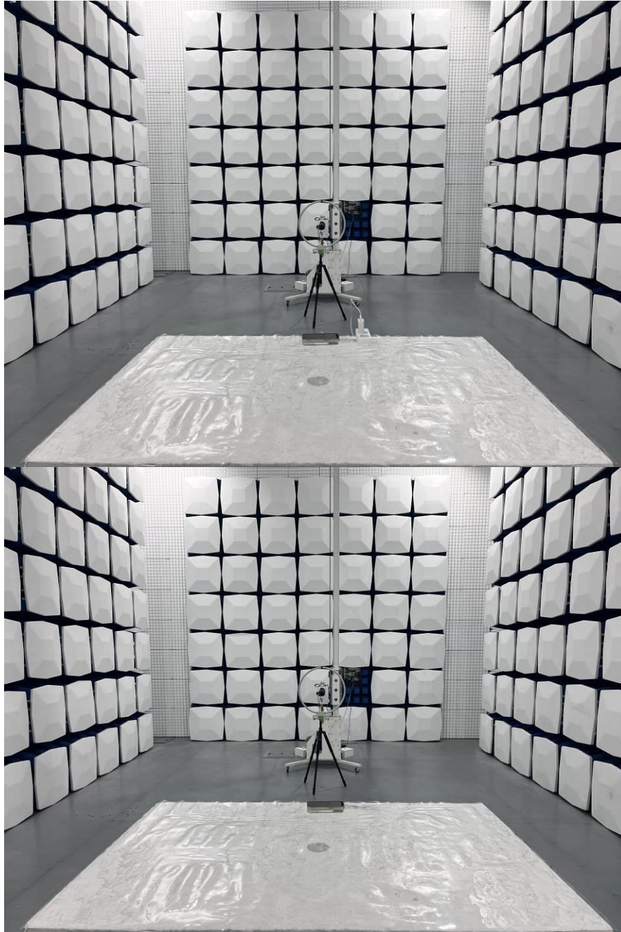
Radiated Emission
