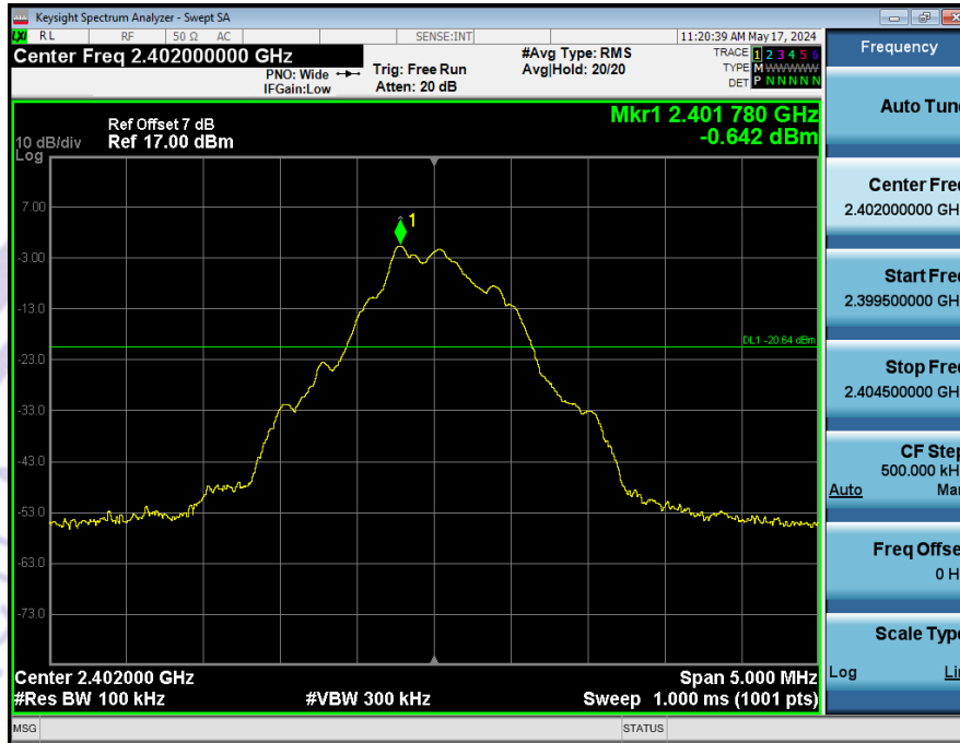
GFSK: Band Edge, Left Side
