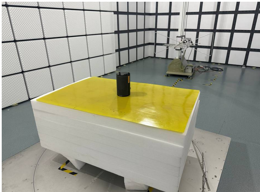
Photo of Radiated Emission Measurement (Below 1G)
