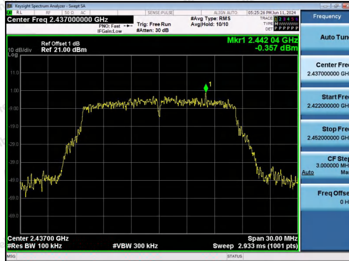
11G-Ant1-2437-0~Reference-PASS
