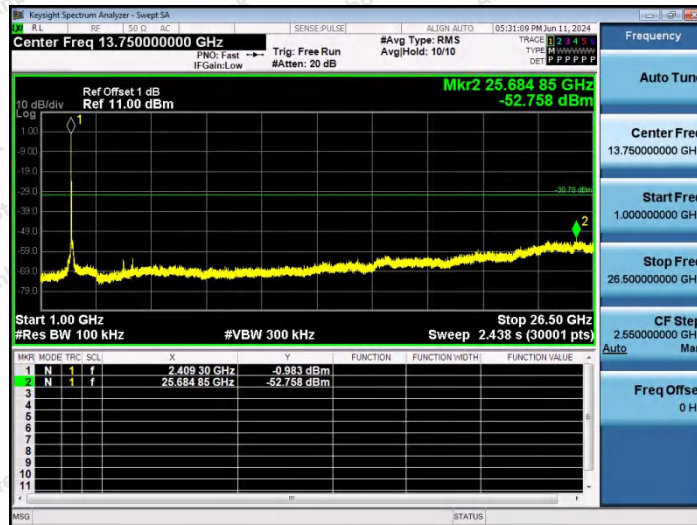
11N20SISO-Ant1-2412-1000~26500-PASS
