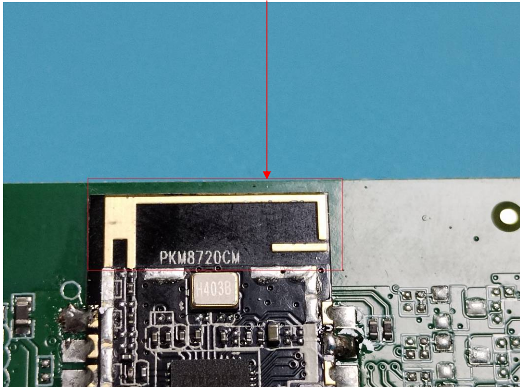
Wi-Fi Antenna
