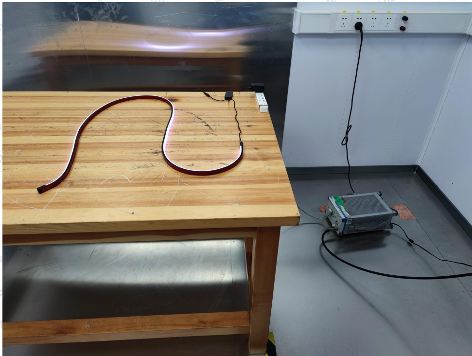
For Model: H61C2 Photo of Conducted Emission Measurement
