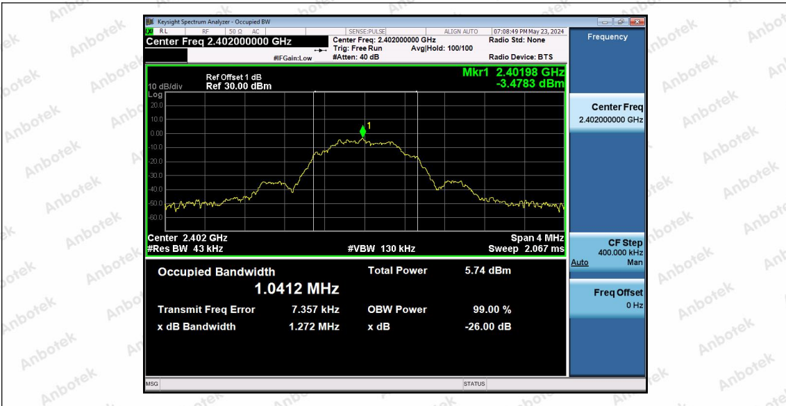
BLE_1M-Ant1-2402
