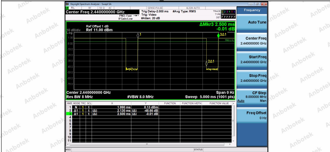
NTNV-BLE 1M-Ant1-2440
