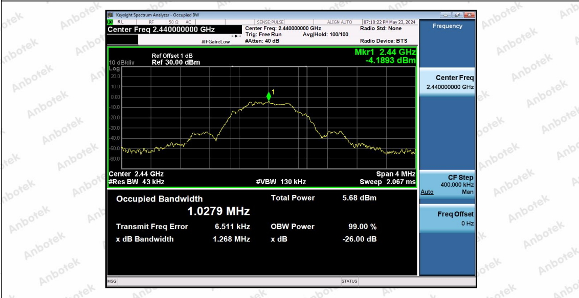
BLE_1M-Ant1-2440
