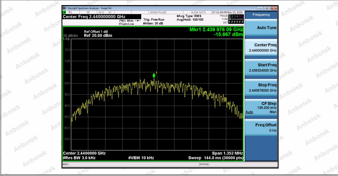
BLE_1M-Ant1-2440-PASS
