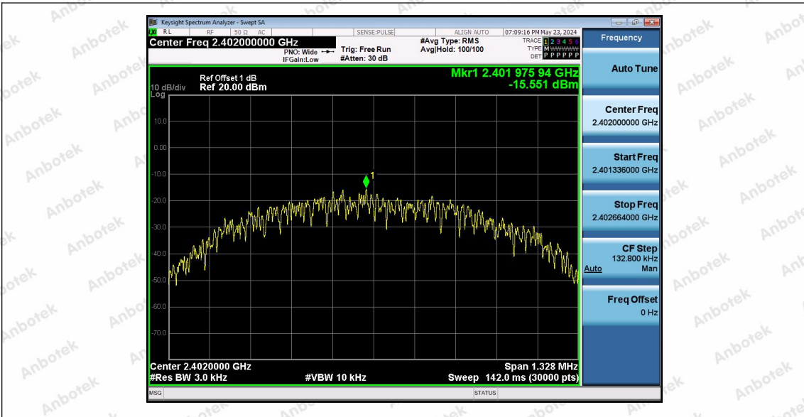
BLE_1M-Ant1-240-PASS
