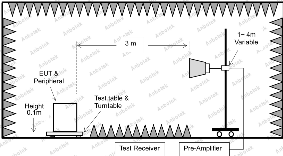
Figure 3. Above 1 GHz
