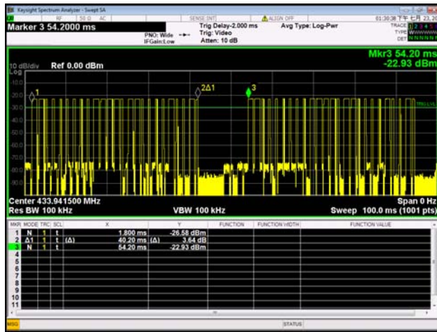
Pulse T_{on}
