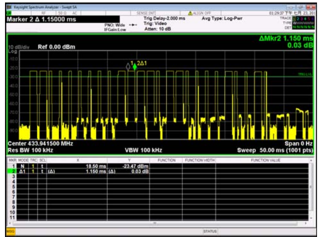
Pulse T_{on}
