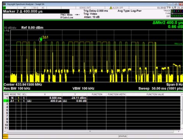
Pulse T_{on}
