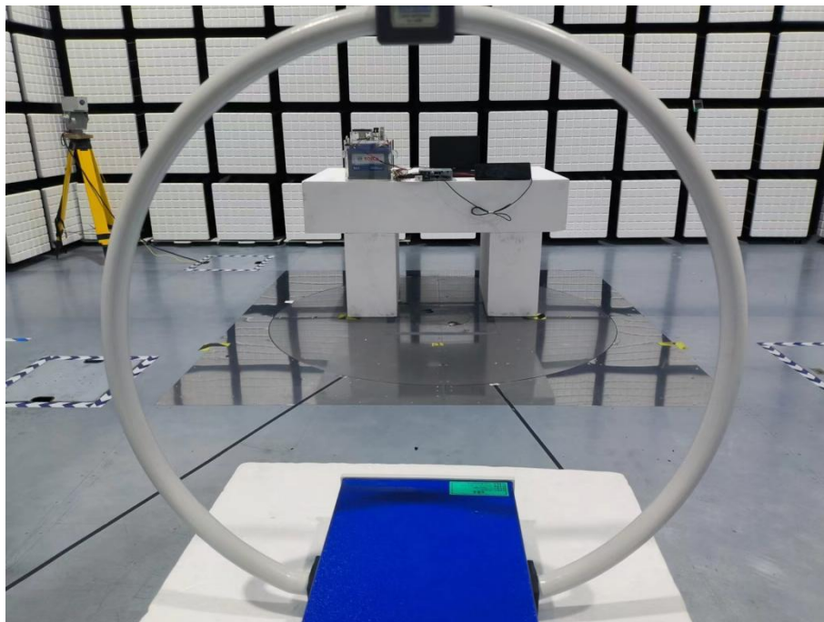
Description: Radiated Emission Test Setup (Below 30MHz)
