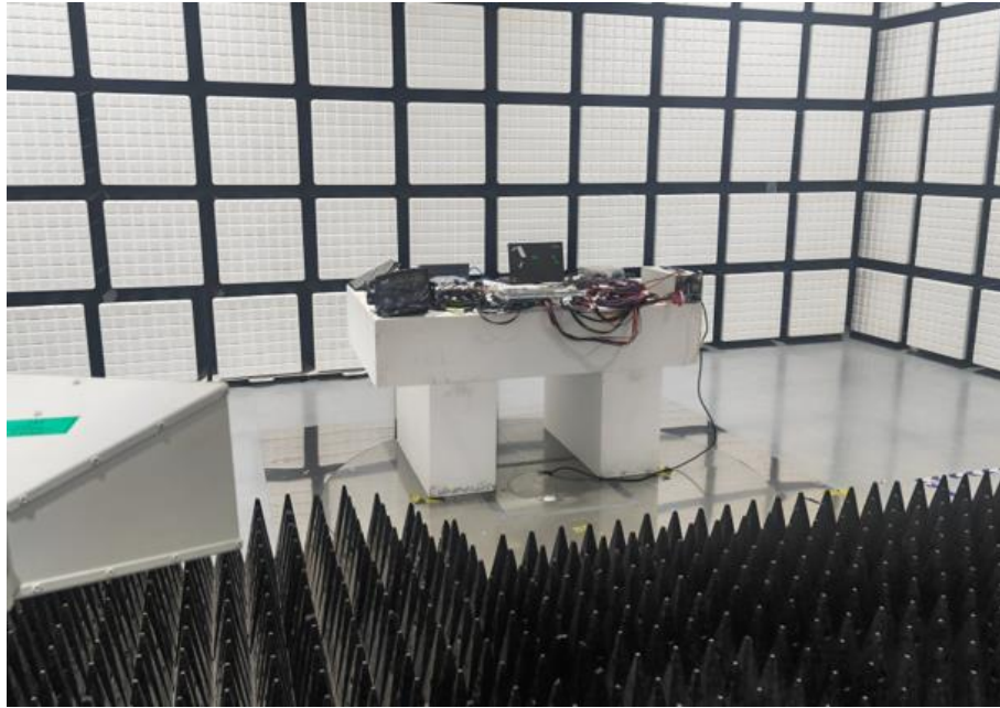
Description: Back view of Radiated Emission Test Setup (Above 1GHz)
