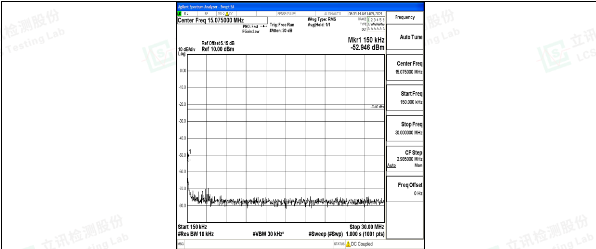
Band71_20MHz_QPSK_133372_1RB#0_0.15~30_0.15~30
