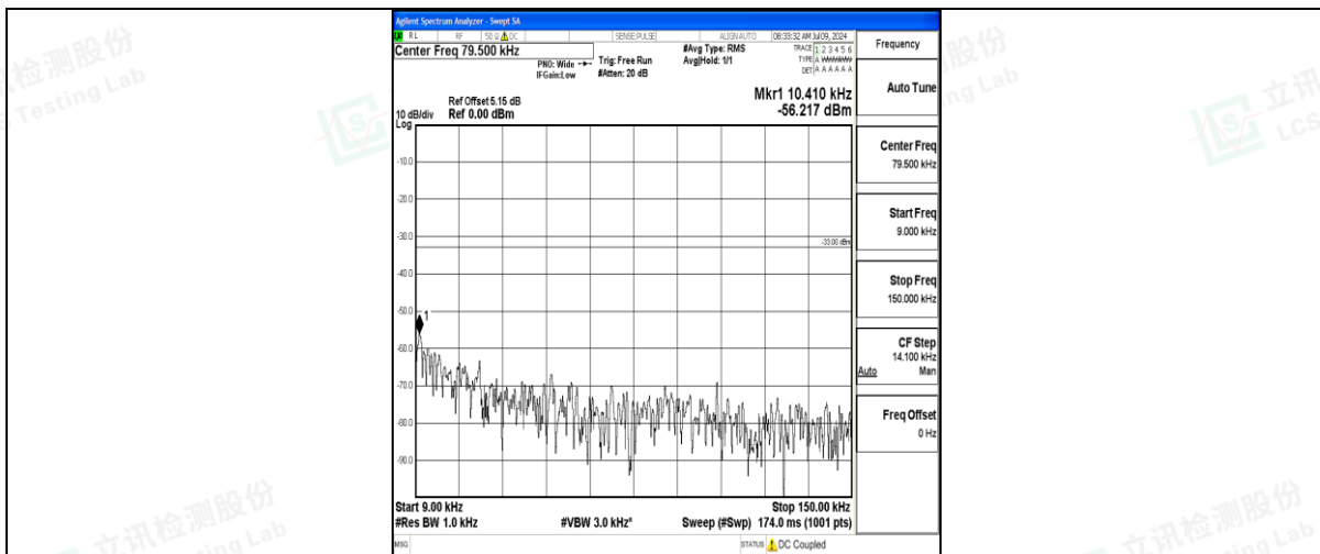
Band71_20MHz_QPSK_133222_1RB#0_0.009~0.15_0.009~0.15
