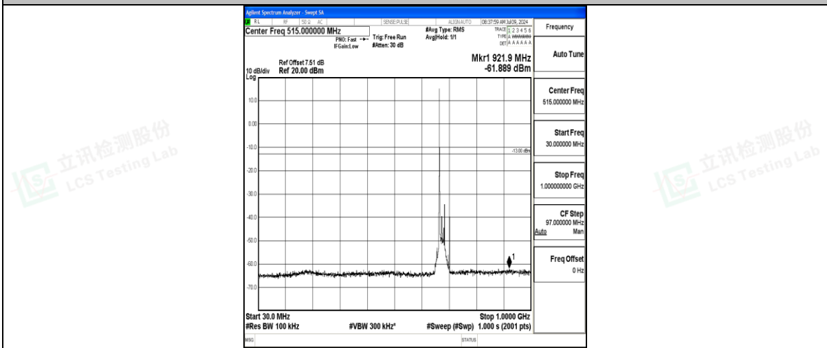
Band71_20MHz_16QAM_133322_1RB#0_30~1000_30~1000
