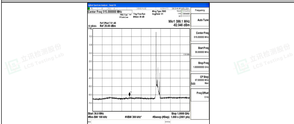
Band71_20MHz_QPSK_133222_1RB#0_30~1000_30~1000
