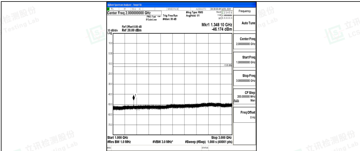
Band71_20MHz_16QAM_133322_1RB#0_1000~3000_1000~3000
