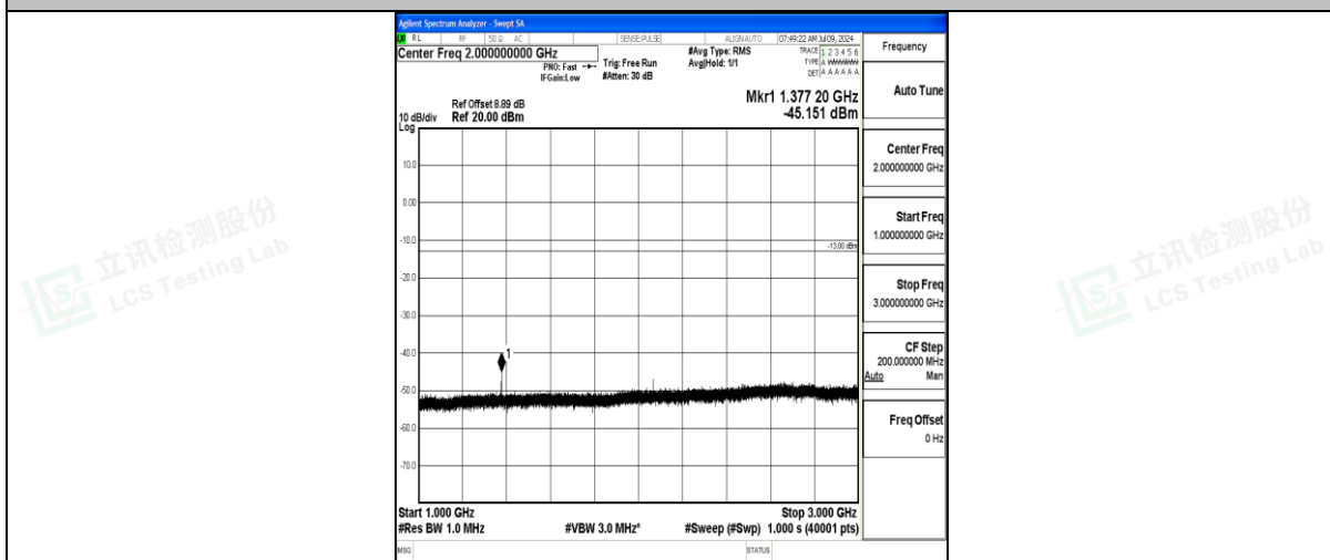
Band71_10MHz_16QAM_133422_1RB#0_1000~3000_1000~3000
