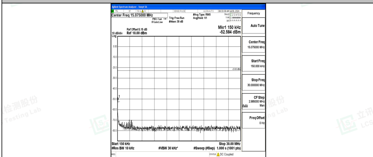
Band71_20MHz_QPSK_133222_1RB#0_0.15~30_0.15~30
