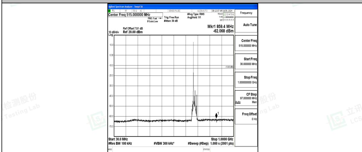
Band71_15MHz_16QAM_133297_1RB#0_30~1000_30~1000
