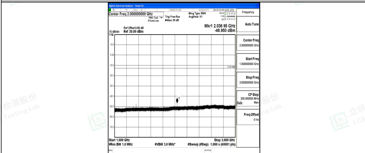
Band71_20MHz_QPSK_133372_1RB#0_1000~3000_1000~3000
