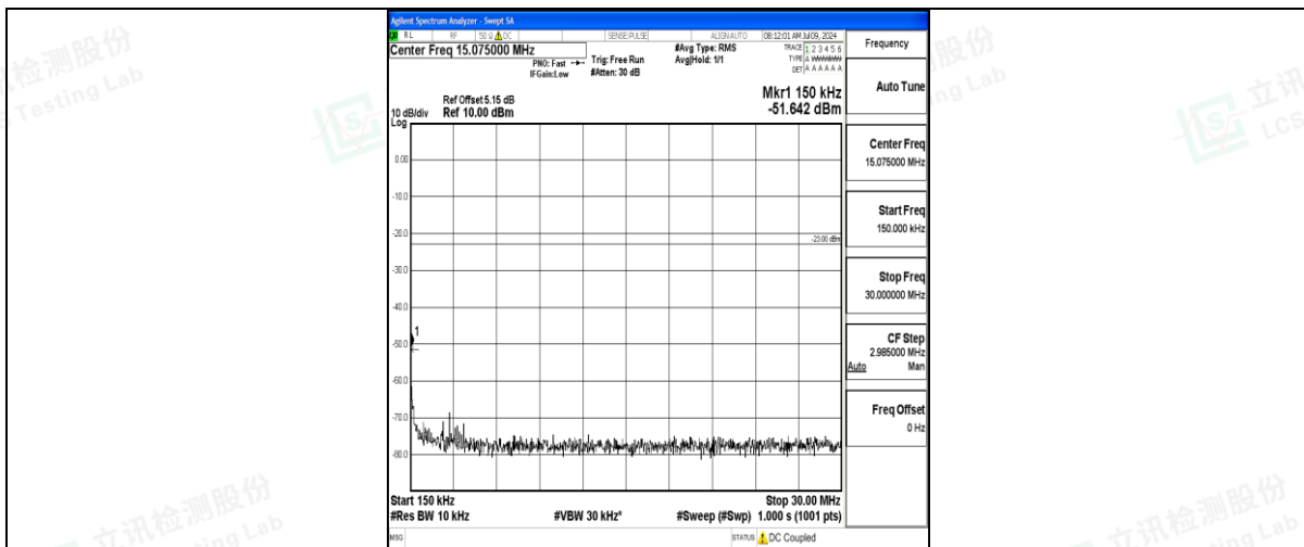
Band71_15MHz_16QAM_133297_1RB#0_0.15~30_0.15~30
