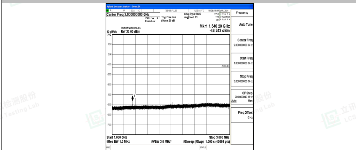
Band71_20MHz_QPSK_133322_1RB#0_1000~3000_1000~3000
