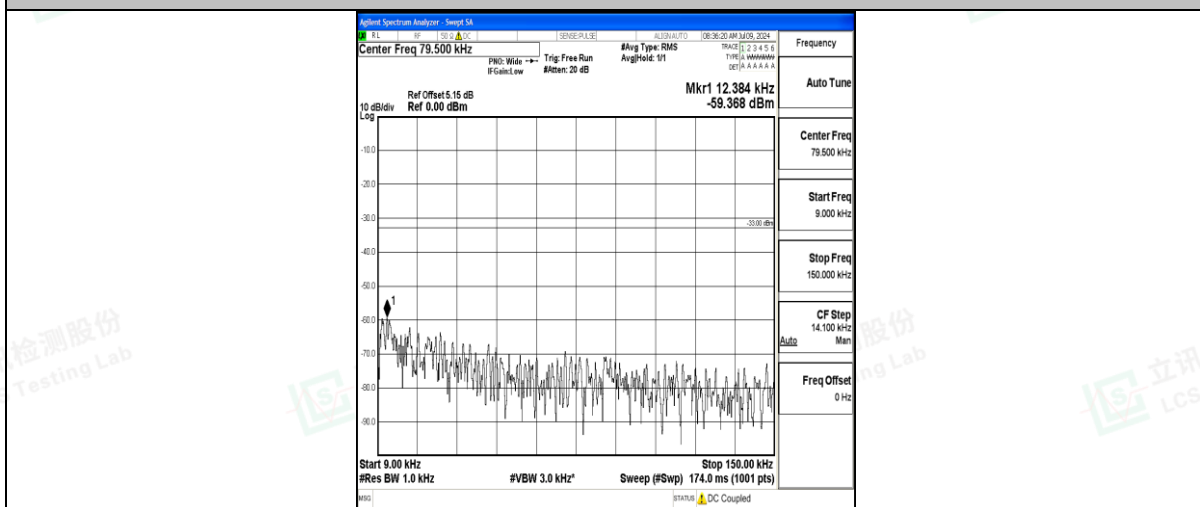
Band71_20MHz_QPSK_133322_1RB#0_0.009~0.15_0.009~0.15
