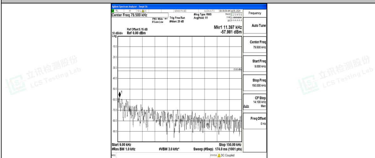
Band71_20MHz_QPSK_133372_1RB#0_0.009~0.15_0.009~0.15
