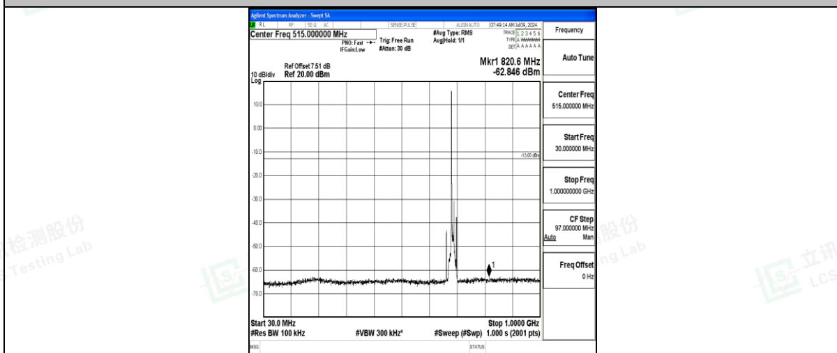
Band71_10MHz_16QAM_133422_1RB#0_30~1000_30~1000
