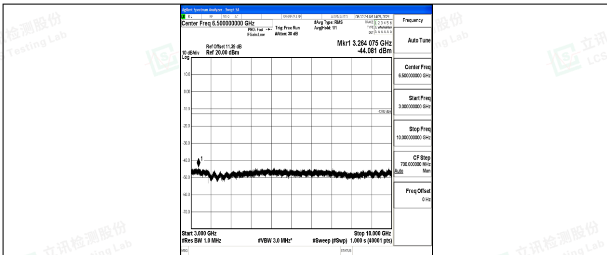
Band71_15MHz_16QAM_133297_1RB#0_3000~10000_3000~10000
