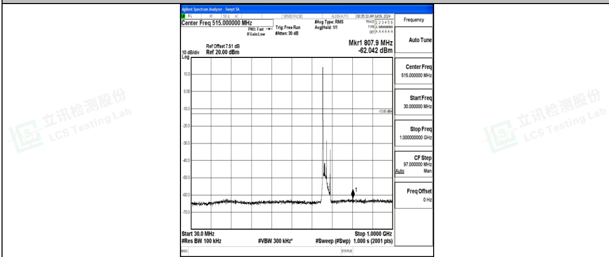
Band71_20MHz_16QAM_133222_1RB#0_30~1000_30~1000
