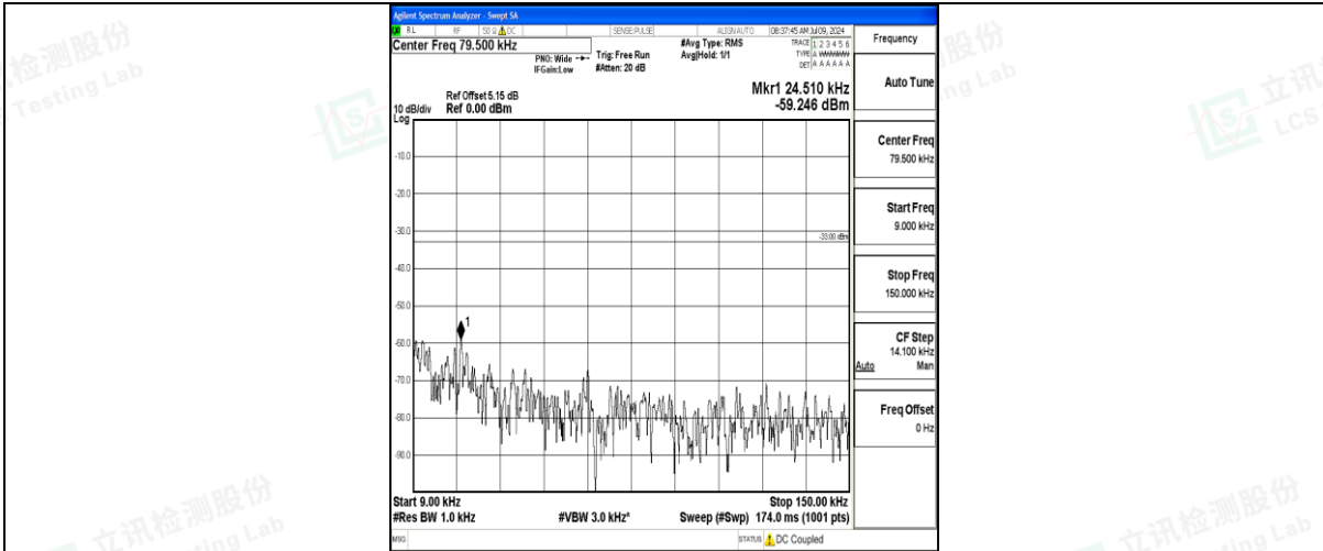
Band71_20MHz_16QAM_133322_1RB#0_0.009~0.15_0.009~0.15
