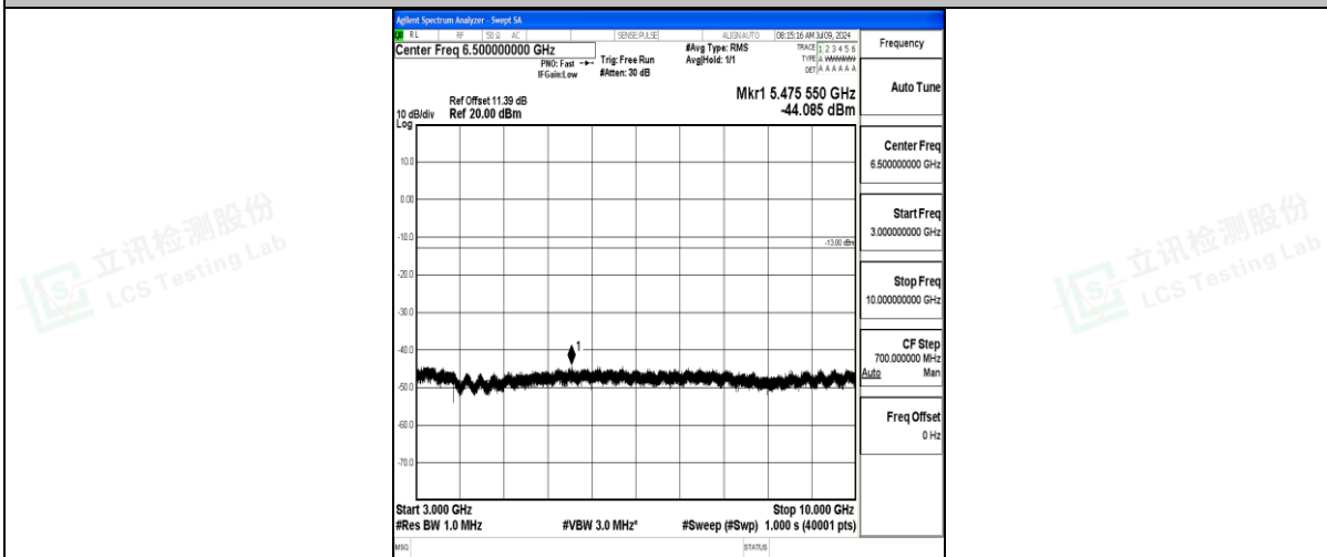
Band71_15MHz_16QAM_133397_1RB#0_3000~10000_3000~10000
