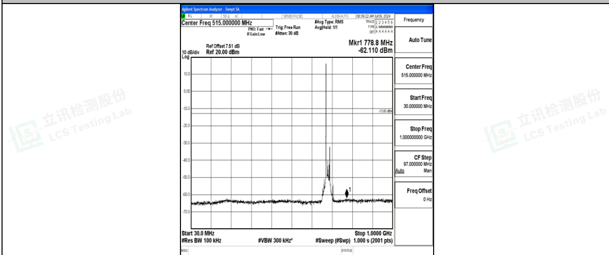
Band71_20MHz_QPSK_133372_1RB#0_30~1000_30~1000
