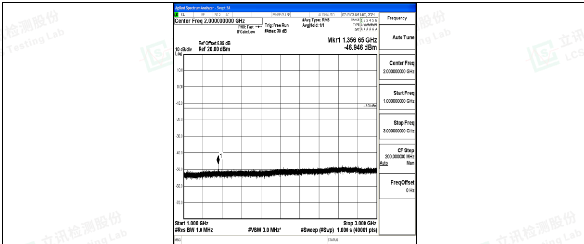
Band71_5MHz_16QAM_133297_1RB#0_1000~3000_1000~3000
