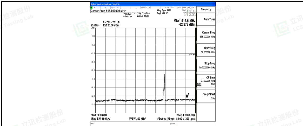
Band71_5MHz_16QAM_133447_1RB#0_30~1000_30~1000
