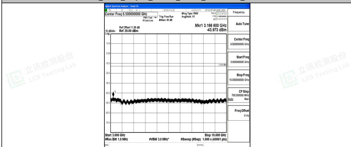
Band71_5MHz_16QAM_133447_1RB#0_3000~10000_3000~10000
