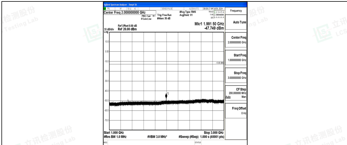
Band71_15MHz_QPSK_133197_1RB#0_1000~3000_1000~3000
