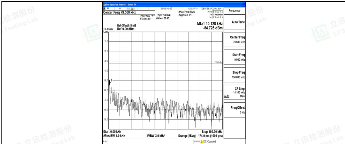
Band71_15MHz_QPSK_133197_1RB#0_0.009~0.15_0.009~0.15
