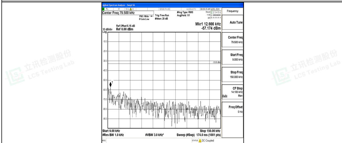
Band71_15MHz_16QAM_133197_1RB#0_0.009~0.15_0.009~0.15
