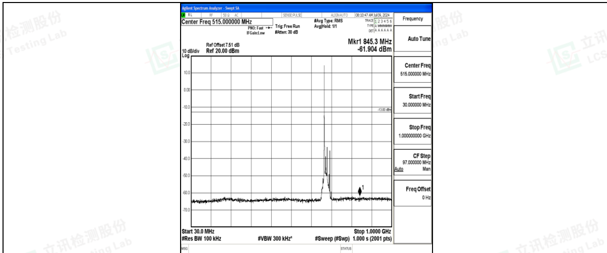
Band71_15MHz_QPSK_133297_1RB#0_30~1000_30~1000
