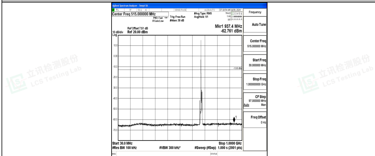
Band71_5MHz_16QAM_133297_1RB#0_30~1000_30~1000
