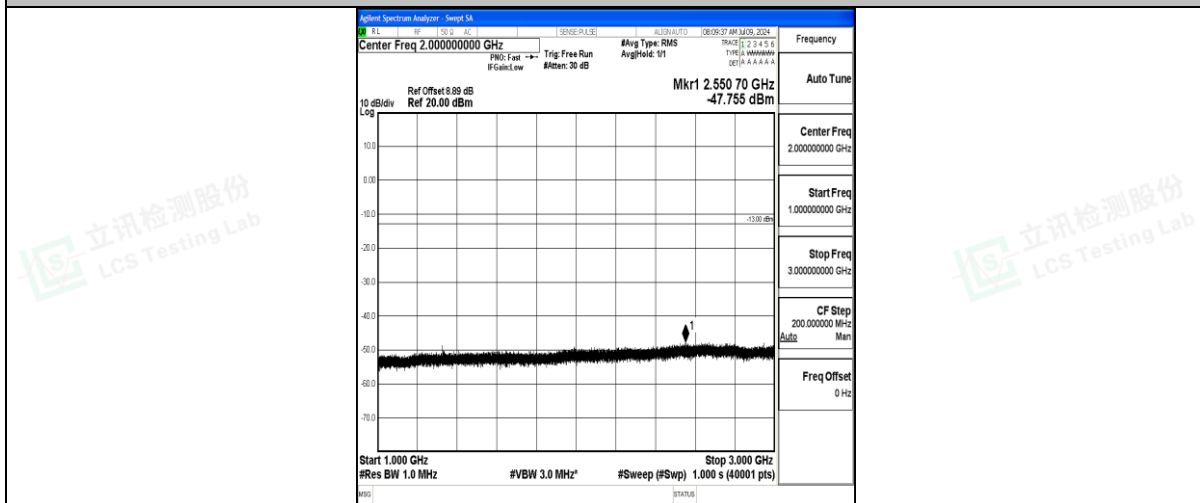
Band71_15MHz_16QAM_133197_1RB#0_1000~3000_1000~3000
