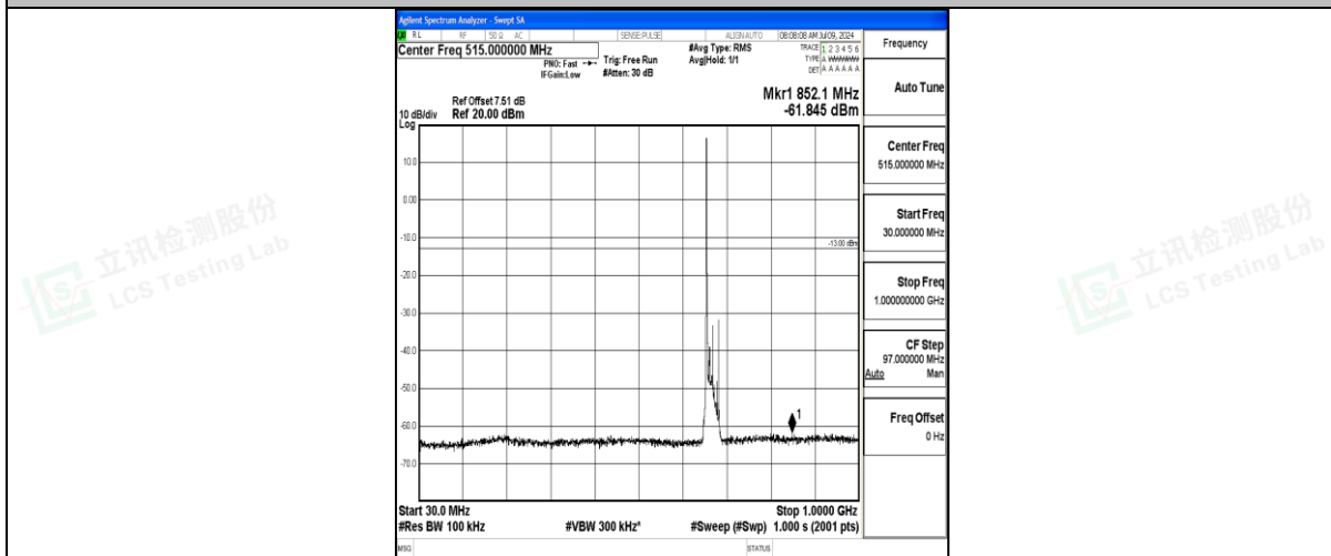
Band71_15MHz_QPSK_133197_1RB#0_30~1000_30~1000
