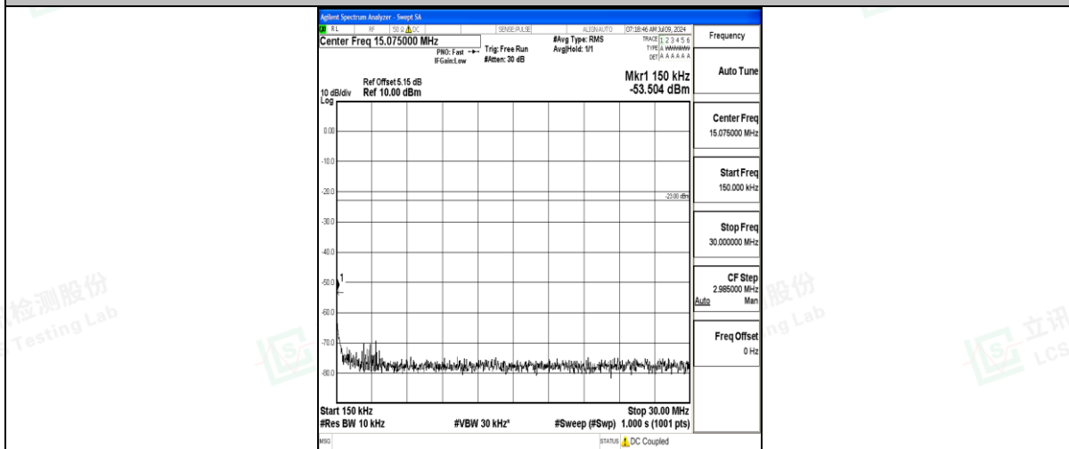
Band71_5MHz_16QAM_133297_1RB#0_0.15~30_0.15~30
