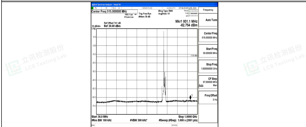
Band71_10MHz_16QAM_133297_1RB#0_30~1000_30~1000
