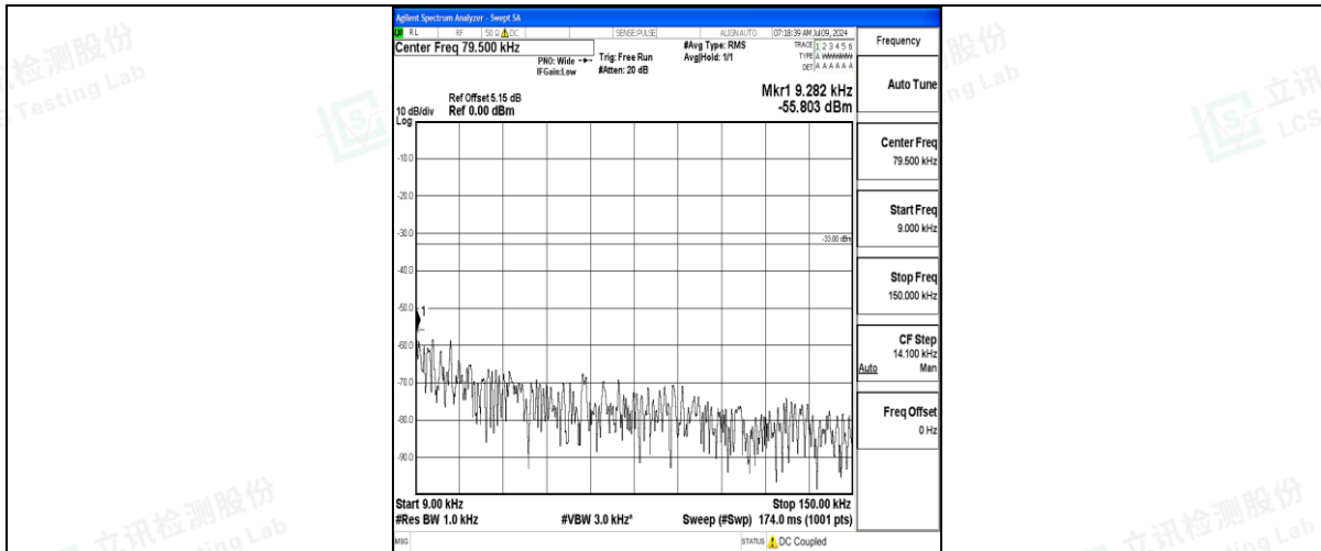
Band71_5MHz_16QAM_133297_1RB#0_0.009~0.15_0.009~0.15
