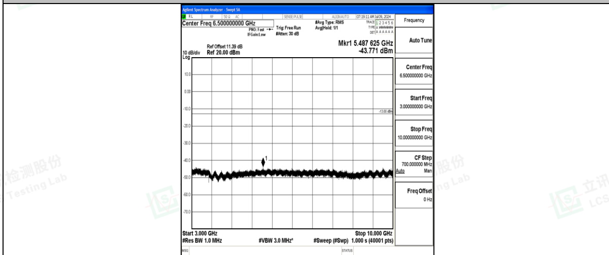
Band71_5MHz_16QAM_133297_1RB#0_3000~10000_3000~10000
