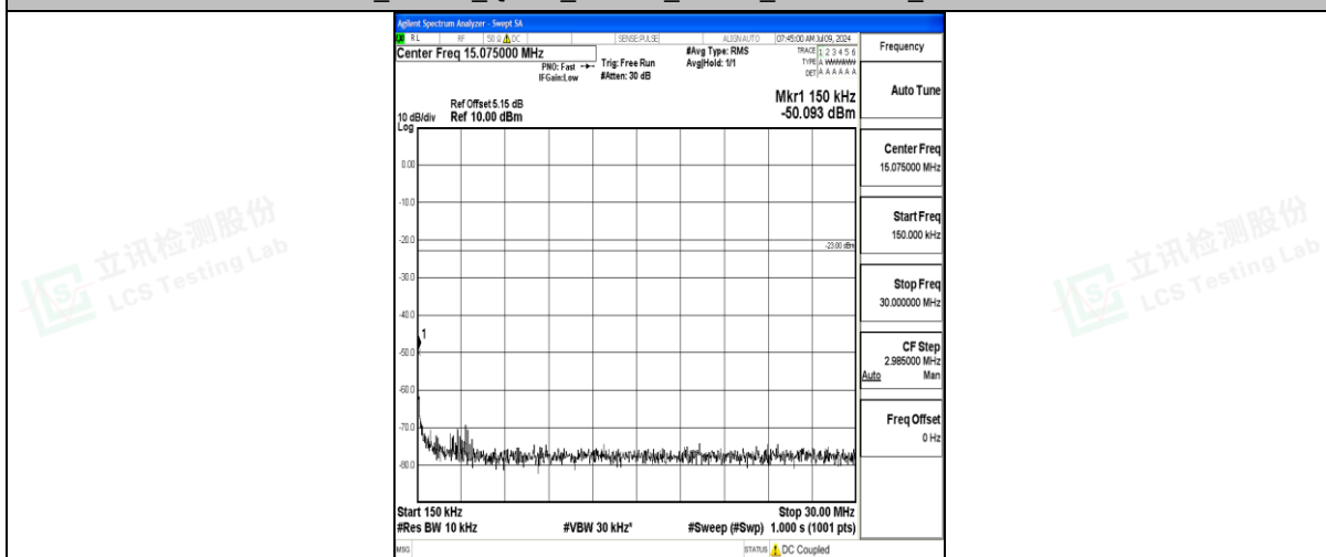
Band71_10MHz_QPSK_133297_1RB#0_0.15~30_0.15~30
