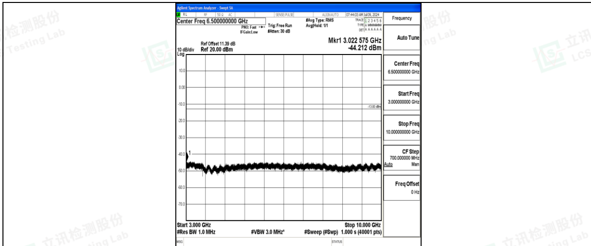
Band71_10MHz_16QAM_133172_1RB#0_3000~10000_3000~10000
