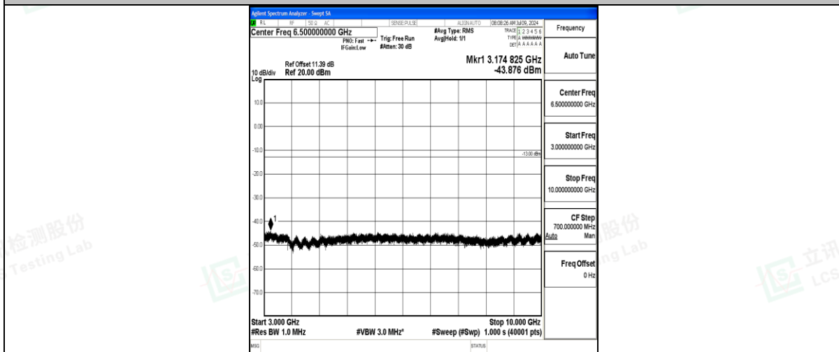
Band71_15MHz_QPSK_133197_1RB#0_3000~10000_3000~10000
