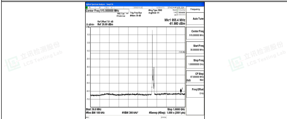
Band71_10MHz_QPSK_133172_1RB#0_30~1000_30~1000
