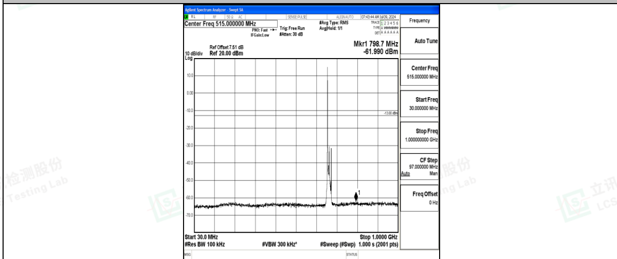
Band71_10MHz_16QAM_133172_1RB#0_30~1000_30~1000
