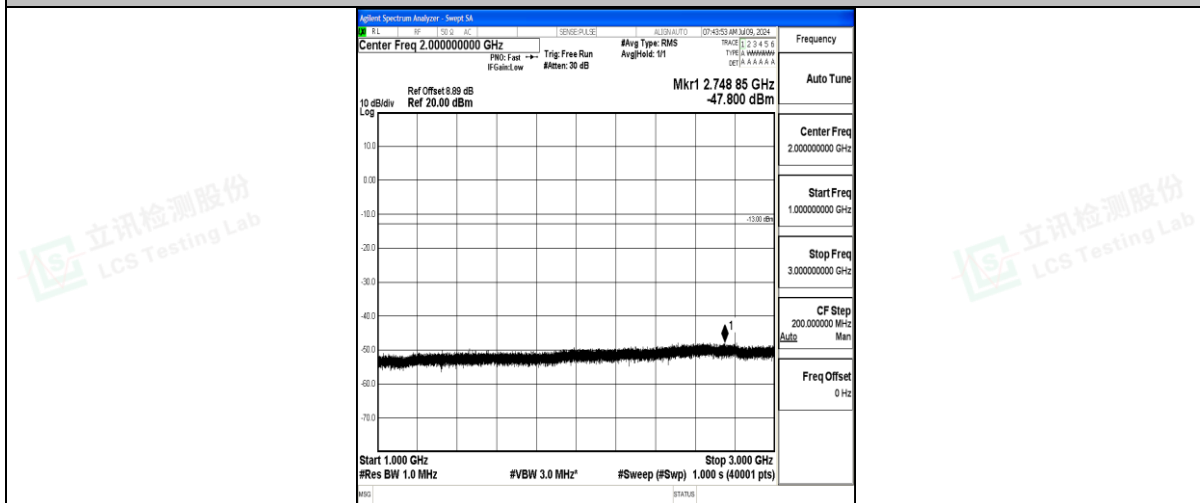
Band71_10MHz_16QAM_133172_1RB#0_1000~3000_1000~3000
