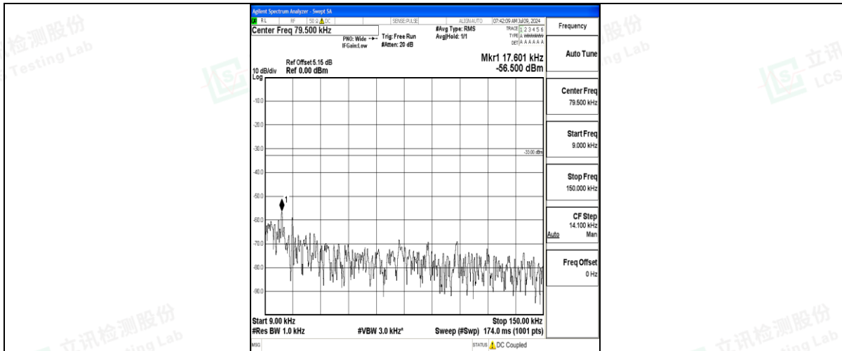
Band71_10MHz_QPSK_133172_1RB#0_0.009~0.15_0.009~0.15
