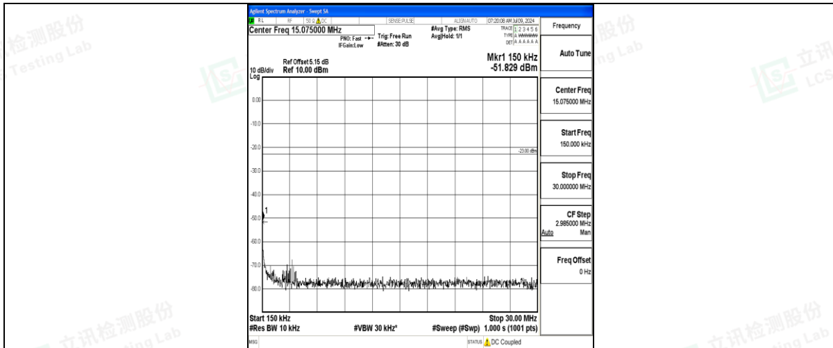
Band71_5MHz_QPSK_133447_1RB#0_0.15~30_0.15~30
