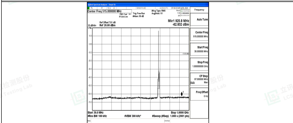
Band71_5MHz_QPSK_133447_1RB#0_30~1000_30~1000
