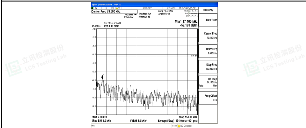
Band71_15MHz_QPSK_133397_1RB#0_0.009~0.15_0.009~0.15
