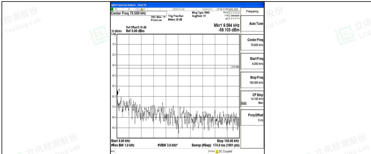
Band71_10MHz_16QAM_133297_1RB#0_0.009~0.15_0.009~0.15
