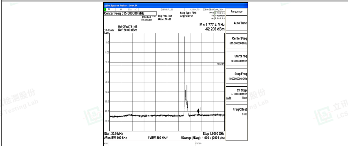
Band71_15MHz_16QAM_133197_1RB#0_30~1000_30~1000
