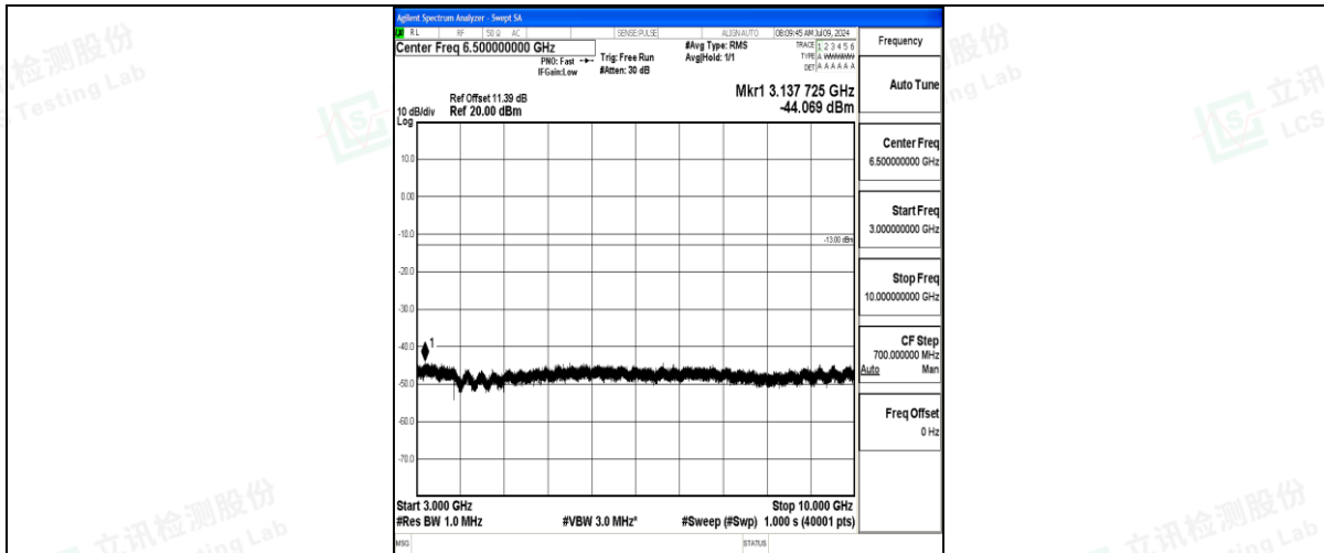
Band71_15MHz_16QAM_133197_1RB#0_3000~10000_3000~10000
