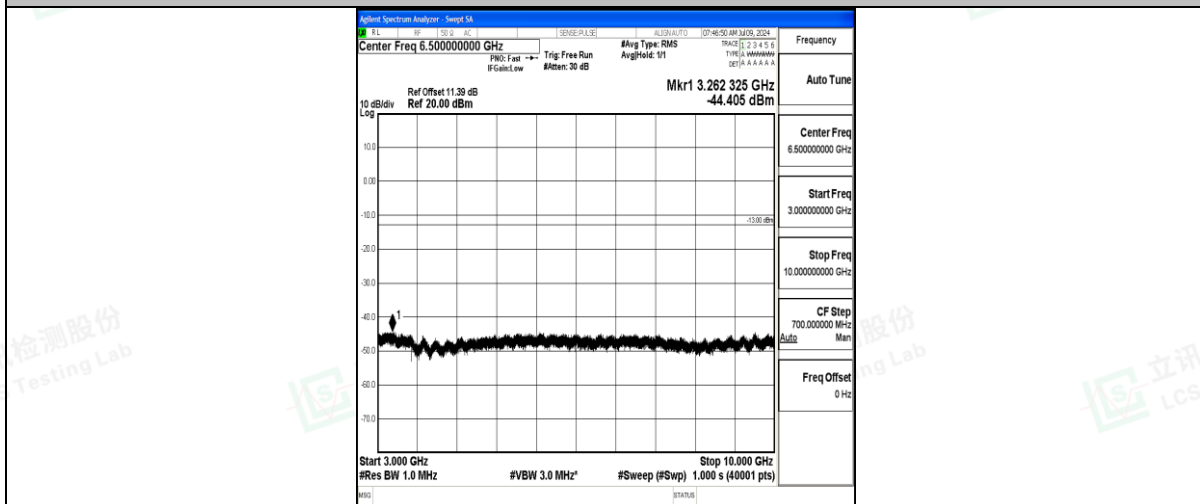
Band71_10MHz_16QAM_133297_1RB#0_3000~10000_3000~10000
