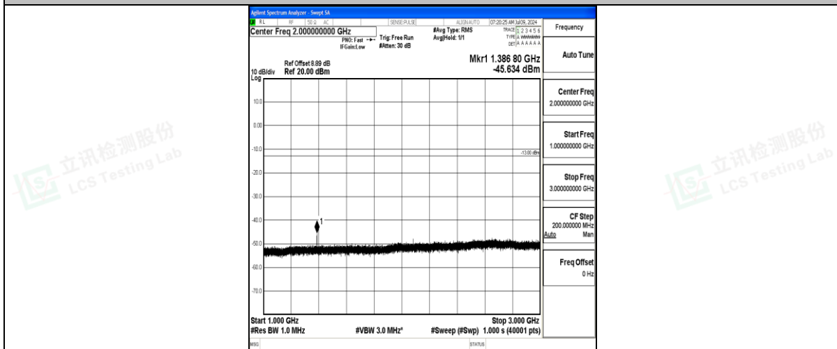
Band71_5MHz_QPSK_133447_1RB#0_1000~3000_1000~3000
