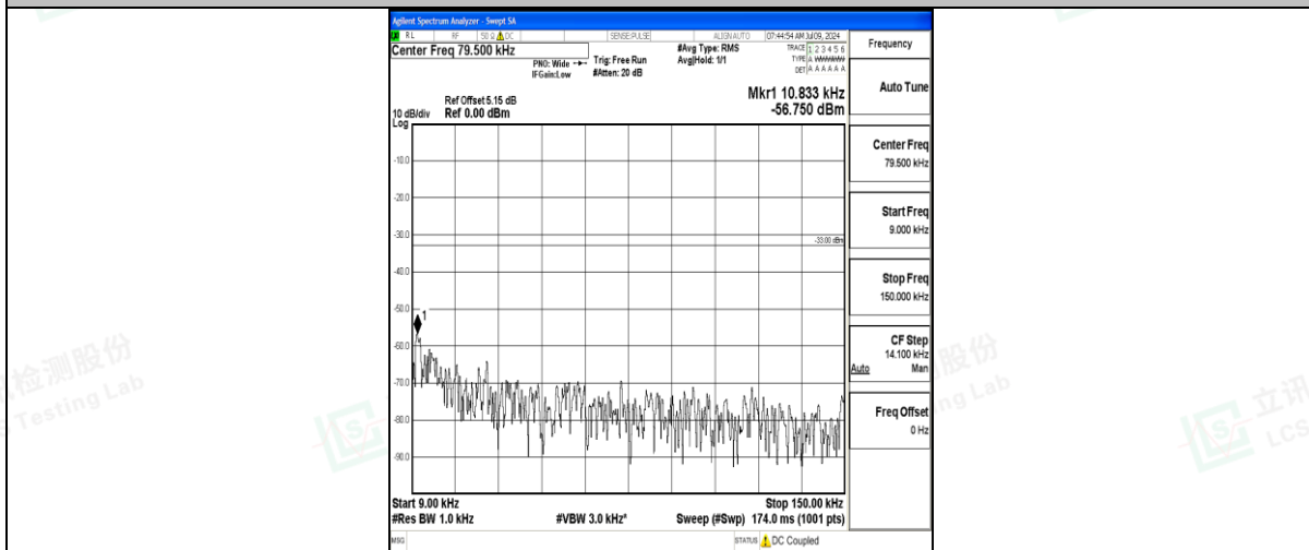
Band71_10MHz_QPSK_133297_1RB#0_0.009~0.15_0.009~0.15
