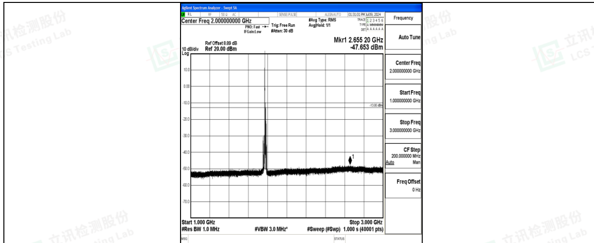
Band66_10MHz_16QAM_132622_1RB#0_1000~3000_1000~3000
