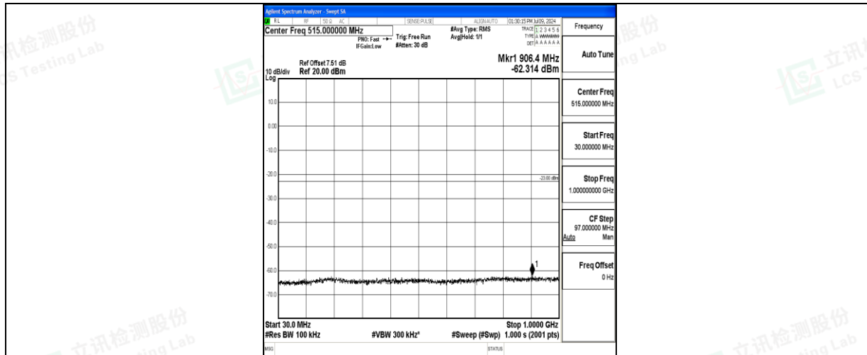
Band66_10MHz_QPSK_132622_1RB#0_30~1000_30~1000
