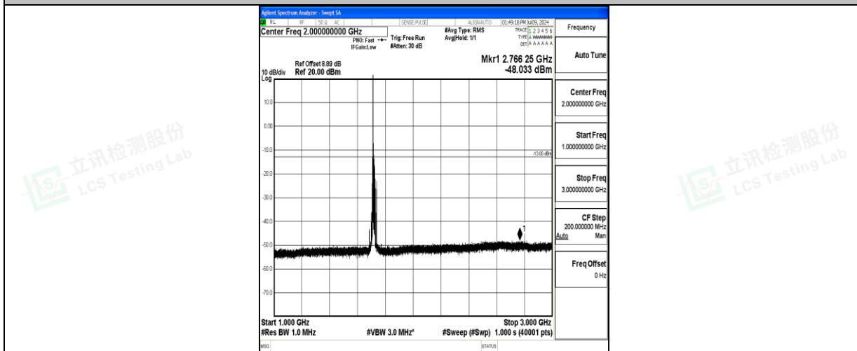
Band66_15MHz_QPSK_132047_1RB#0_1000~3000_1000~3000
