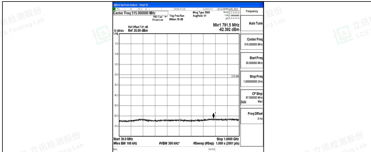
Band66_20MHz_QPSK_132572_1RB#0_30~1000_30~1000
