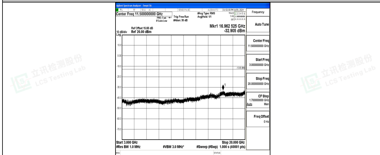
Band66_15MHz_QPSK_132597_1RB#0_3000~20000_3000~20000
