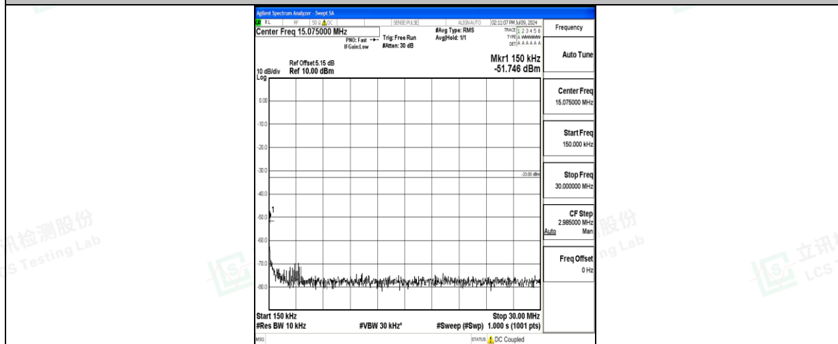
Band66_20MHz_QPSK_132322_1RB#0_0.15~30_0.15~30
