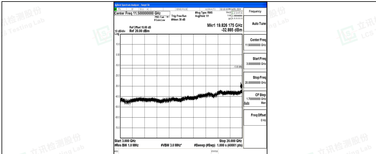
Band66_20MHz_QPSK_132072_1RB#0_3000~20000_3000~20000
