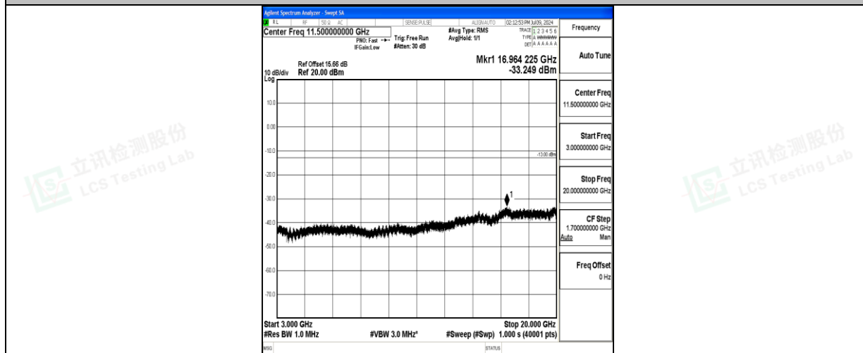
Band66_20MHz_QPSK_132572_1RB#0_3000~20000_3000~20000
