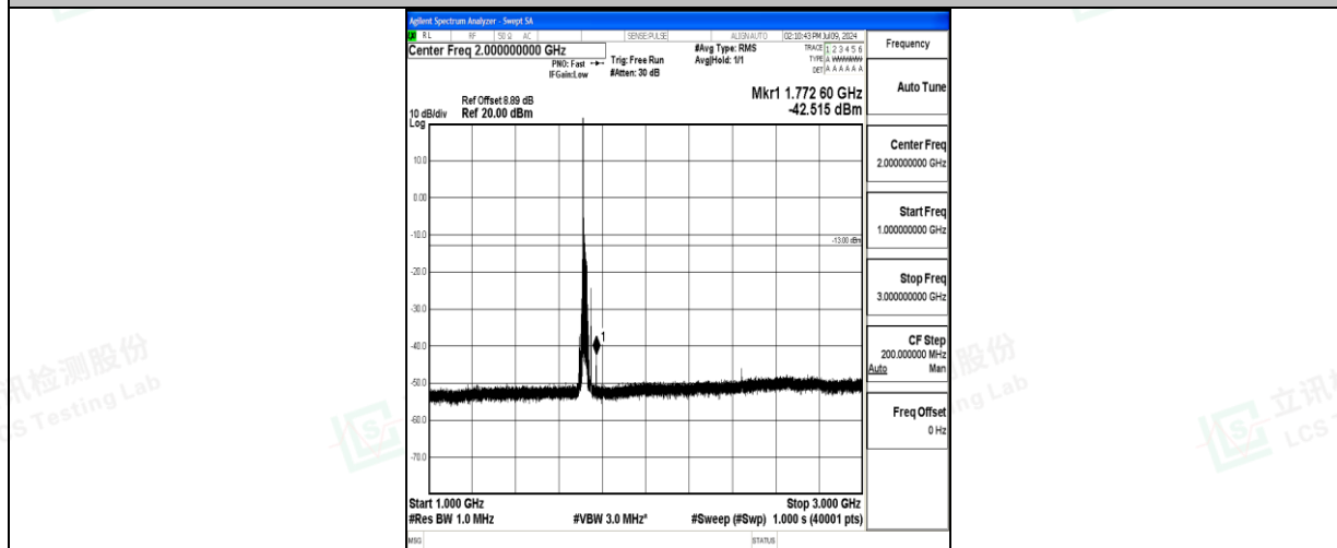
Band66_20MHz_16QAM_132072_1RB#0_1000~3000_1000~3000
