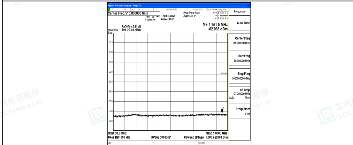
Band66_15MHz_16QAM_132322_1RB#0_30~1000_30~1000
