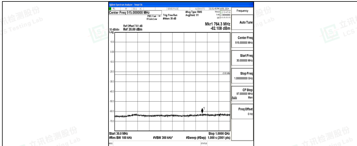
Band66_15MHz_QPSK_132597_1RB#0_30~1000_30~1000
