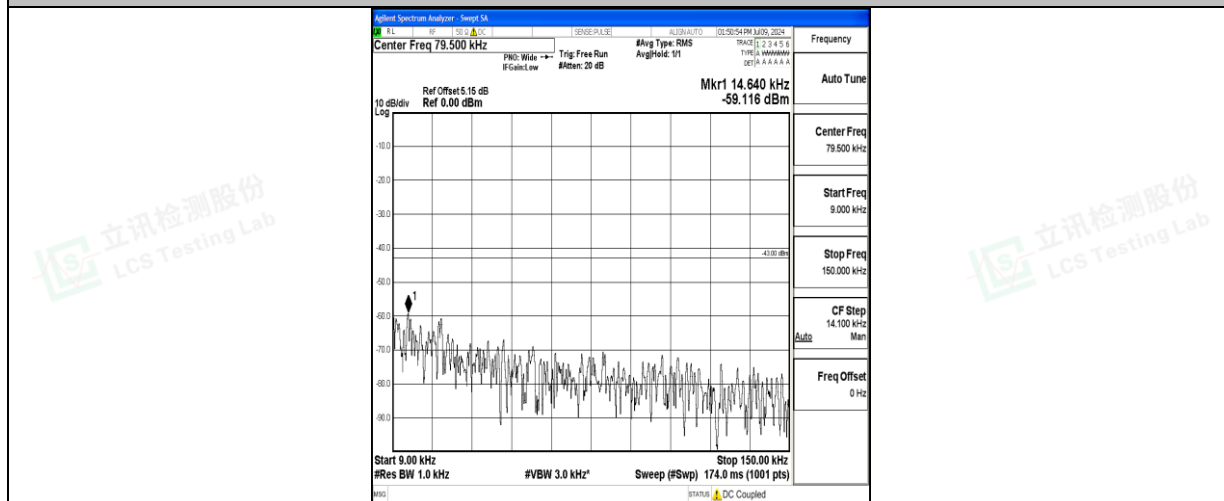
Band66_15MHz_16QAM_132322_1RB#0_0.009~0.15_0.009~0.15
