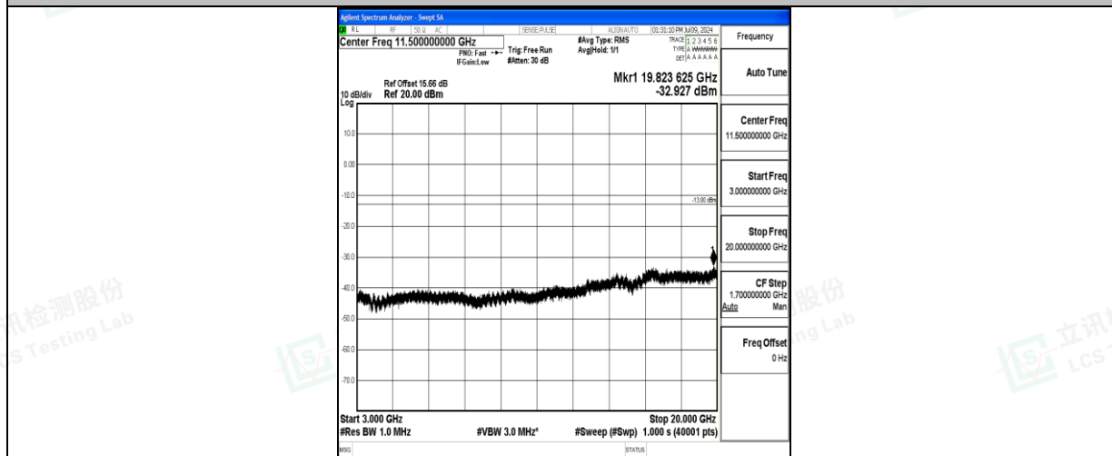
Band66_10MHz_16QAM_132622_1RB#0_3000~20000_3000~20000
