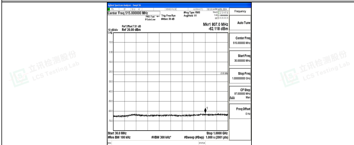
Band66_20MHz_16QAM_132572_1RB#0_30~1000_30~1000
