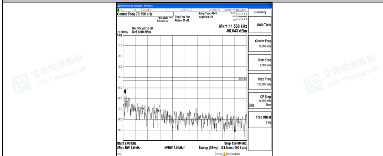
Band66_15MHz_QPSK_132047_1RB#0_0.009~0.15_0.009~0.15
