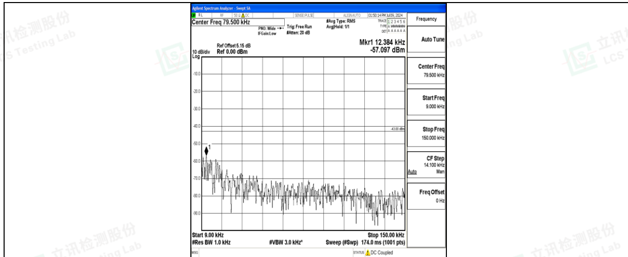
Band66_15MHz_QPSK_132322_1RB#0_0.009~0.15_0.009~0.15
