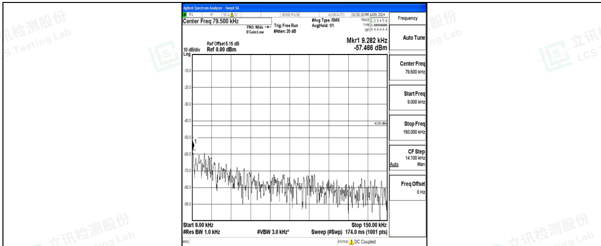
Band66_15MHz_16QAM_132597_1RB#0_0.009~0.15_0.009~0.15
