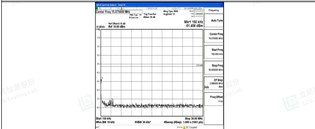
Band66_20MHz_16QAM_132572_1RB#0_0.15~30_0.15~30
