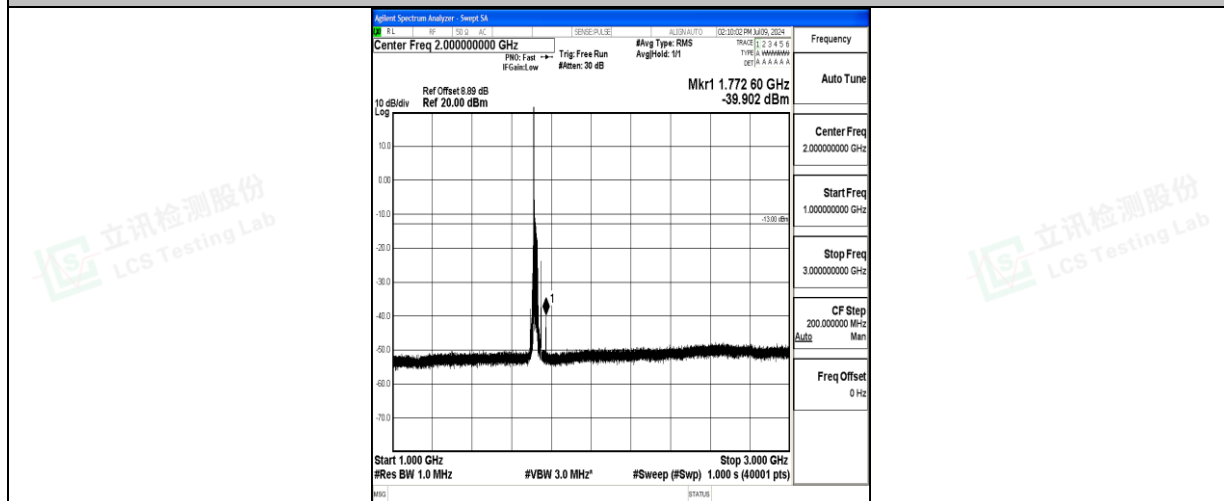
Band66_20MHz_QPSK_132072_1RB#0_1000~3000_1000~3000
