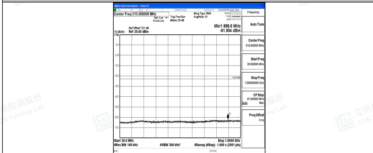
Band66_20MHz_QPSK_132072_1RB#0_30~1000_30~1000
