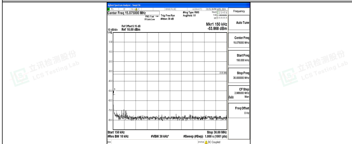
Band66_15MHz_QPSK_132597_1RB#0_0.15~30_0.15~30
