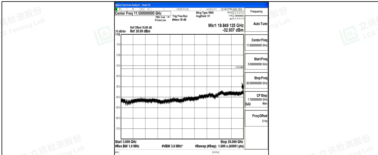
Band66_15MHz_QPSK_132047_1RB#0_3000~20000_3000~20000
