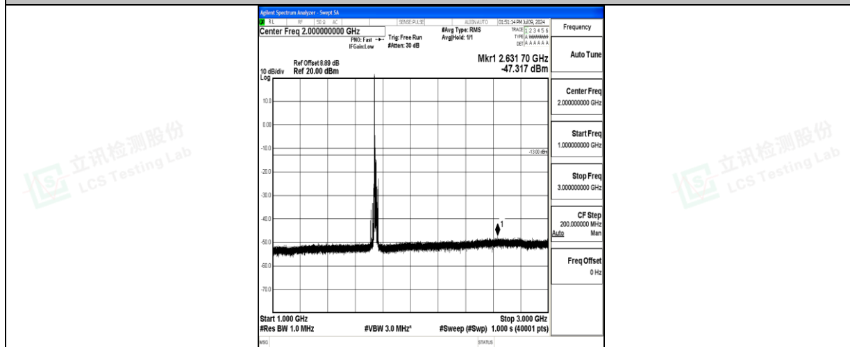
Band66_15MHz_16QAM_132322_1RB#0_1000~3000_1000~3000
