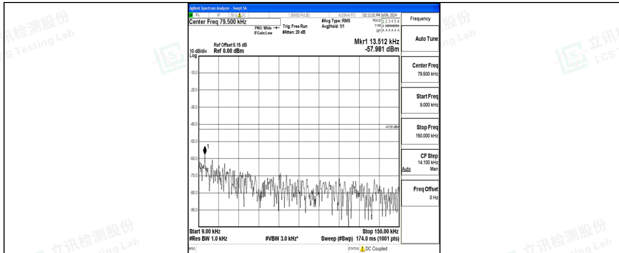
Band66_20MHz_QPSK_132322_1RB#0_0.009~0.15_0.009~0.15
