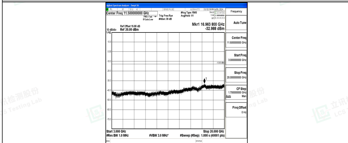
Band66_15MHz_16QAM_132597_1RB#0_3000~20000_3000~20000
