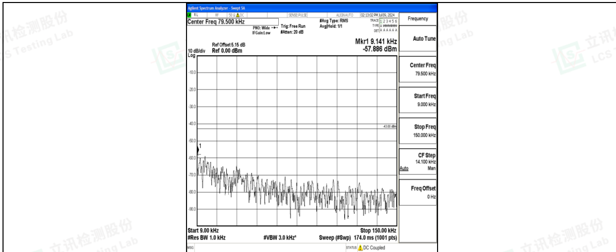
Band66_20MHz_16QAM_132572_1RB#0_0.009~0.15_0.009~0.15
