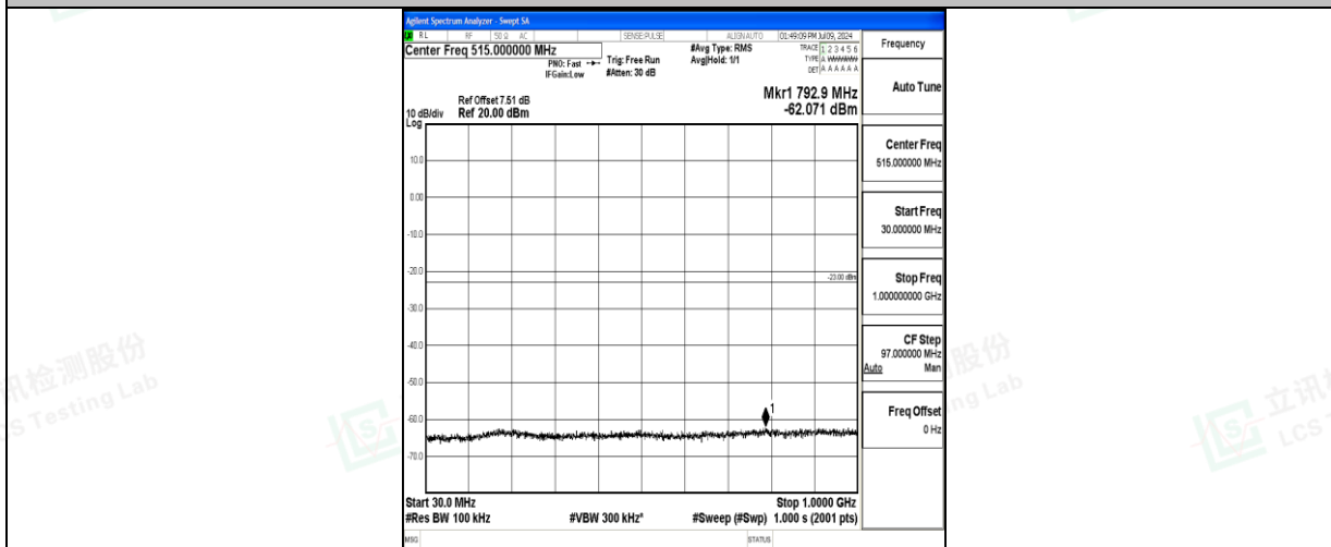
Band66_15MHz_QPSK_132047_1RB#0_30~1000_30~1000
