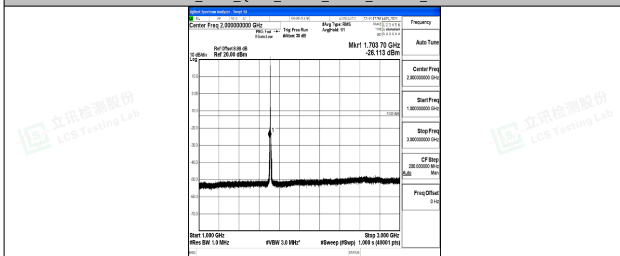
Band66 3MHz QPSK 131987 1RB#0 1000~3000 1000~3000
