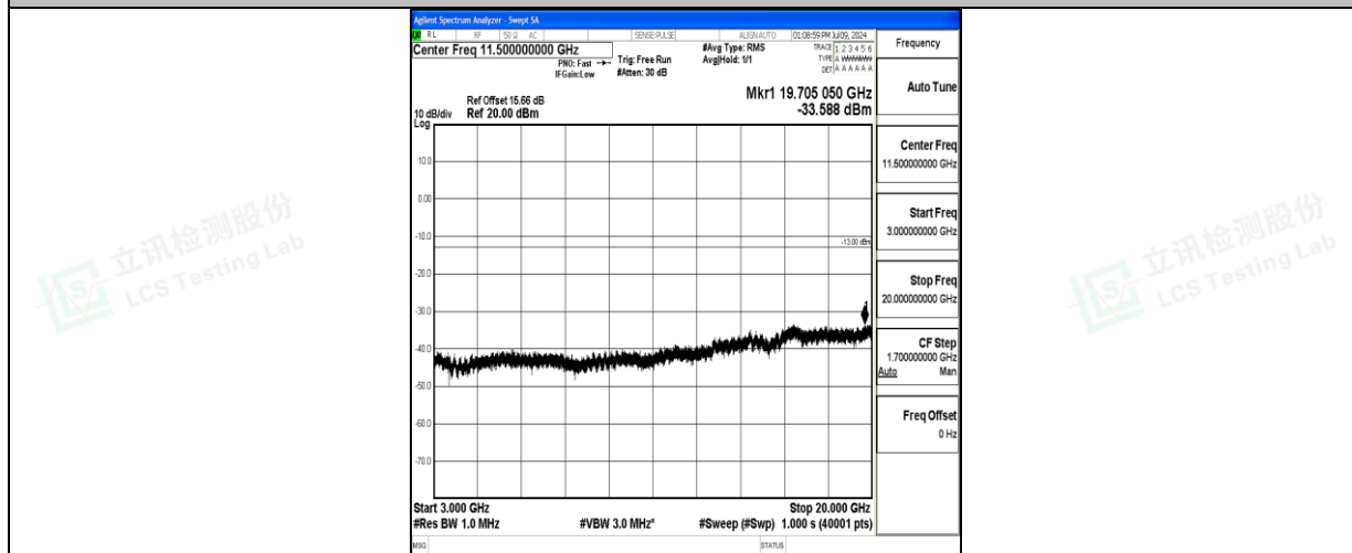
Band66_5MHz_QPSK_132647_1RB#0_3000~20000_3000~20000
