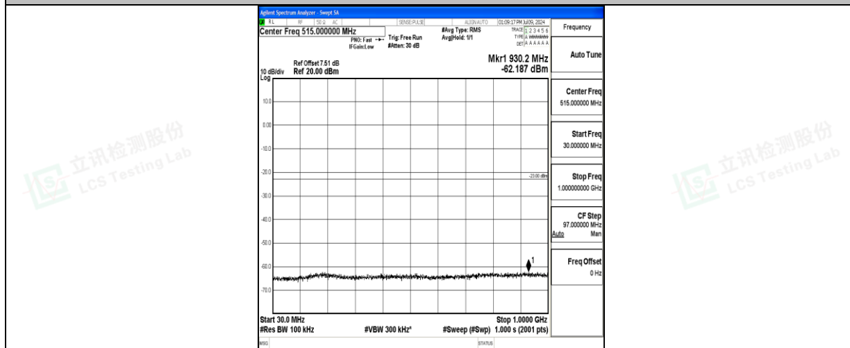
Band66_5MHz_16QAM_132647_1RB#0_30~1000_30~1000
