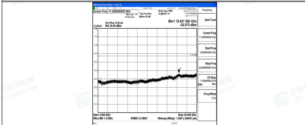
Band66_1.4MHz_QPSK_132322_1RB#0_3000~20000_3000~20000
