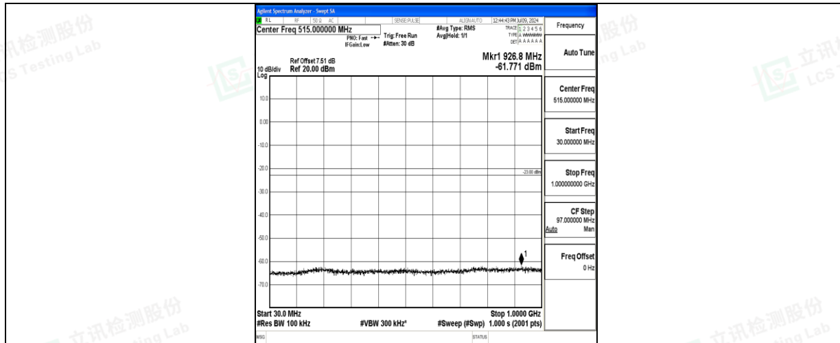
Band66_3MHz_16QAM_131987_1RB#0_30~1000_30~1000
