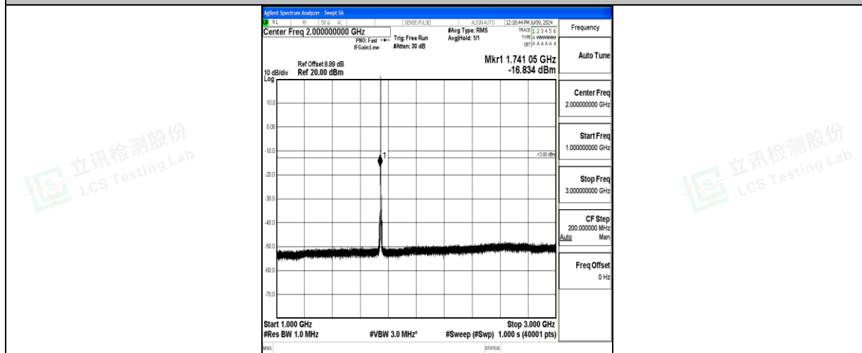
Band66_1.4MHz_16QAM_132322_1RB#0_1000~3000_1000~3000
