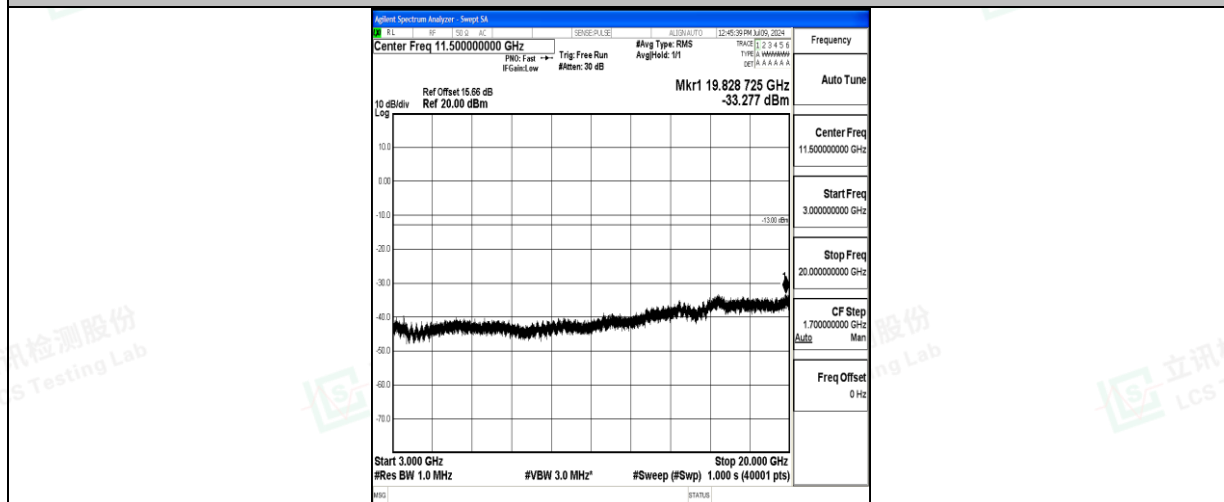
Band66_3MHz_QPSK_132322_1RB#0_3000~20000_3000~20000
