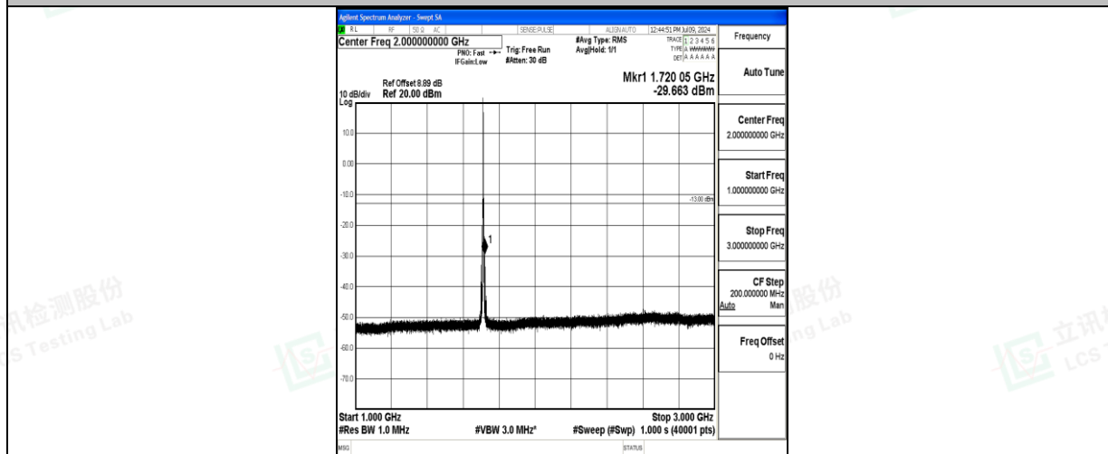
Band66_3MHz_16QAM_131987_1RB#0_1000~3000_1000~3000
