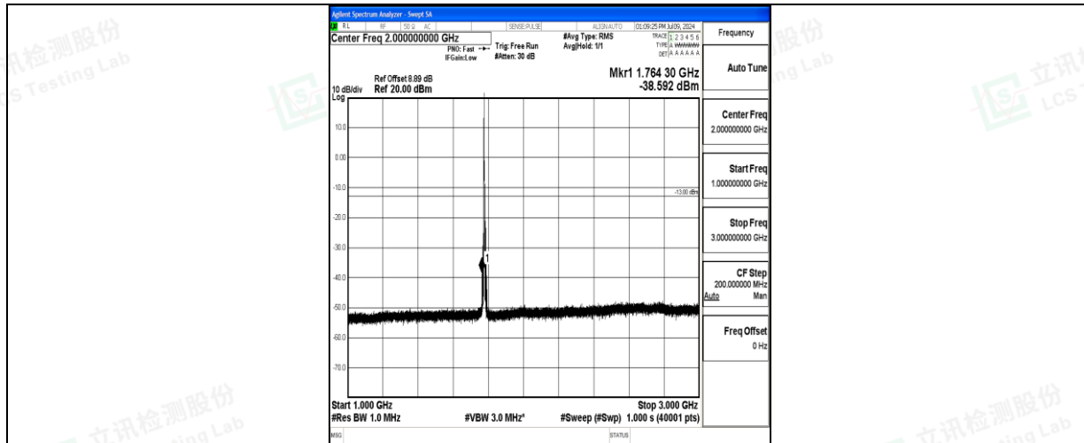
Band66_5MHz_16QAM_132647_1RB#0_1000~3000_1000~3000
