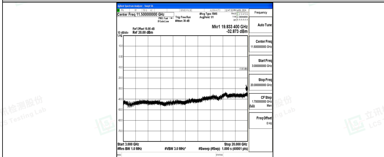
Band66_3MHz_16QAM_132657_1RB#0_3000~20000_3000~20000
