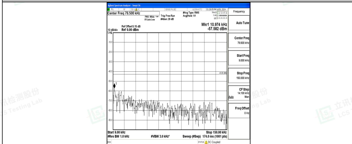
Band66_10MHz_16QAM_132022_1RB#0_0.009~0.15_0.009~0.15
