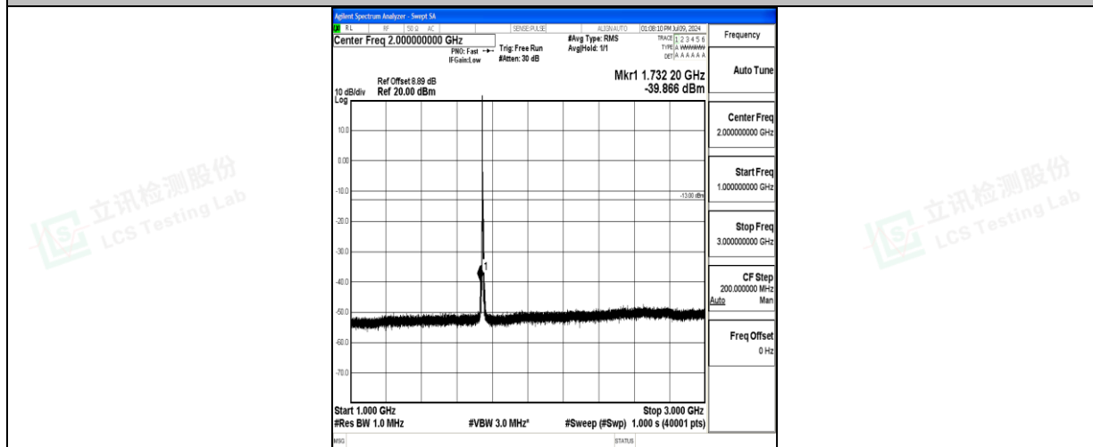
Band66_5MHz_16QAM_132322_1RB#0_1000~3000_1000~3000
