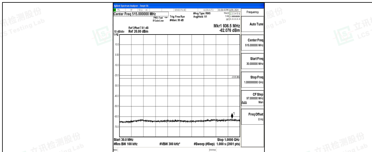
Band66_5MHz_16QAM_131997_1RB#0_30~1000_30~1000
