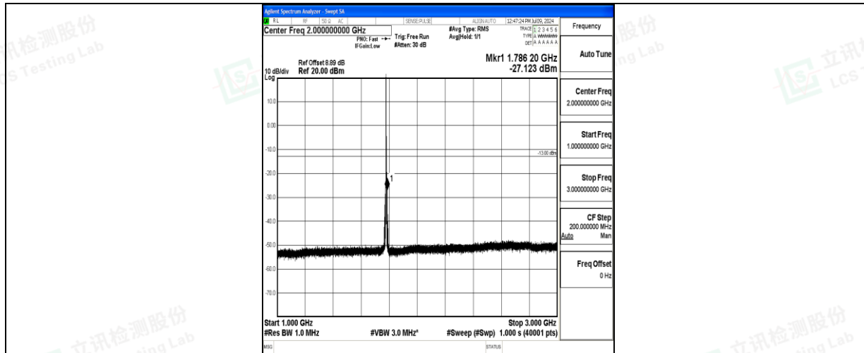
Band66_3MHz_16QAM_132657_1RB#0_1000~3000_1000~3000
