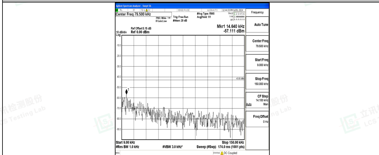
Band66_3MHz_16QAM_131987_1RB#0_0.009~0.15_0.009~0.15
