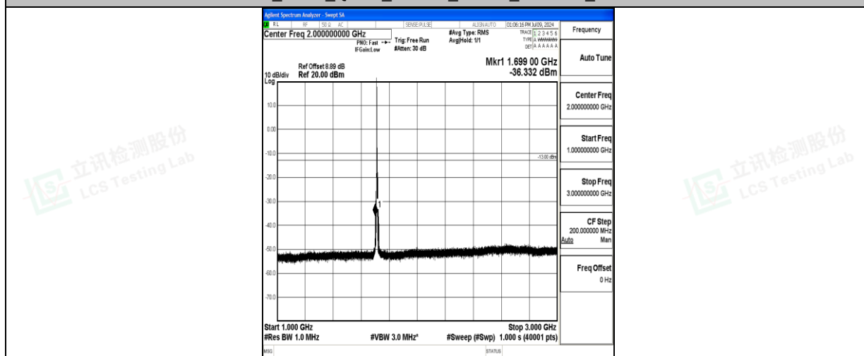
Band66_5MHz_QPSK_131997_1RB#0_1000~3000_1000~3000
