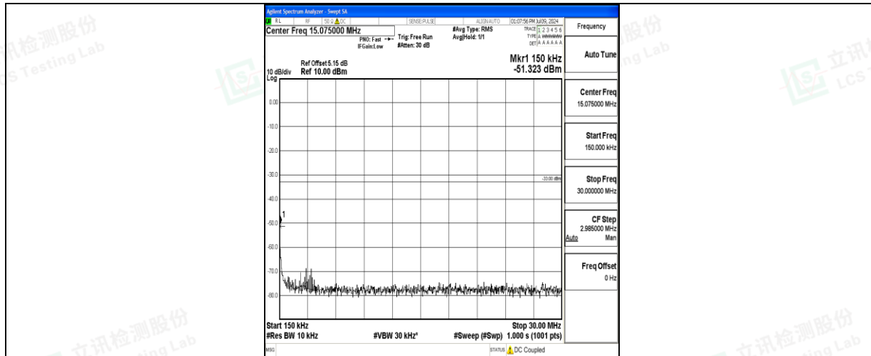
Band66_5MHz_16QAM_132322_1RB#0_0.15~30_0.15~30
