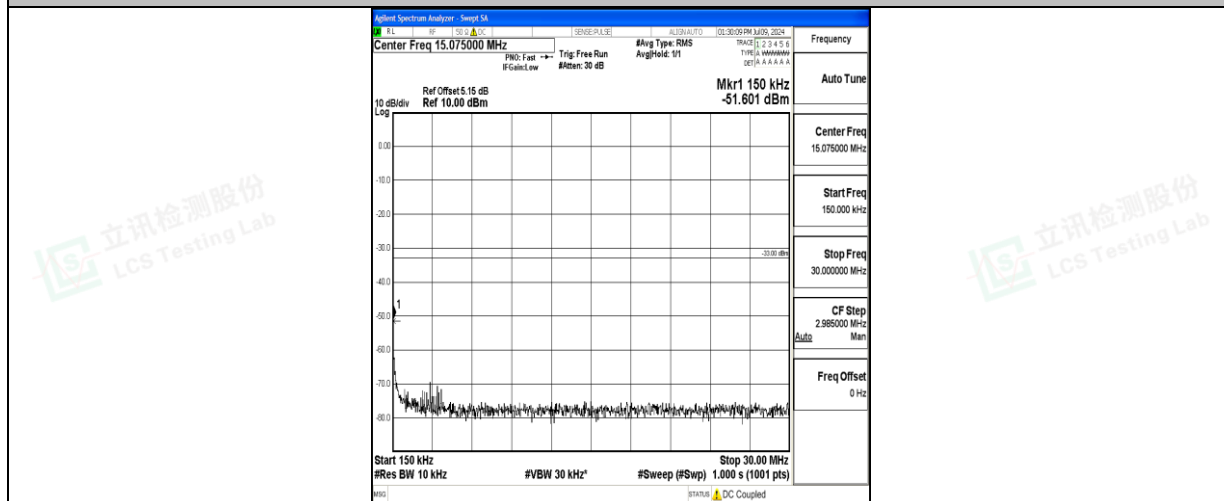
Band66_10MHz_QPSK_132622_1RB#0_0.15~30_0.15~30
