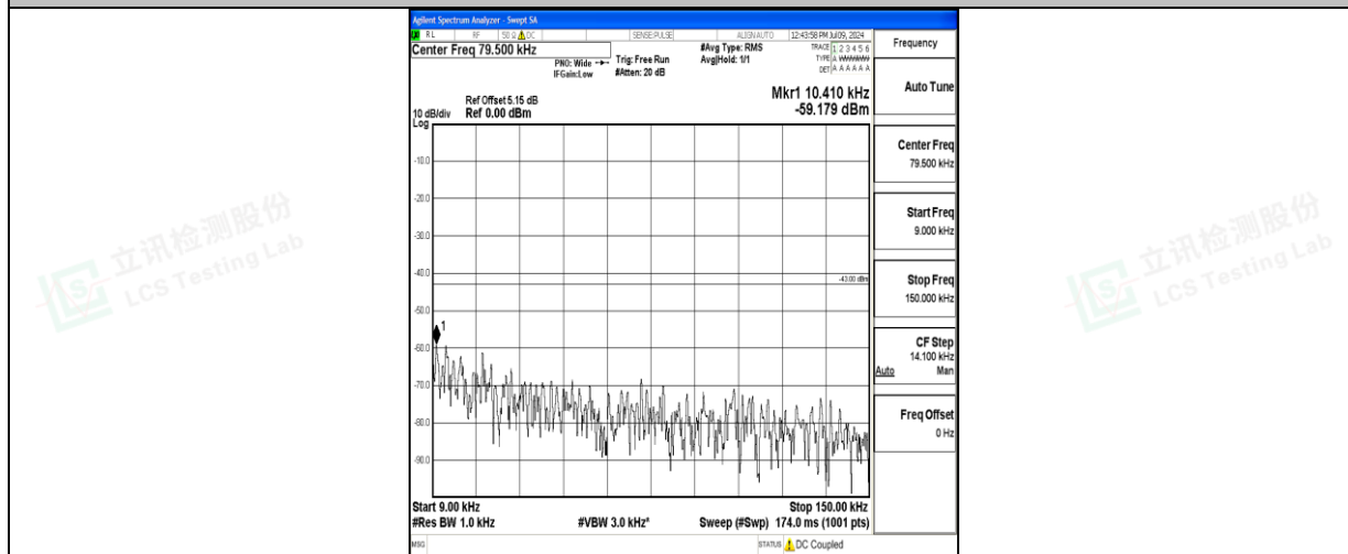
Band66_3MHz_QPSK_131987_1RB#0_0.009~0.15_0.009~0.15
