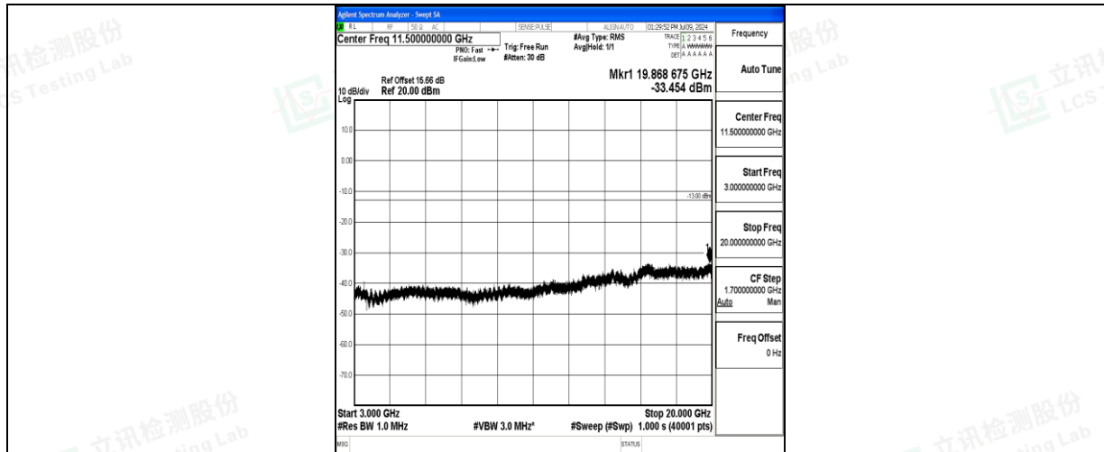
Band66_10MHz_16QAM_132322_1RB#0_3000~20000_3000~20000
