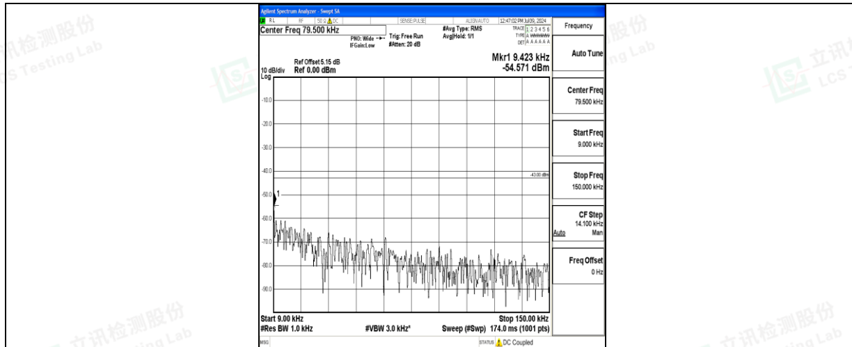
Band66_3MHz_16QAM_132657_1RB#0_0.009~0.15_0.009~0.15
