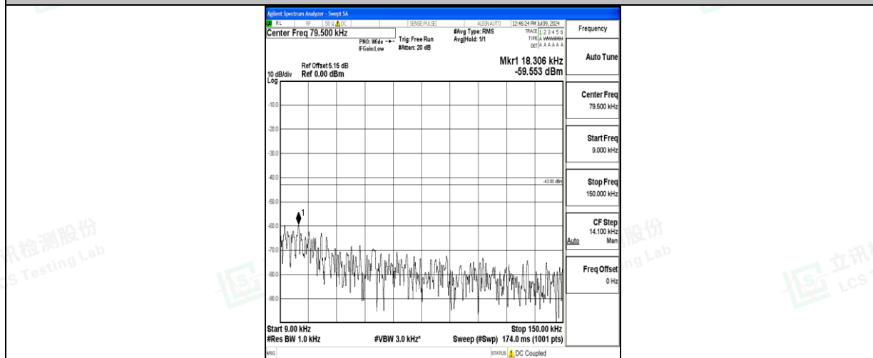
Band66_3MHz_QPSK_132657_1RB#0_0.009~0.15_0.009~0.15
