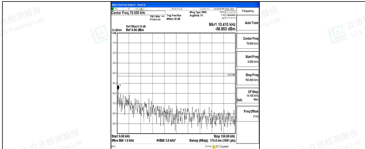
Band66_5MHz_16QAM_132647_1RB#0_0.009~0.15_0.009~0.15
