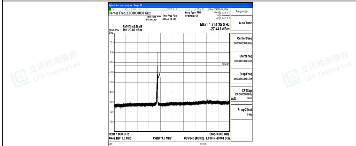
Band66_3MHz_16QAM_132322_1RB#0_1000~3000_1000~3000
