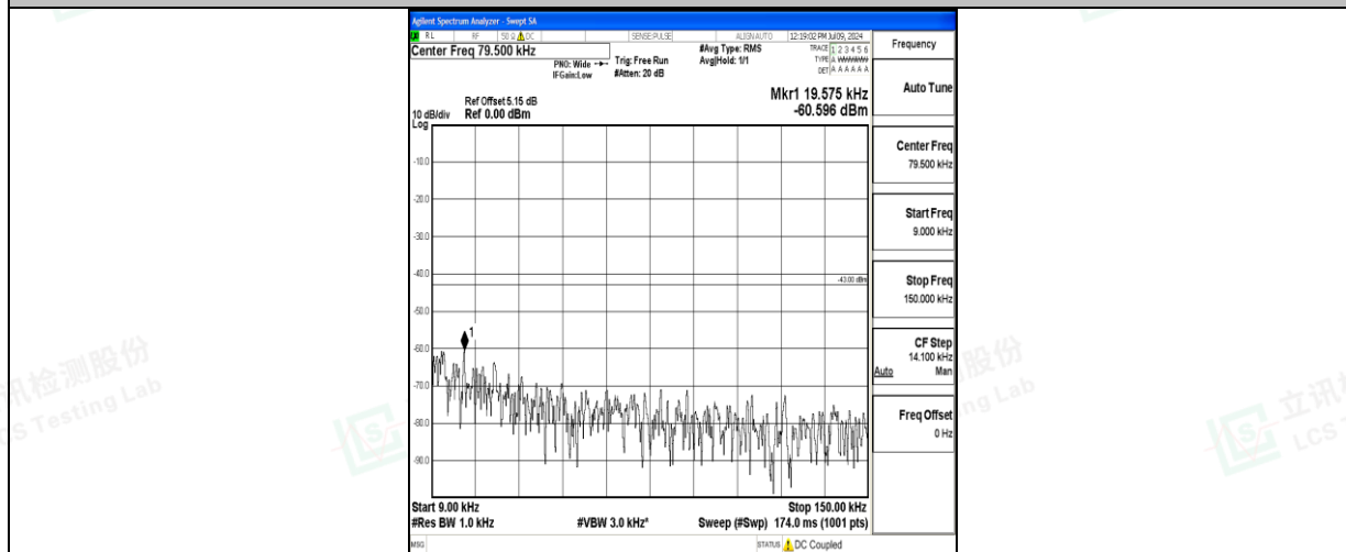
Band66_1.4MHz_QPSK_132665_1RB#0_0.009~0.15_0.009~0.15
