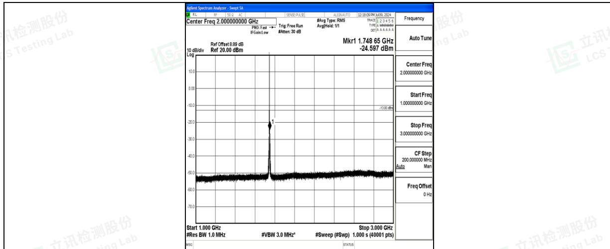
Band66_1.4MHz_QPSK_132322_1RB#0_1000~3000_1000~3000
