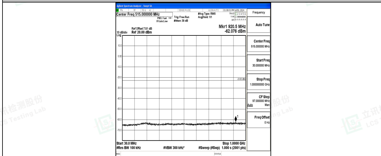
Band66_5MHz_16QAM_132322_1RB#0_30~1000_30~1000
