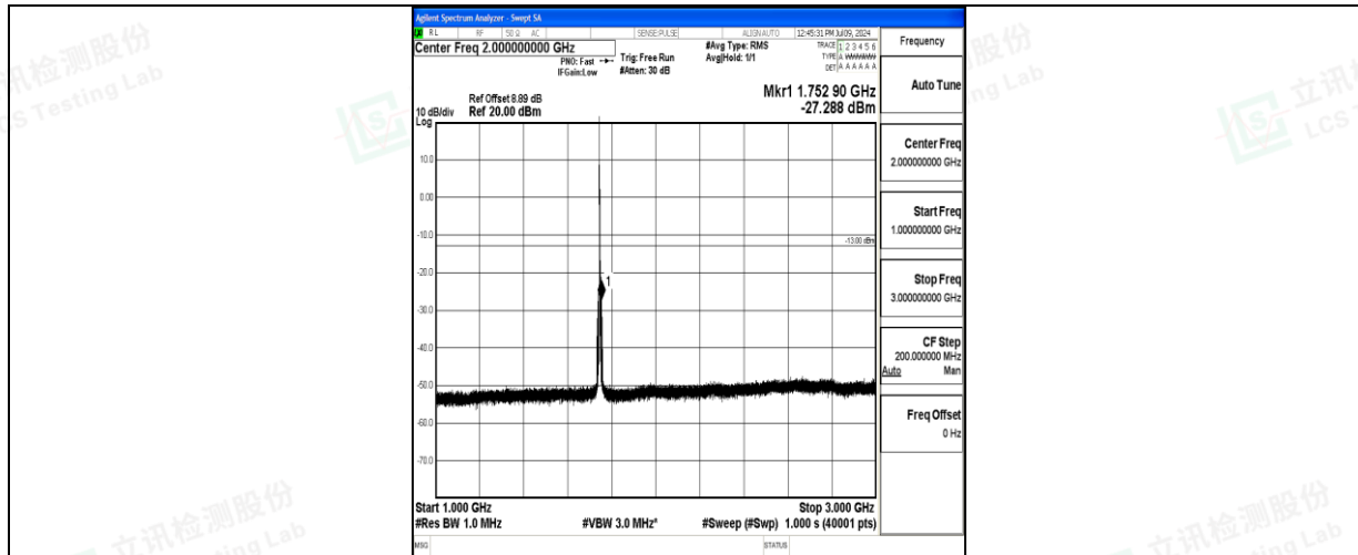
Band66_3MHz_QPSK_132322_1RB#0_1000~3000_1000~3000
