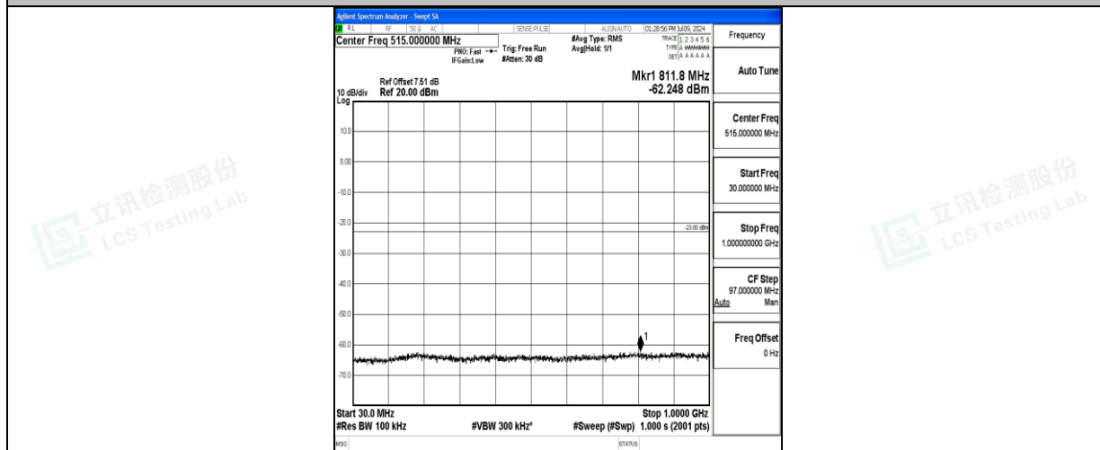
Band66_10MHz_QPSK_132322_1RB#0_30~1000_30~1000
