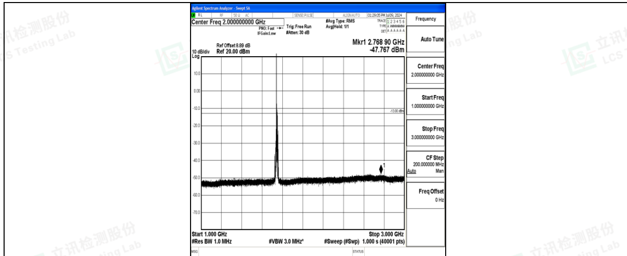
Band66_10MHz_QPSK_132322_1RB#0_1000~3000_1000~3000
