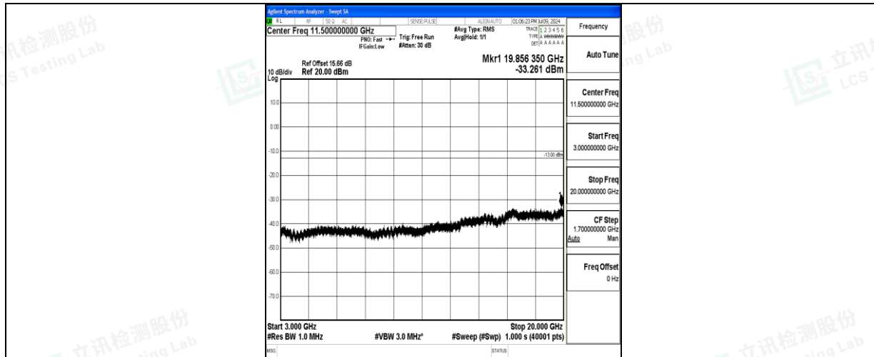
Band66_5MHz_QPSK_131997_1RB#0_3000~20000_3000~20000
