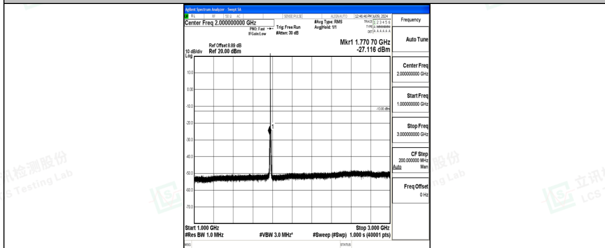
Band66_3MHz_QPSK_132657_1RB#0_1000~3000_1000~3000
