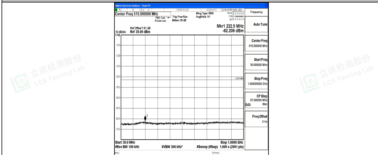
Band66_3MHz_QPSK_132322_1RB#0_30~1000_30~1000
