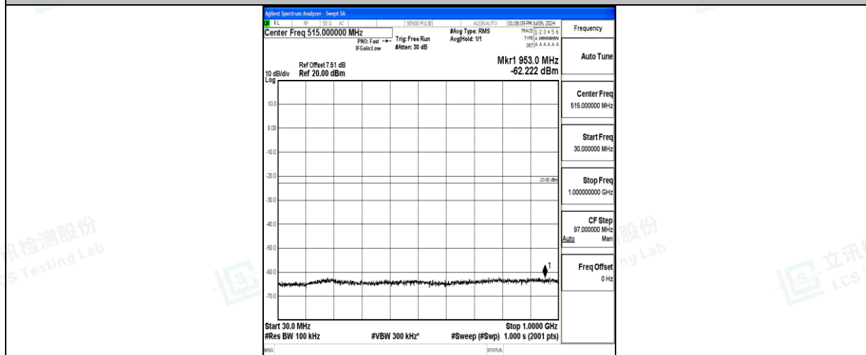
Band66_5MHz_QPSK_131997_1RB#0_30~1000_30~1000
