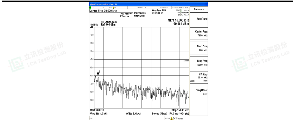
Band66_10MHz_16QAM_132322_1RB#0_0.009~0.15_0.009~0.15
