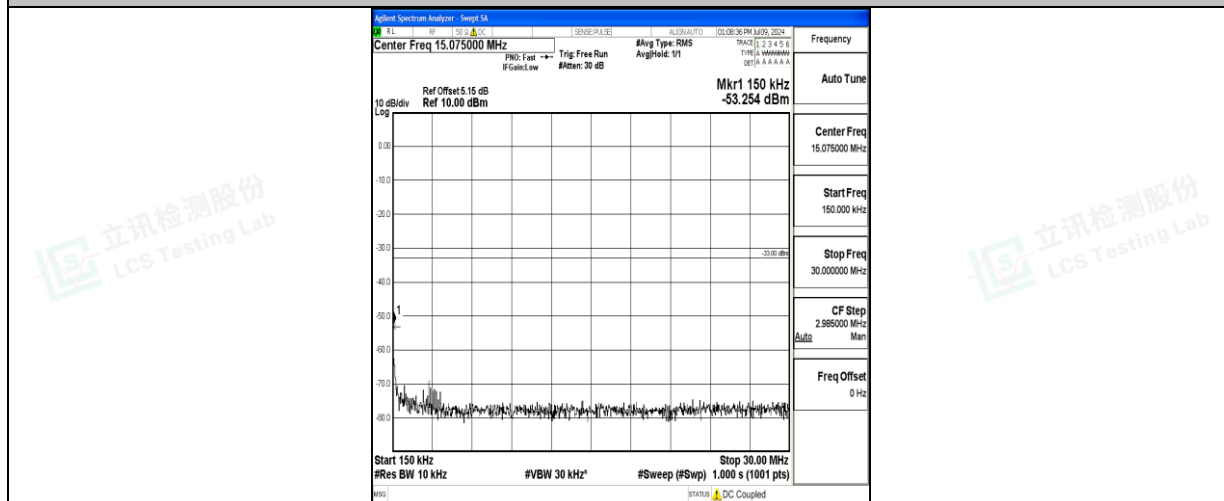
Band66_5MHz_QPSK_132647_1RB#0_0.15~30_0.15~30
