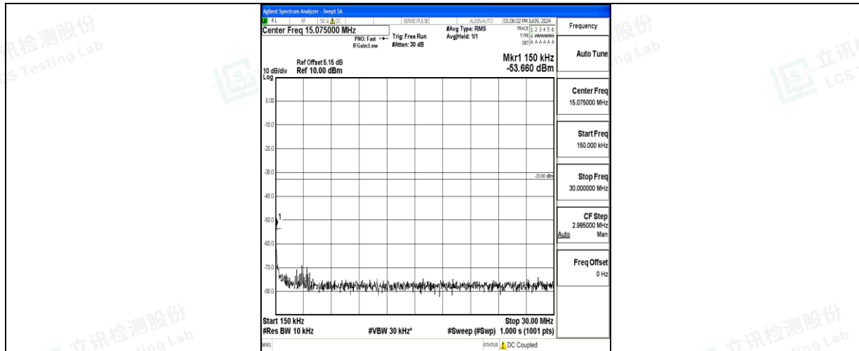
Band66_5MHz_QPSK_131997_1RB#0_0.15~30_0.15~30
