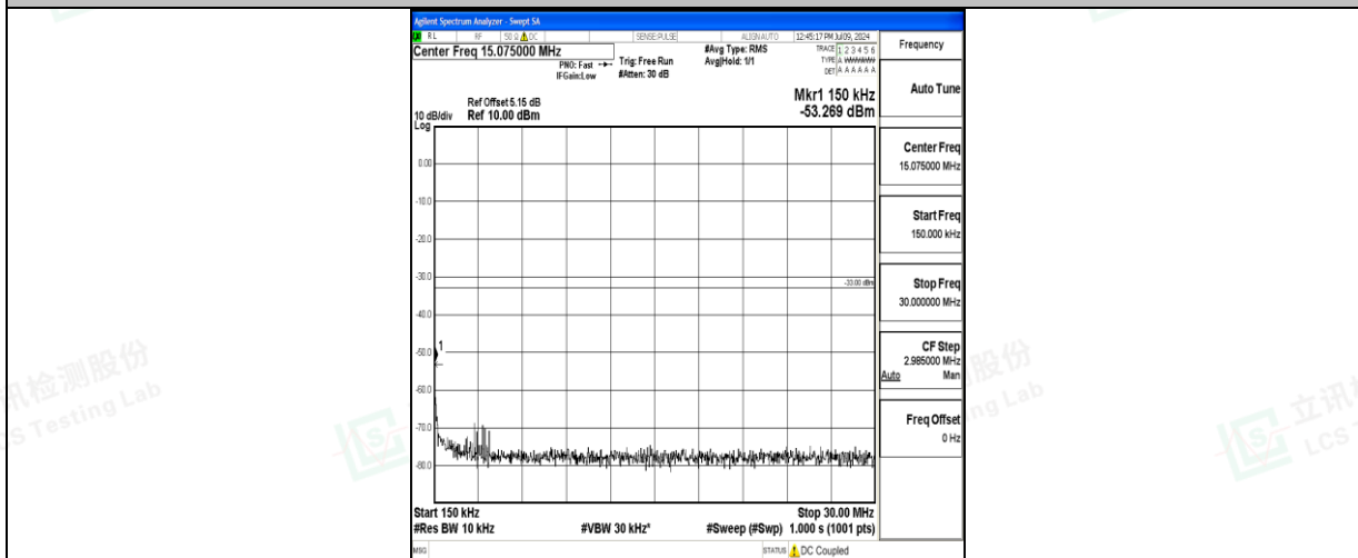
Band66_3MHz_QPSK_132322_1RB#0_0.15~30_0.15~30
