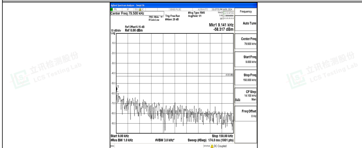
Band66_5MHz_16QAM_132322_1RB#0_0.009~0.15_0.009~0.15
