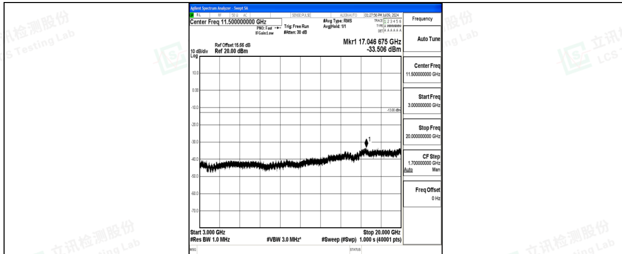
Band66_10MHz_QPSK_132022_1RB#0_3000~20000_3000~20000
