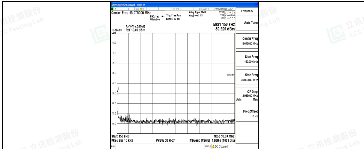
Band66_3MHz_16QAM_132322_1RB#0_0.15~30_0.15~30
