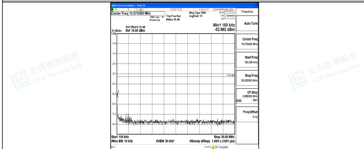
Band66_3MHz_16QAM_131987_1RB#0_0.15~30_0.15~30
