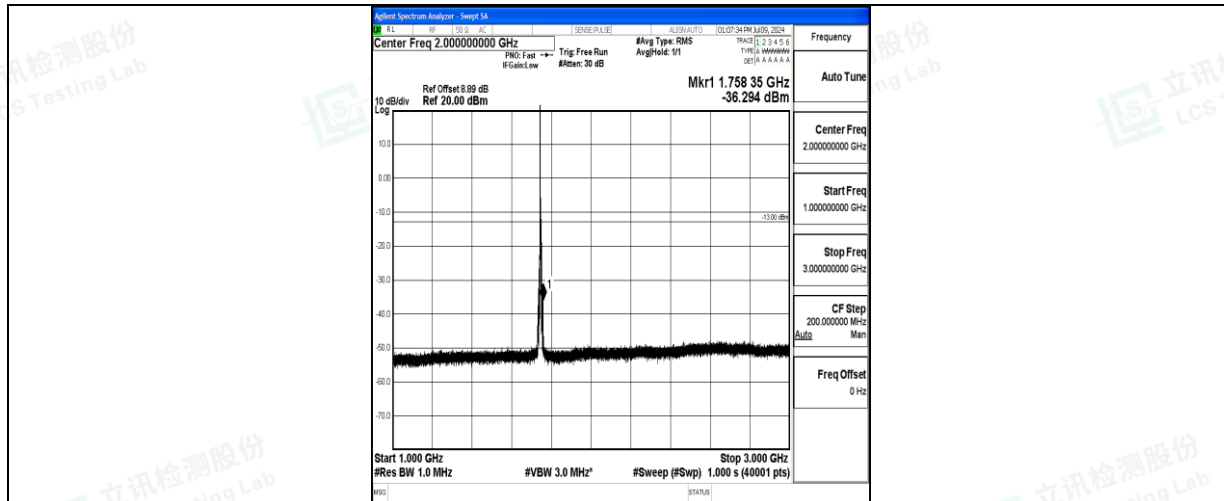
Band66_5MHz_QPSK_132322_1RB#0_1000~3000_1000~3000
