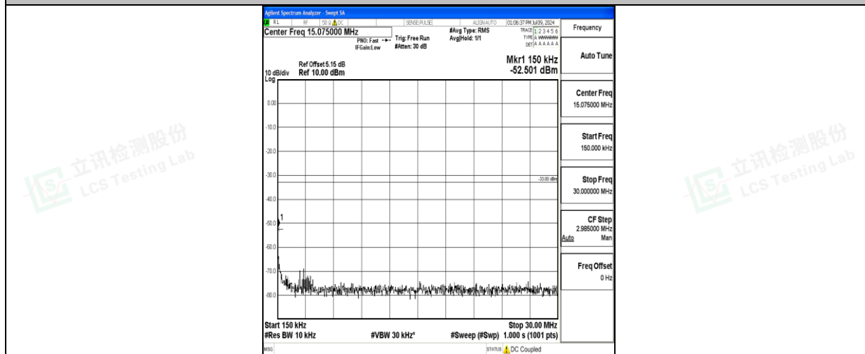
Band66_5MHz_16QAM_131997_1RB#0_0.15~30_0.15~30
