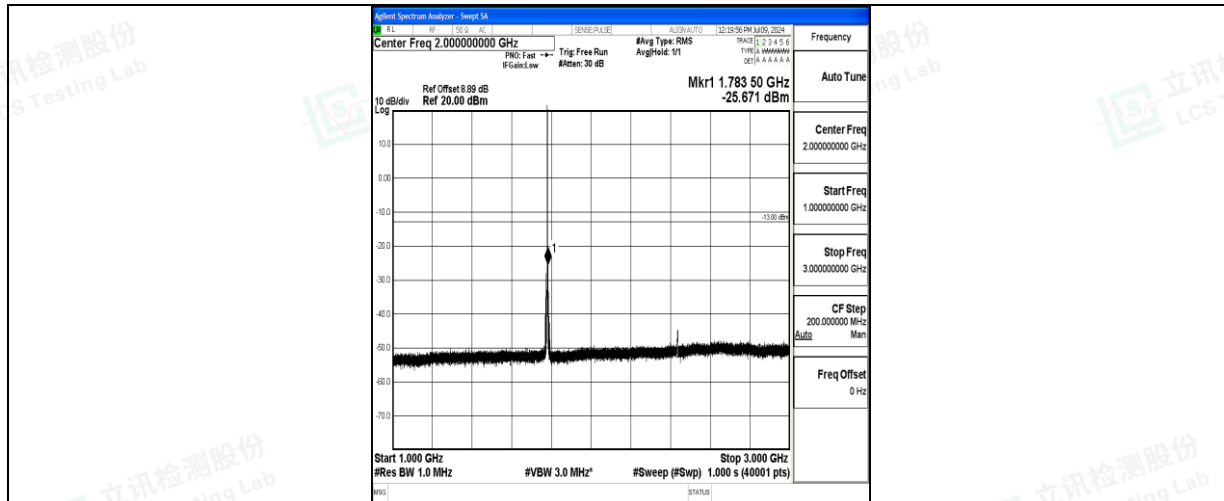
Band66_1.4MHz_16QAM_132665_1RB#0_1000~3000_1000~3000
