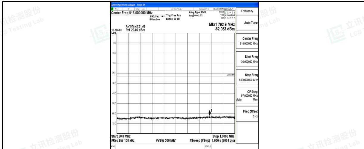
Band66_5MHz_QPSK_132647_1RB#0_30~1000_30~1000
