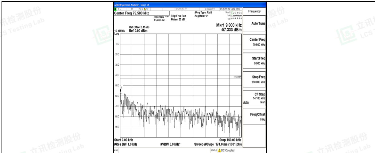
Band66_3MHz_QPSK_132322_1RB#0_0.009~0.15_0.009~0.15
