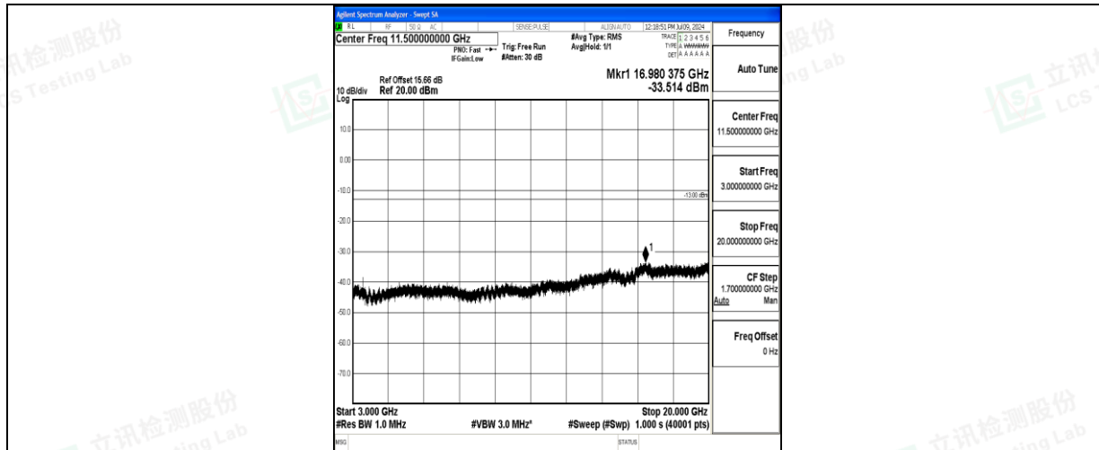
Band66_1.4MHz_16QAM_132322_1RB#0_3000~20000_3000~20000
