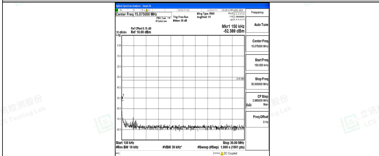
Band66_5MHz_16QAM_132647_1RB#0_0.15~30_0.15~30
