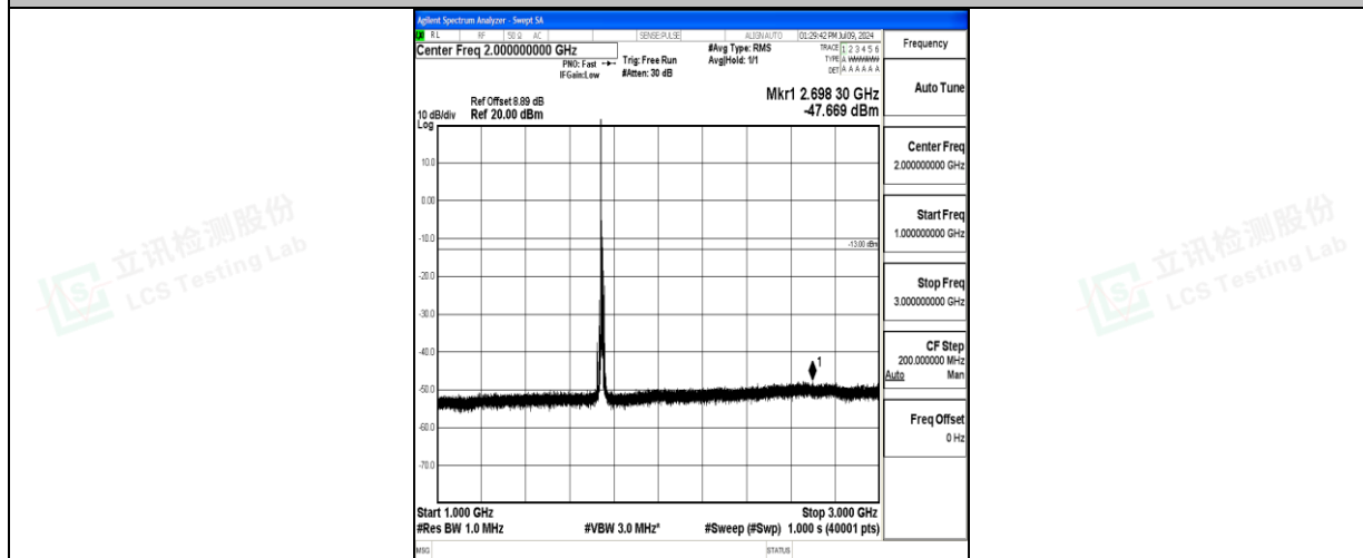
Band66_10MHz_16QAM_132322_1RB#0_1000~3000_1000~3000
