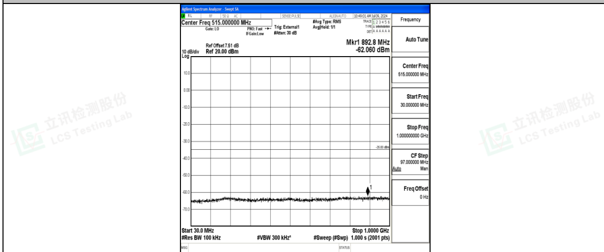
Band41_10MHz_16QAM_40620_1RB#0_30~1000_30~1000
