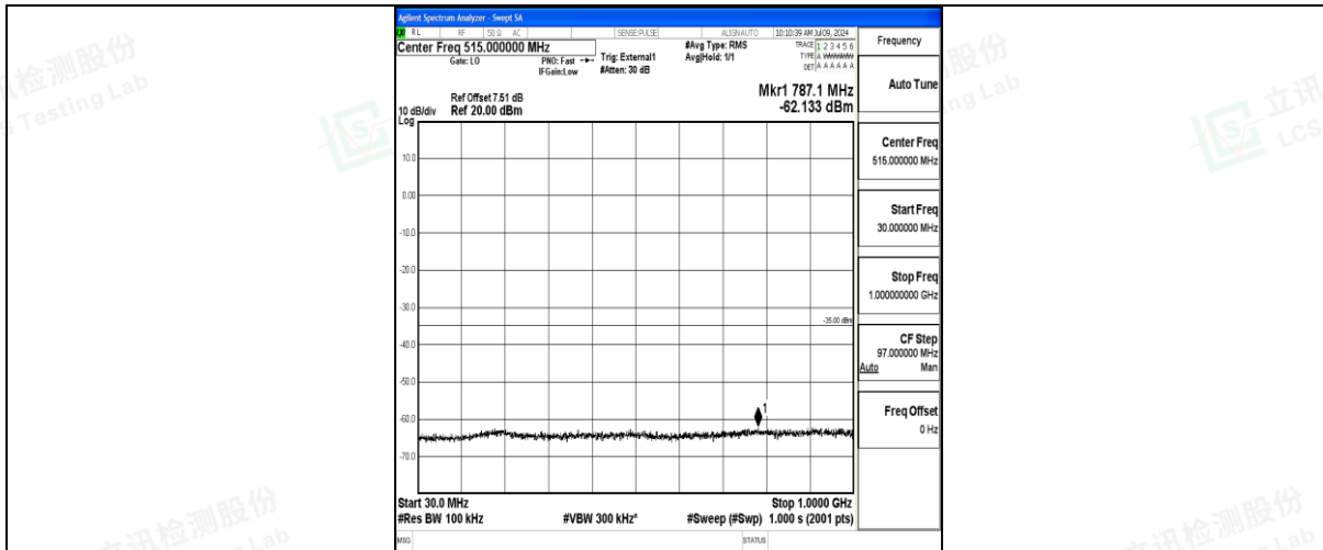
Band41_5MHz_QPSK_40620_1RB#0_30~1000_30~1000
