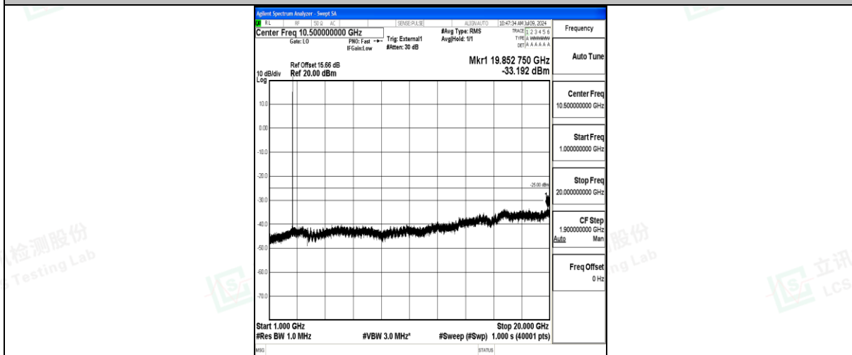
Band41_10MHz_QPSK_40620_1RB#0_1000~20000_1000~20000
