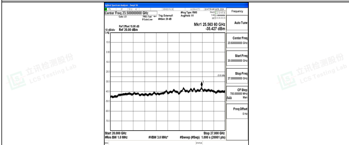
Band41_10MHz_QPSK_40620_1RB#0_20000~27000_20000~27000
