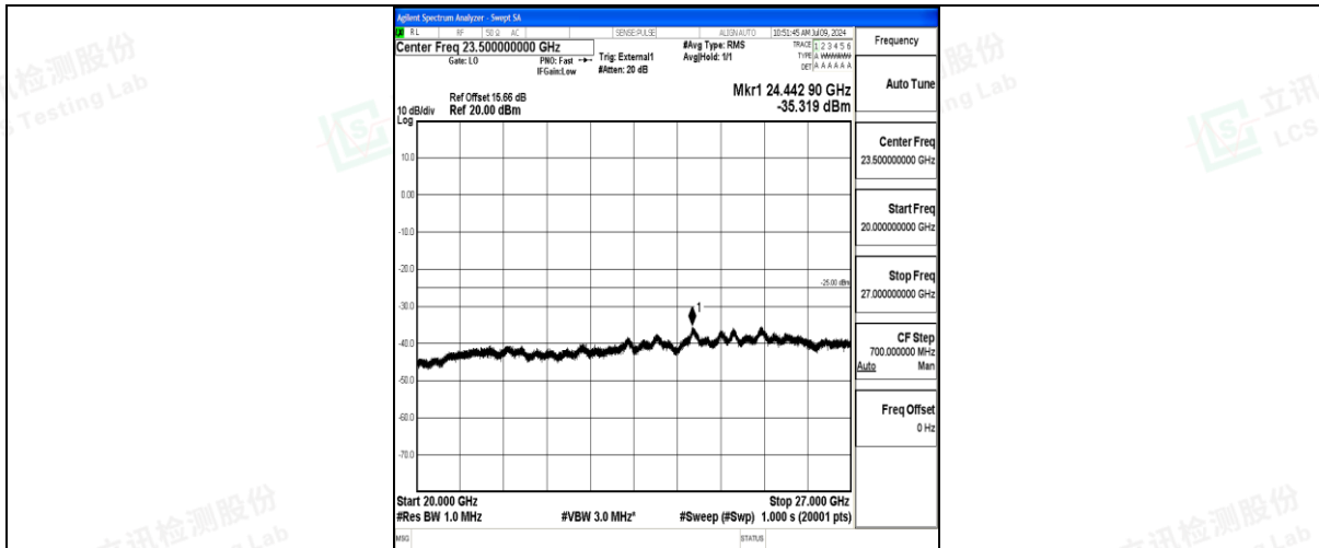
Band41_10MHz_QPSK_41540_1RB#0_20000~27000_20000~27000
