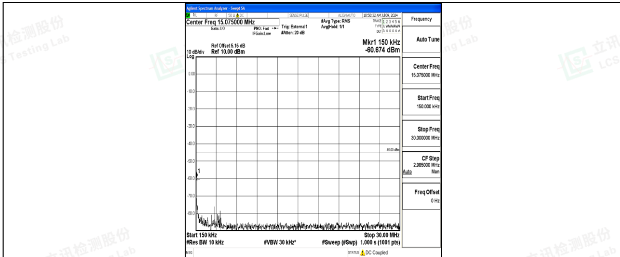
Band41_10MHz_QPSK_41540_1RB#0_0.15~30_0.15~30
