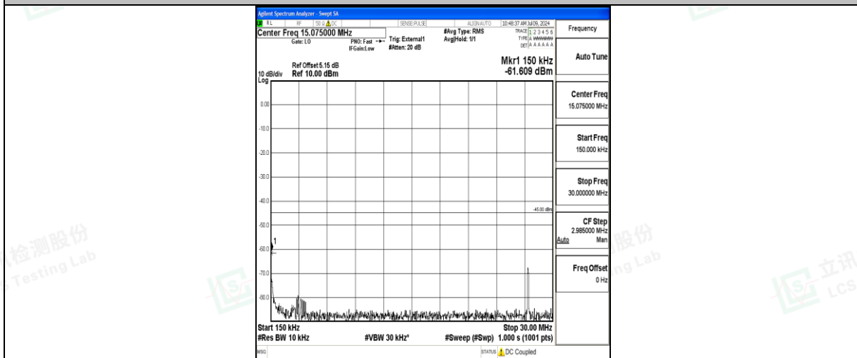
Band41_10MHz_16QAM_40620_1RB#0_0.15~30_0.15~30
