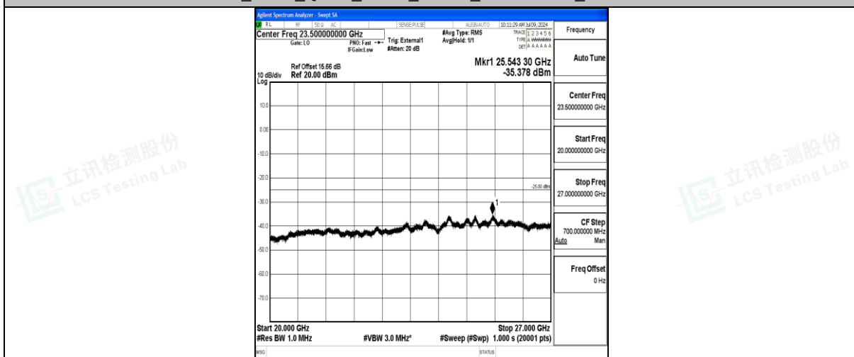
Band41_5MHz_QPSK_40620_1RB#0_20000~27000_20000~27000
