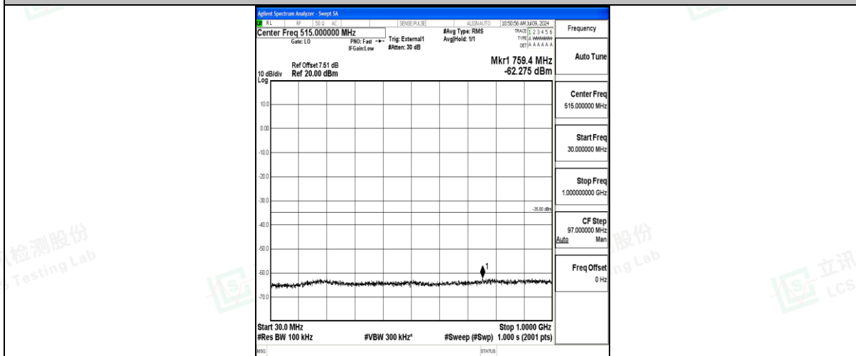
Band41_10MHz_QPSK_41540_1RB#0_30~1000_30~1000
