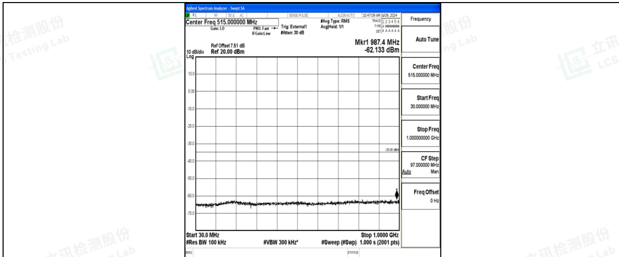
Band41_10MHz_QPSK_40620_1RB#0_30~1000_30~1000
