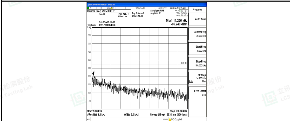
Band41_5MHz_16QAM_41565_1RB#0_0.009~0.15_0.009~0.15
