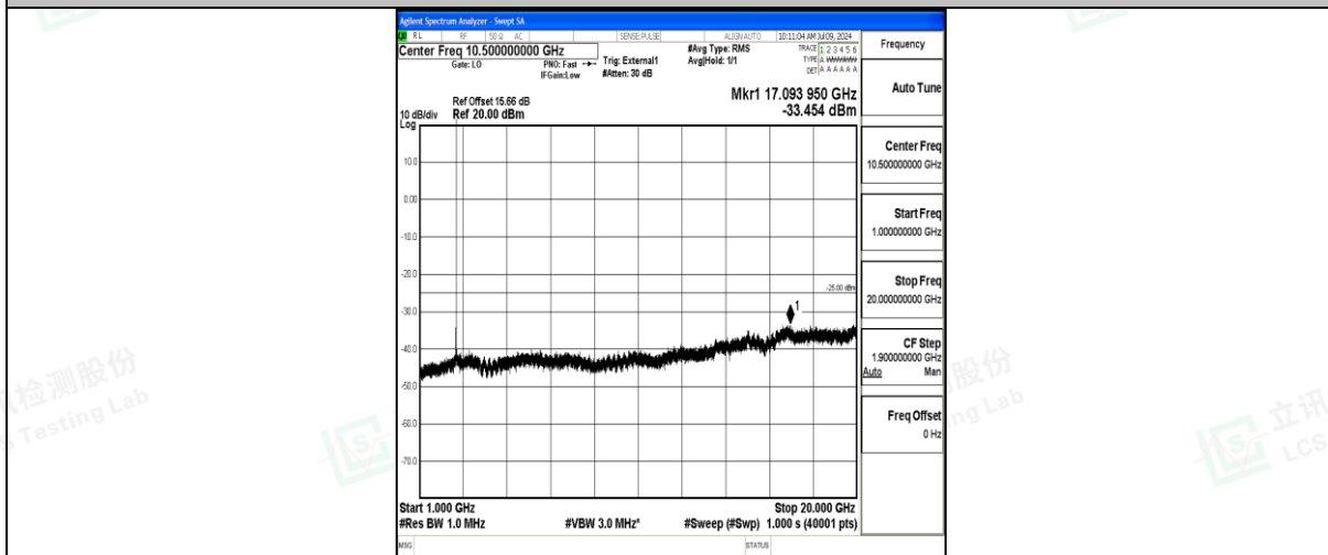
Band41_5MHz_QPSK_40620_1RB#0_1000~20000_1000~20000
