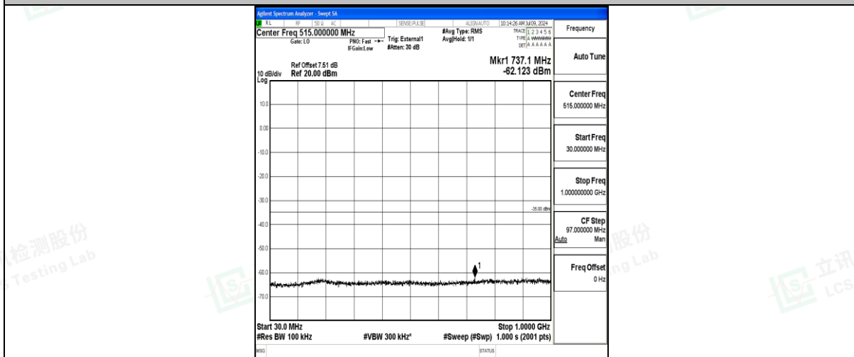
Band41_5MHz_QPSK_41565_1RB#0_30~1000_30~1000
