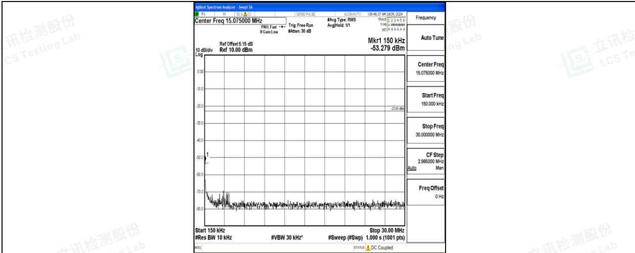
Band26_15MHz_QPSK_26965_1RB#0_0.15~30_0.15~30
