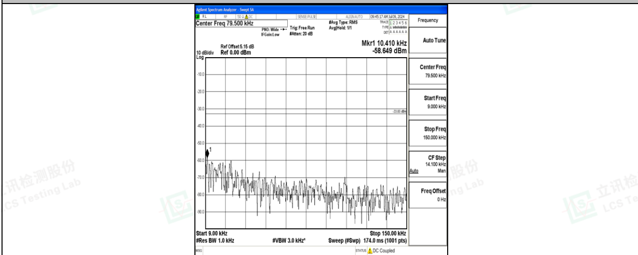
Band26_15MHz_QPSK_26915_1RB#0_0.009~0.15_0.009~0.15
