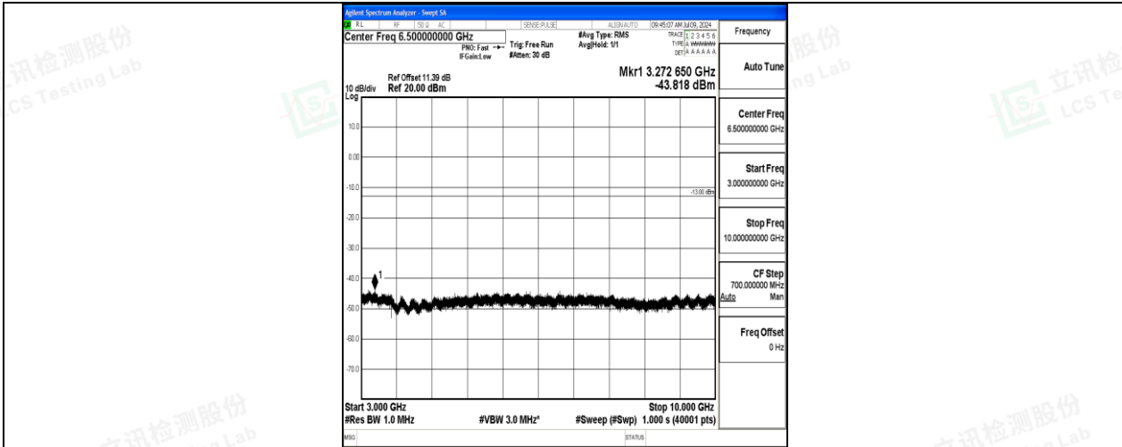
Band26_15MHz_16QAM_26865_1RB#0_3000~10000_3000~10000
