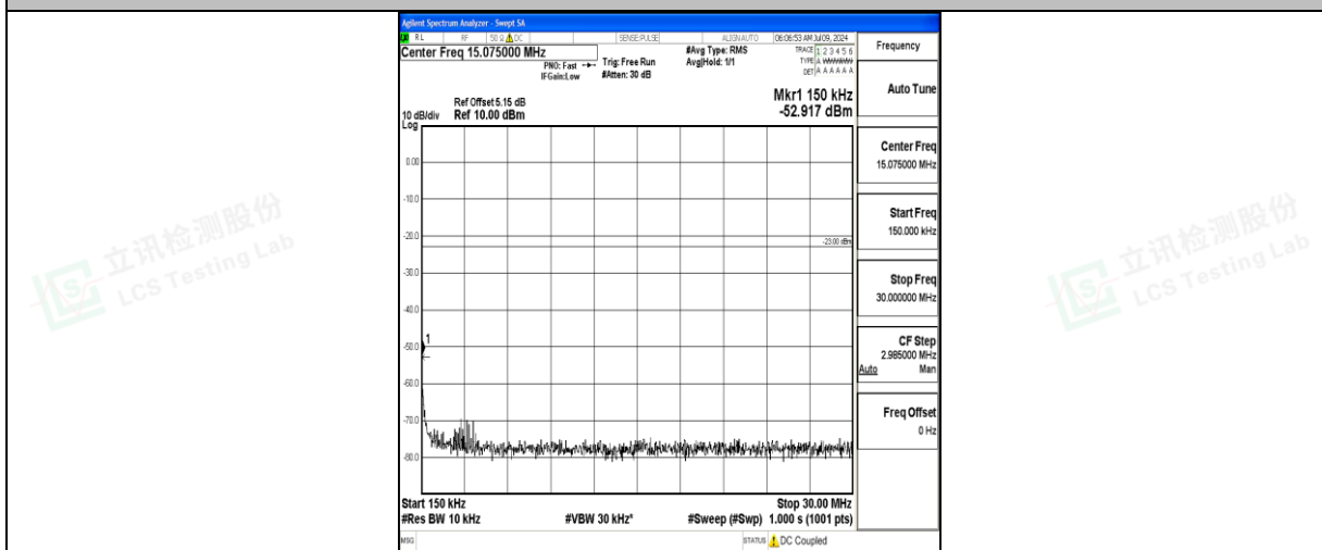
Band26_10MHz_16QAM_26740_1RB#0_0.15~30_0.15~30
