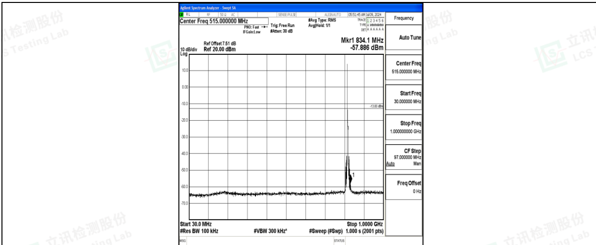
Band26_5MHz_QPSK_26765_1RB#0_30~1000_30~1000
