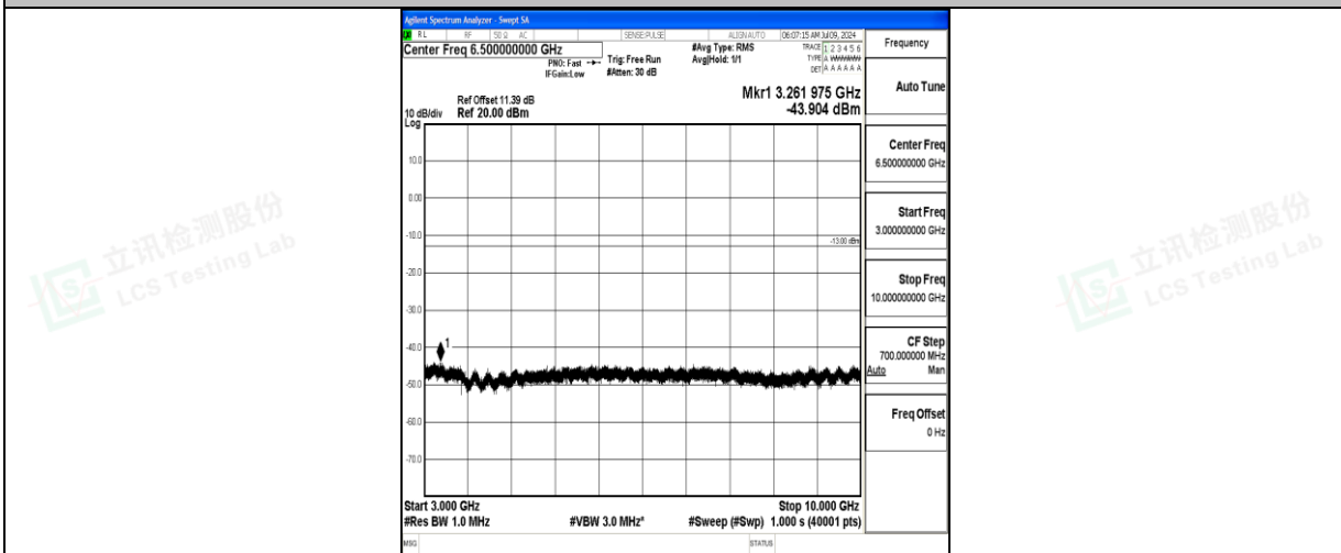
Band26_10MHz_16QAM_26740_1RB#0_3000~10000_3000~10000
