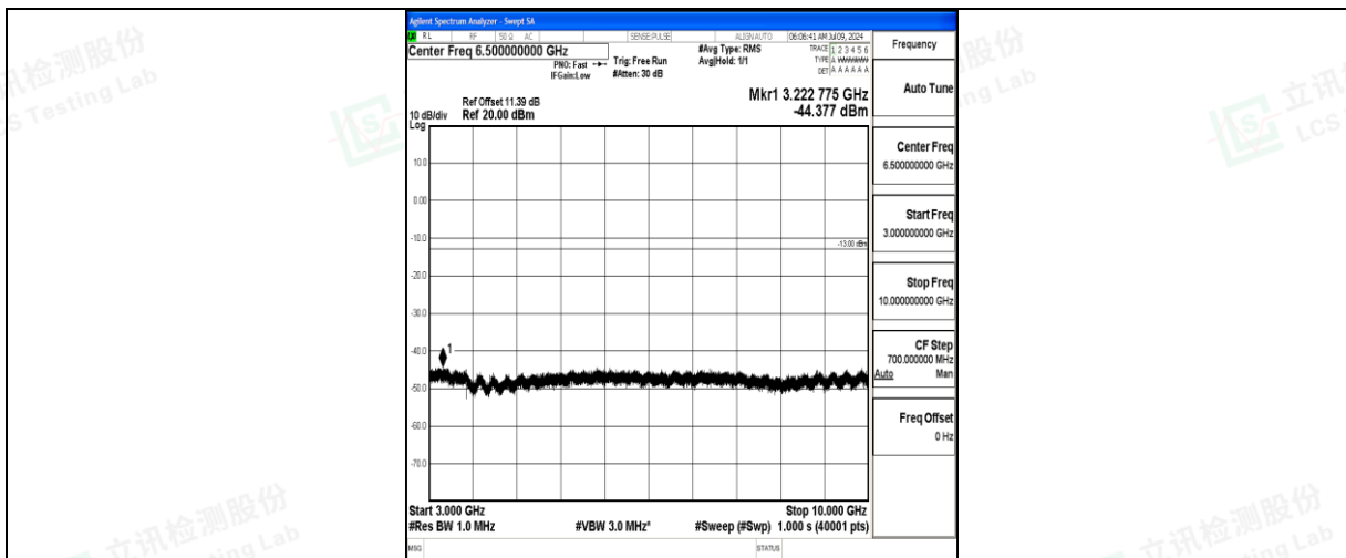
Band26_10MHz_QPSK_26740_1RB#0_3000~10000_3000~10000
