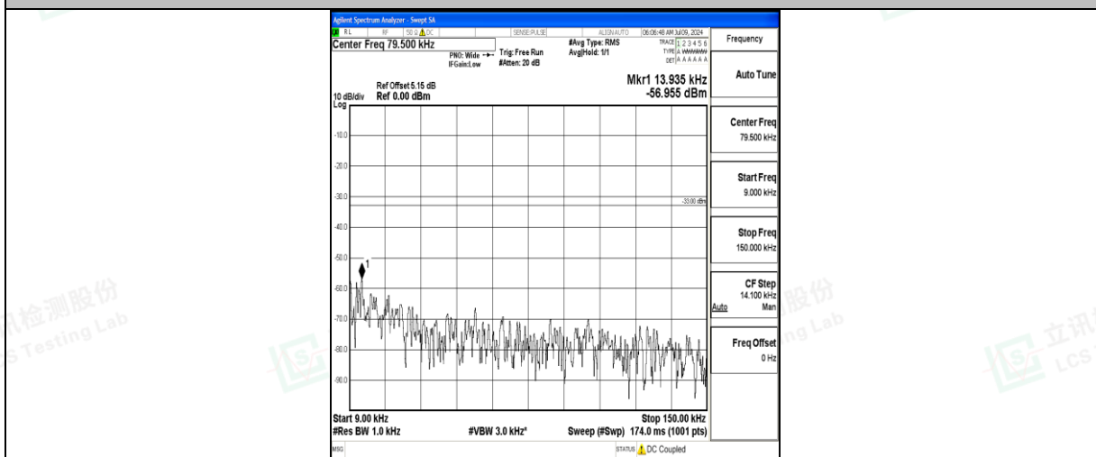
Band26_10MHz_16QAM_26740_1RB#0_0.009~0.15_0.009~0.15
